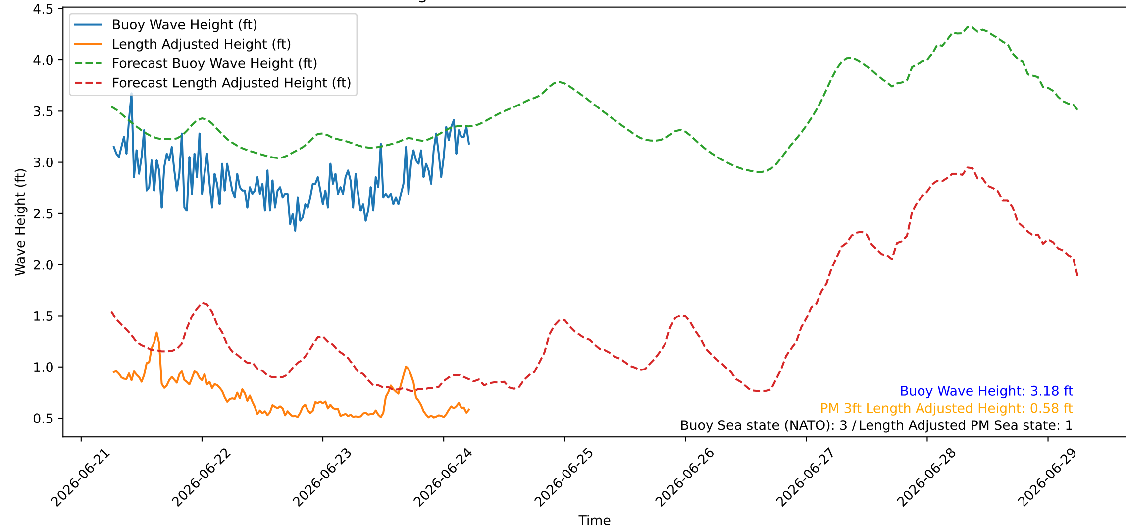
Wave Heights over Time for Red Beach at 2026-06-24 06:00:44
