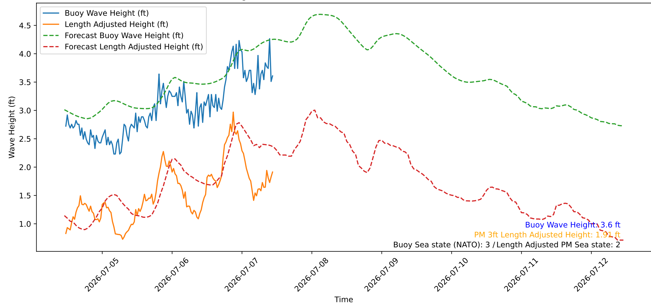
Wave Heights over Time for Red Beach at 2026-07-07 11:10:46
