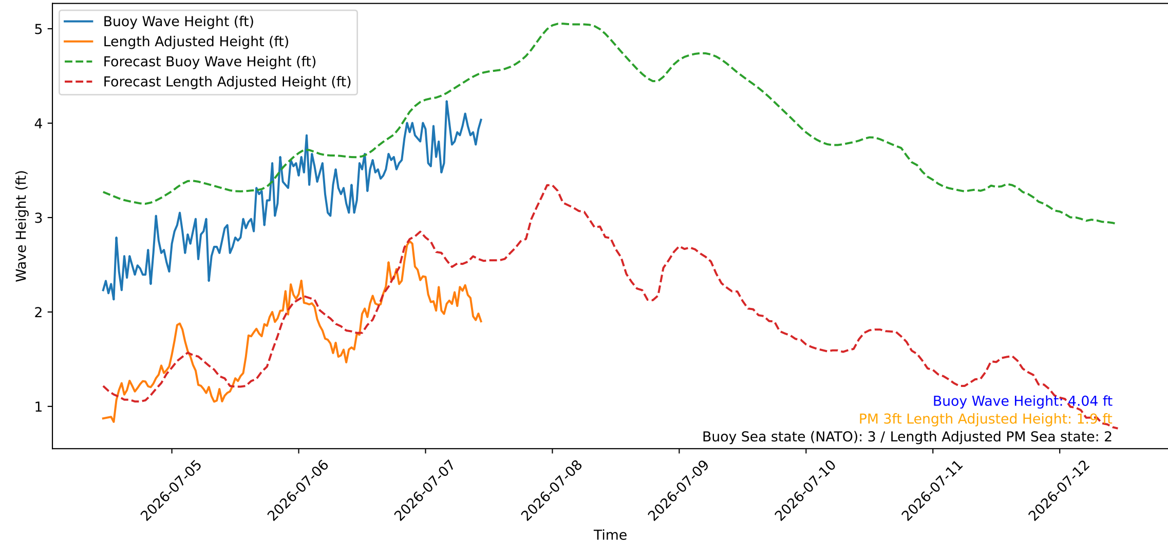
Wave Heights over Time for Oceanside Harbor at 2026-07-07 11:10:27
