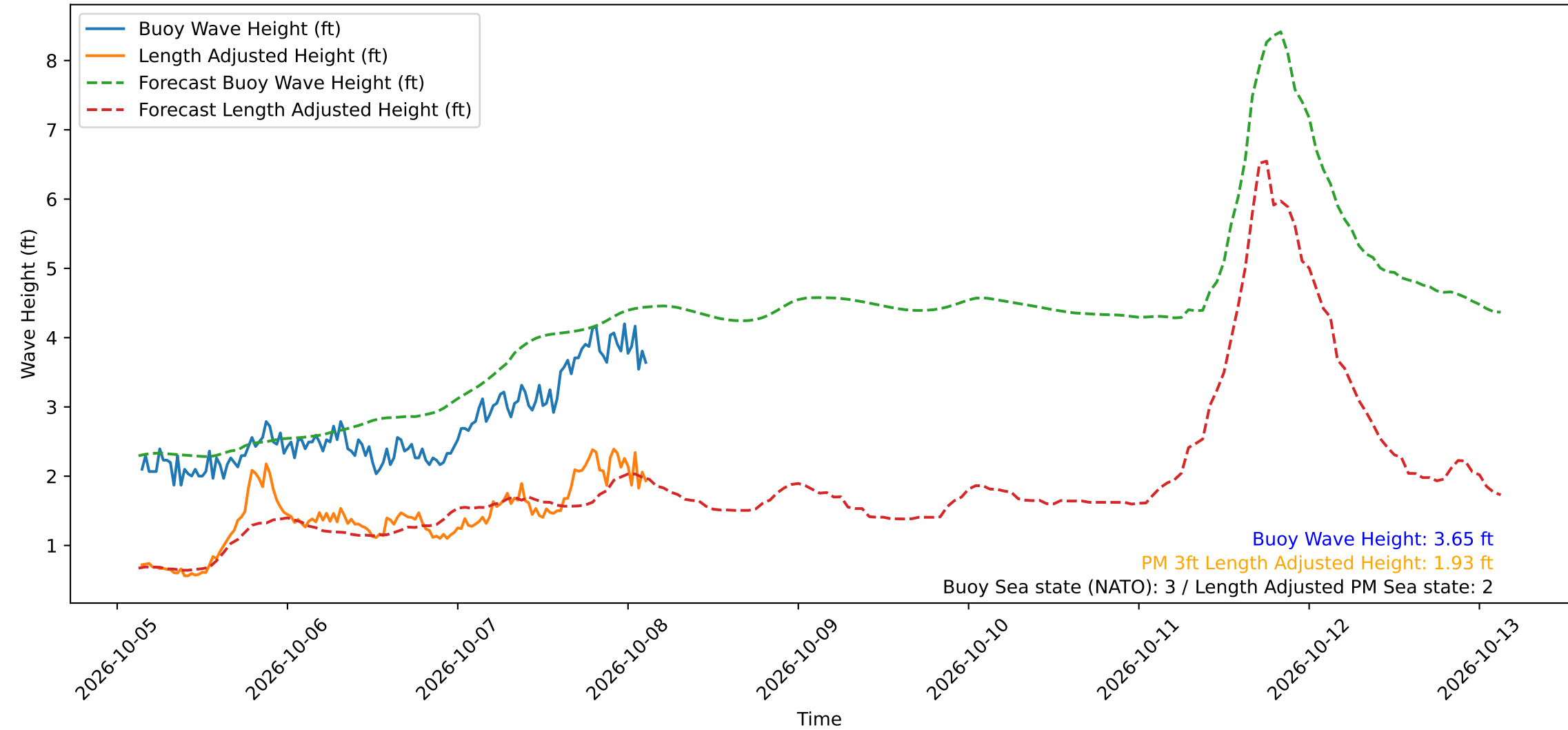
Wave Heights over Time for Oceanside Harbor at 2026-10-08 03:20:29
