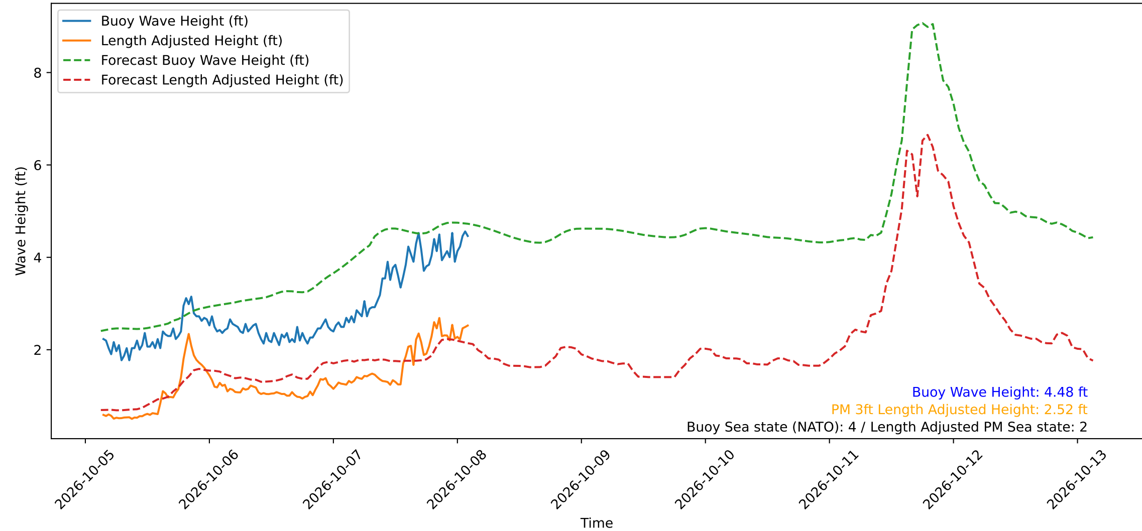
Wave Heights over Time for Green Beach at 2026-10-08 03:21:14
