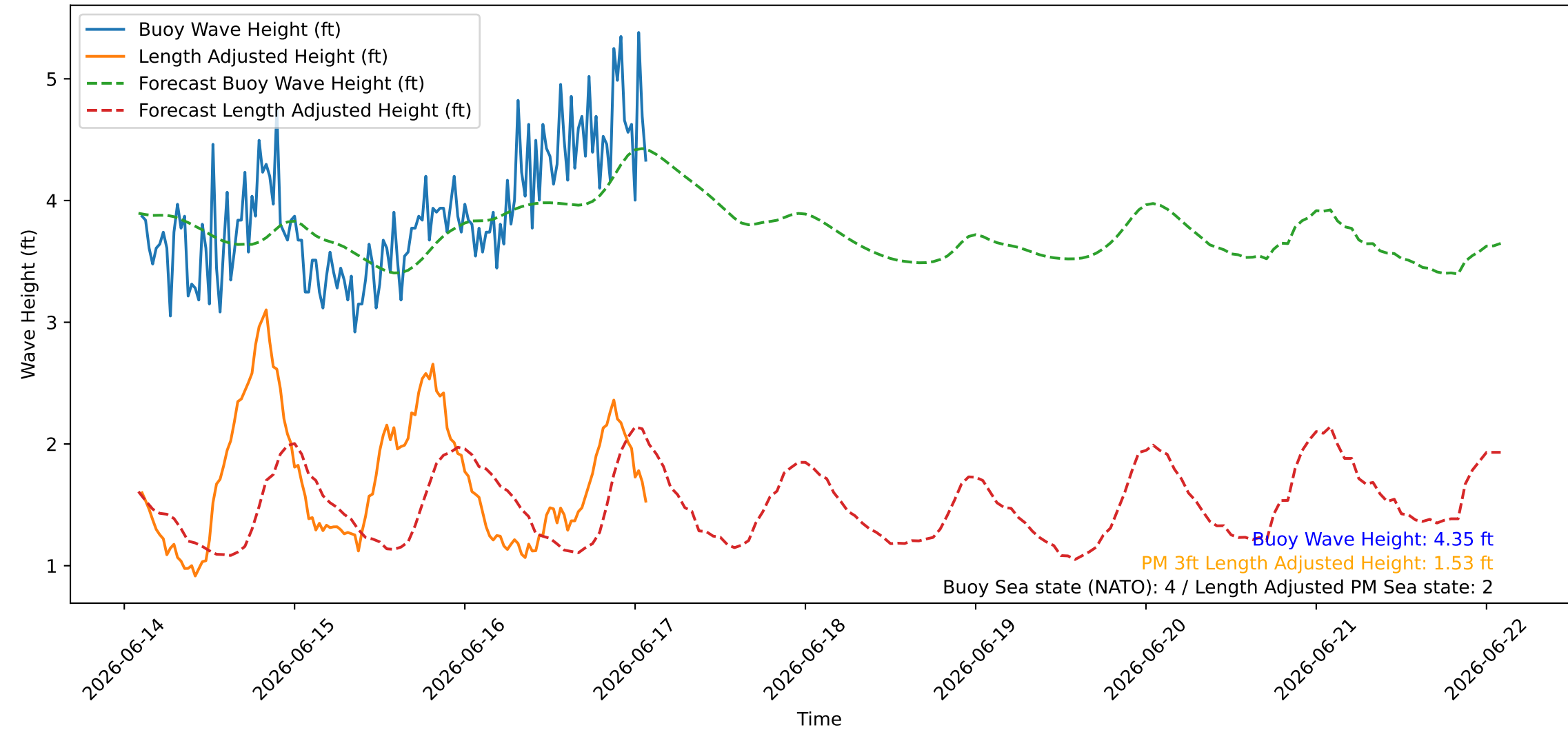
Wave Heights over Time for Red Beach at 2026-06-17 02:20:46
