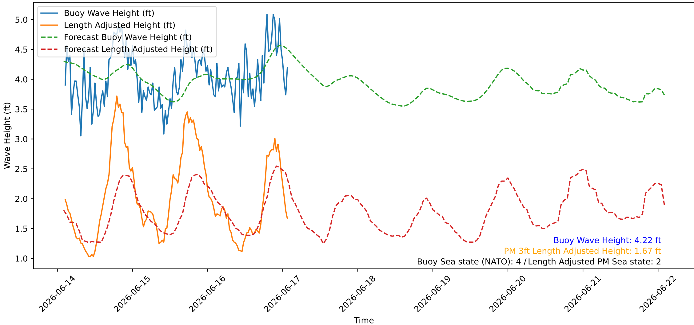
Wave Heights over Time for Green Beach at 2026-06-17 02:21:08
