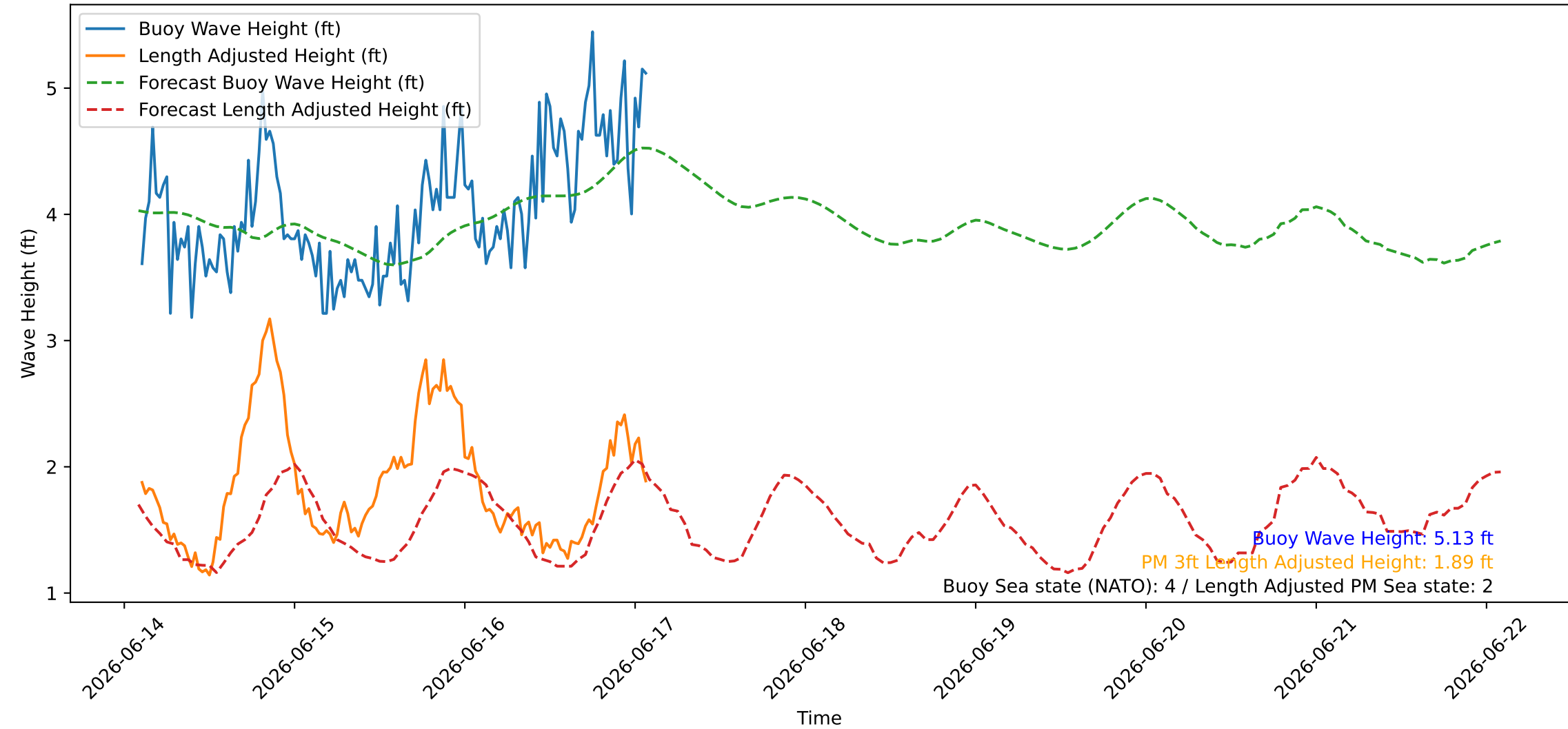
Wave Heights over Time for Oceanside Harbor at 2026-06-17 02:20:26
