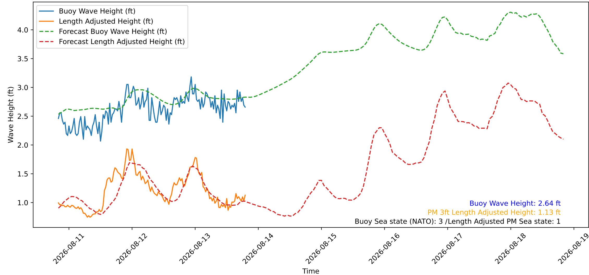
Wave Heights over Time for Oceanside Harbor at 2026-08-13 19:50:26
