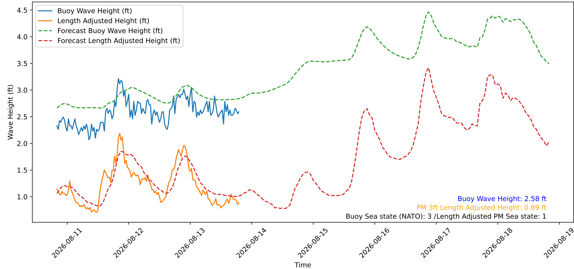
Wave Heights over Time for Green Beach at 2026-08-13 19:51:10
