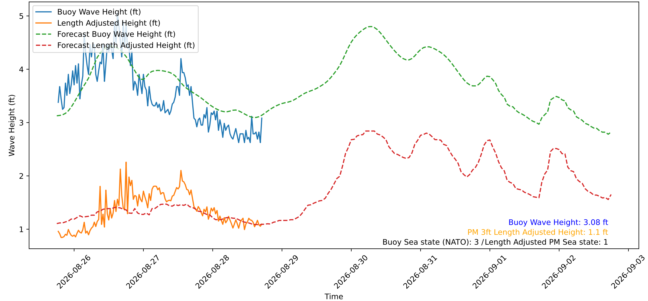
Wave Heights over Time for Red Beach at 2026-08-28 18:00:50
