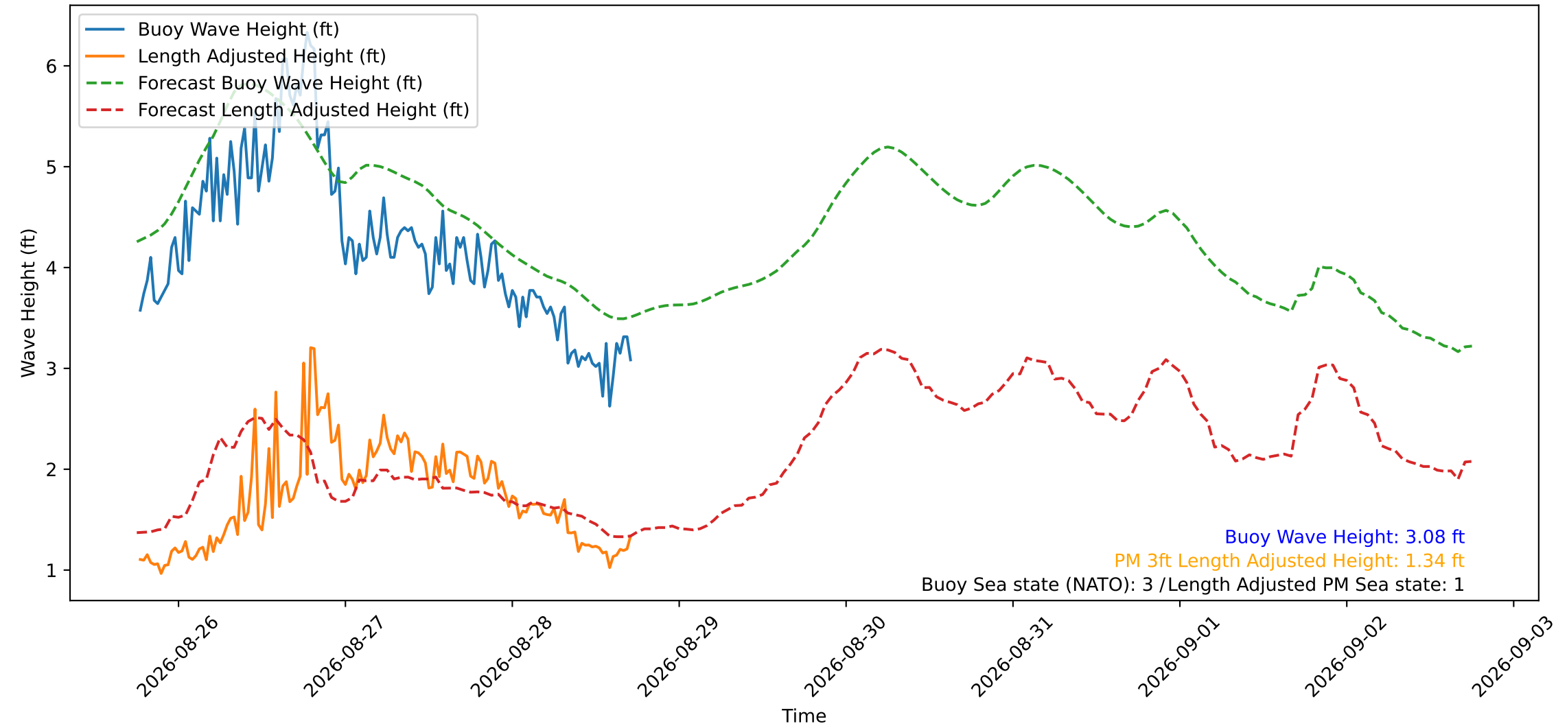
Wave Heights over Time for Green Beach at 2026-08-28 18:01:12
