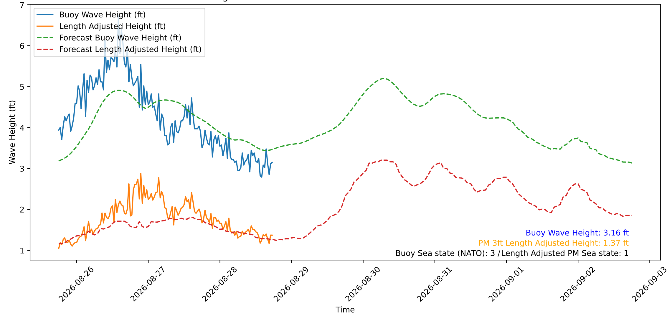
Wave Heights over Time for Oceanside Harbor at 2026-08-28 18:00:30
