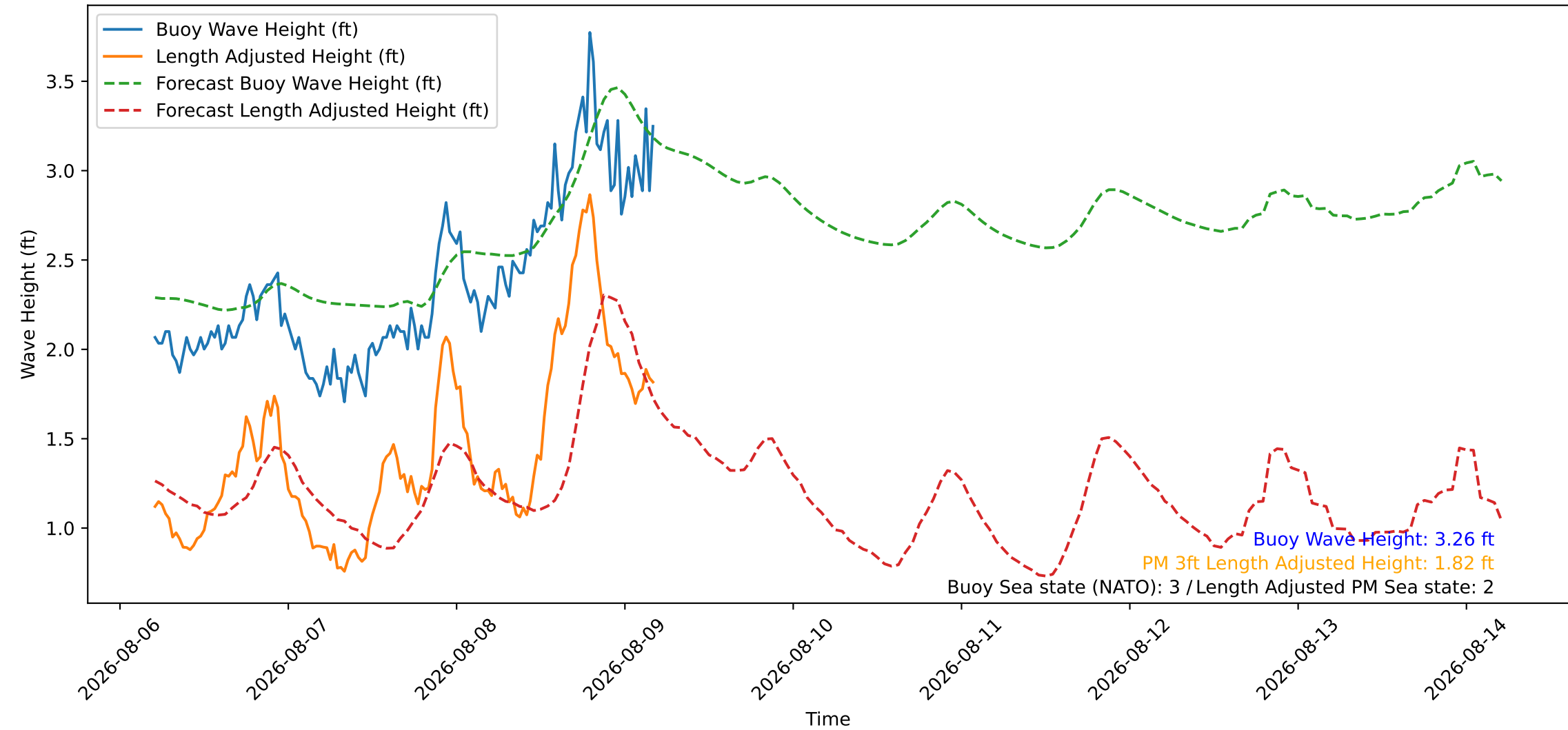
Wave Heights over Time for Green Beach at 2026-08-09 04:51:11
