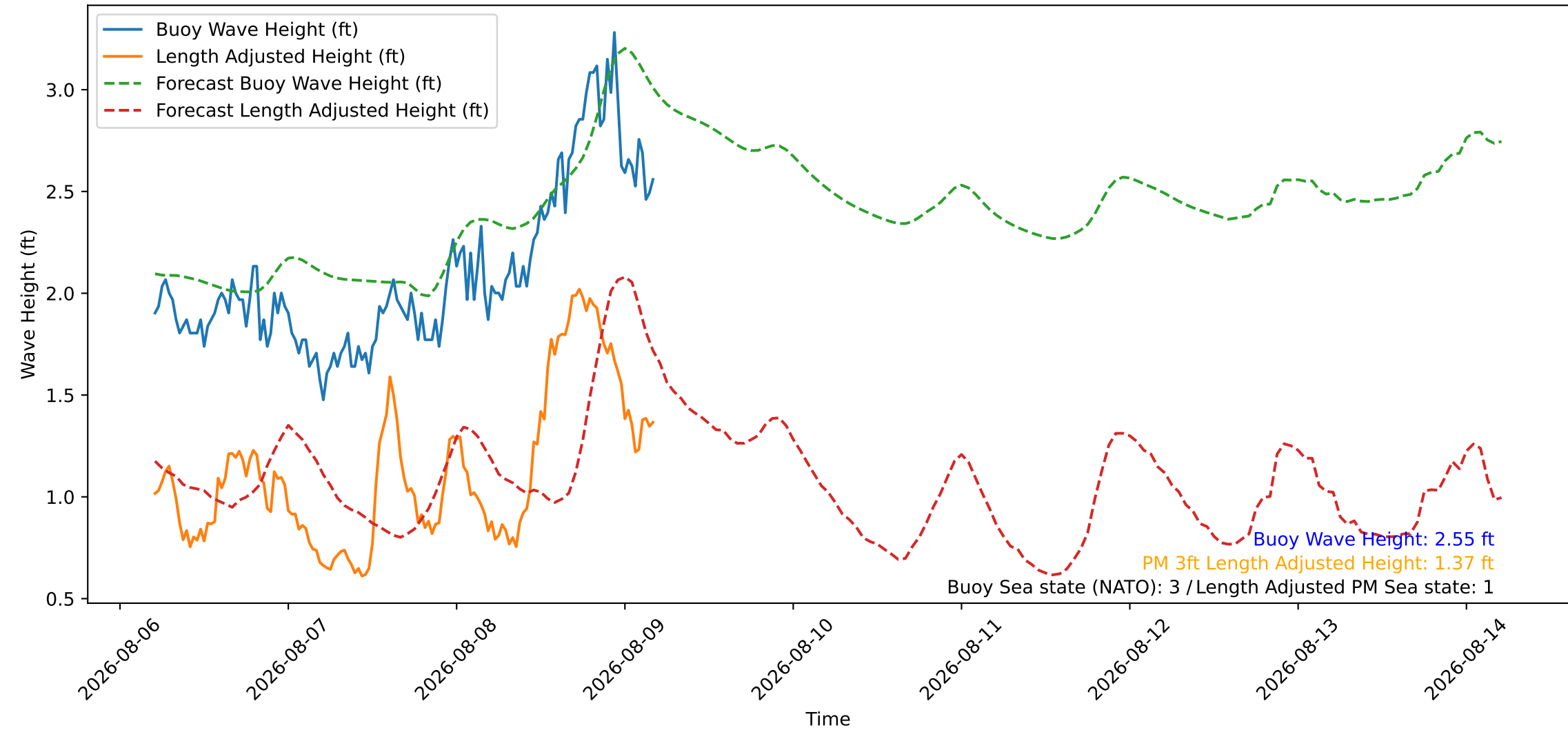
Wave Heights over Time for Red Beach at 2026-08-09 04:50:49
