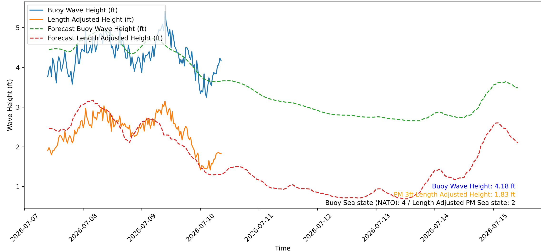
Wave Heights over Time for Oceanside Harbor at 2026-07-10 09:30:26
