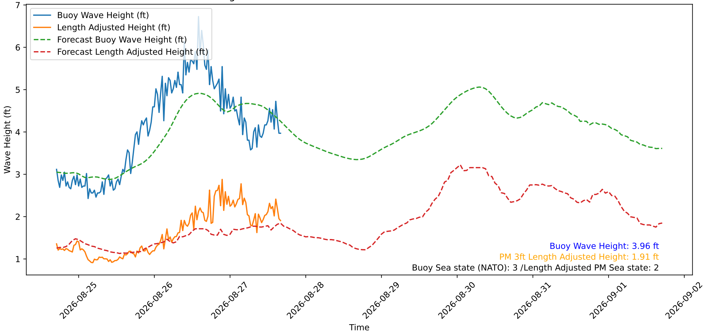
Wave Heights over Time for Oceanside Harbor at 2026-08-27 16:50:29
