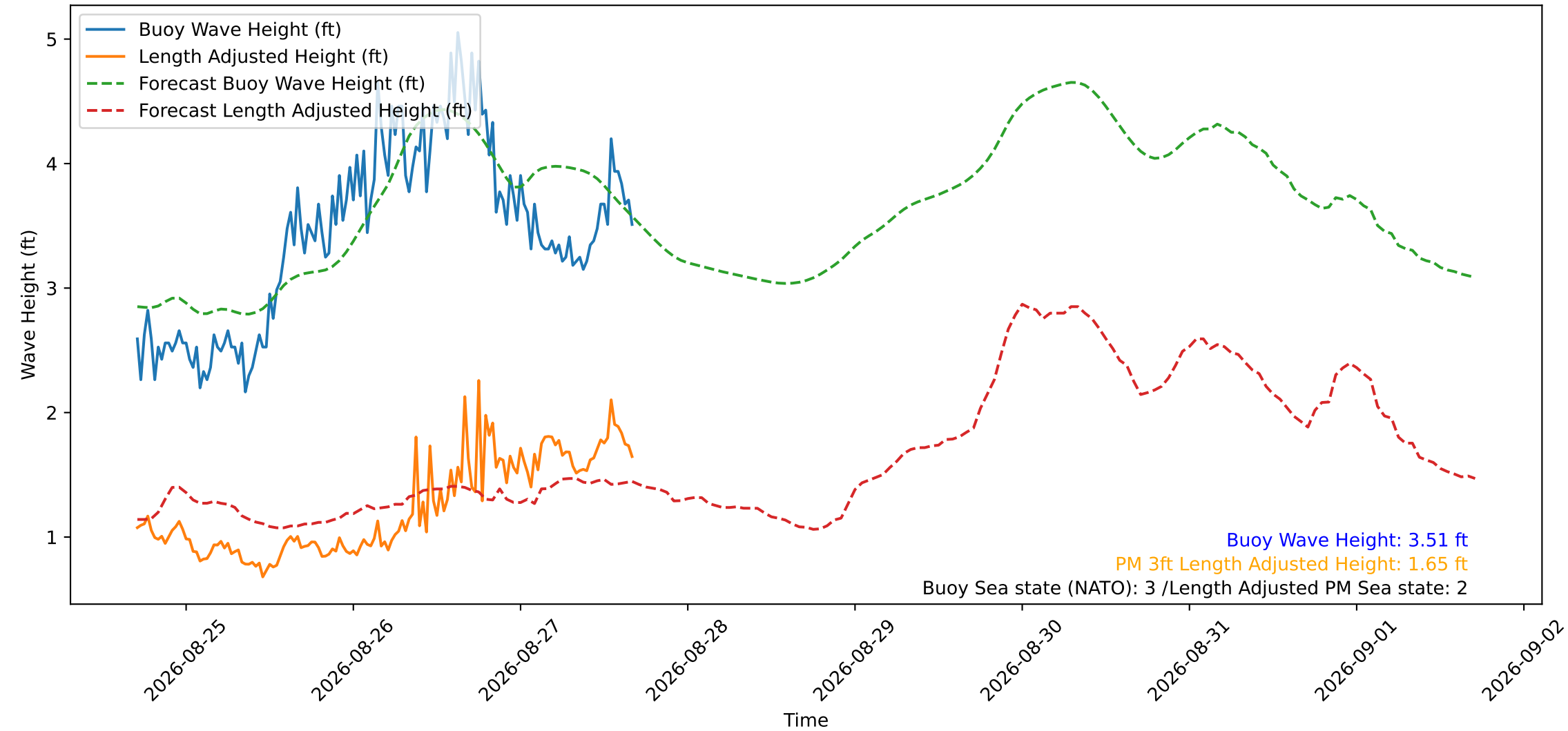
Wave Heights over Time for Red Beach at 2026-08-27 16:50:51
