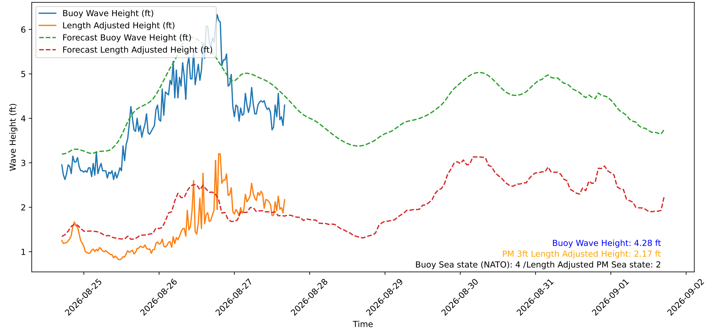
Wave Heights over Time for Green Beach at 2026-08-27 16:51:15
