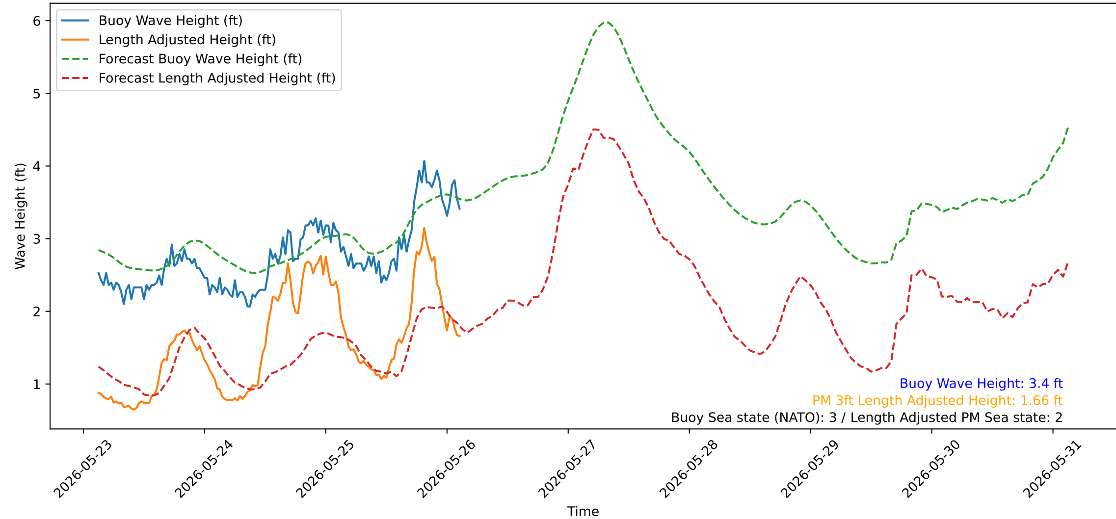
Wave Heights over Time for Green Beach at 2026-05-26 03:11:11
