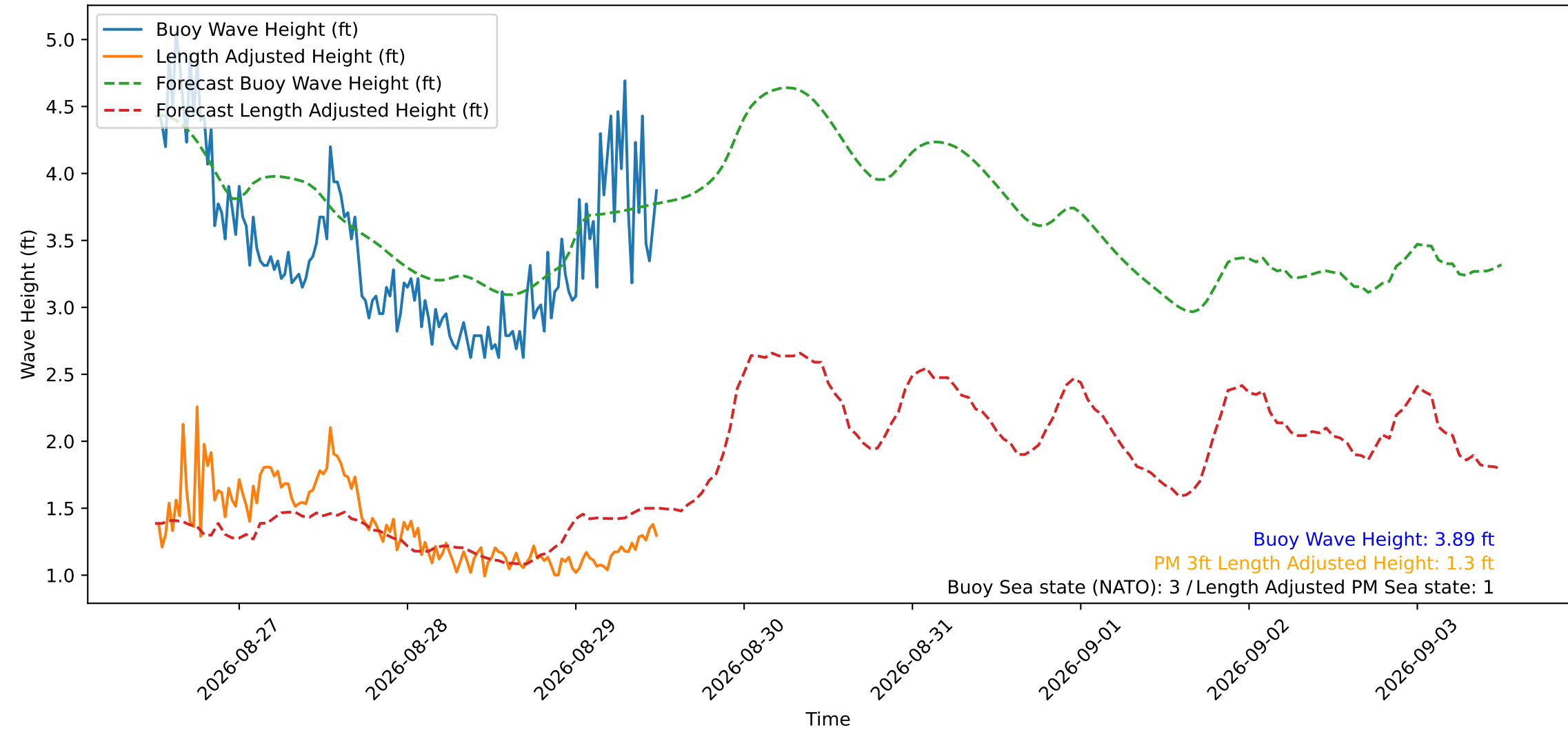
Wave Heights over Time for Red Beach at 2026-08-29 12:10:49
