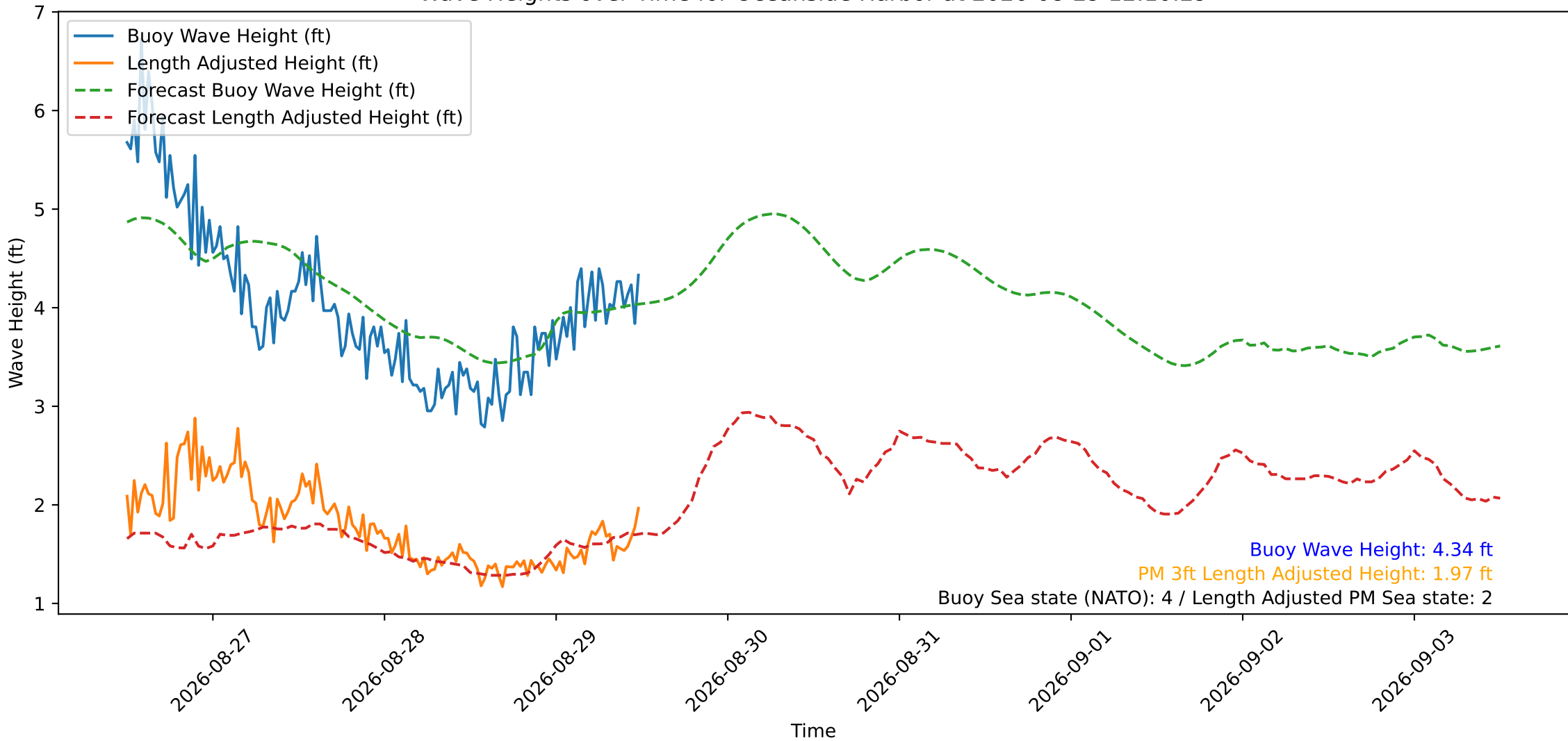
Wave Heights over Time for Oceanside Harbor at 2026-08-29 12:10:29
