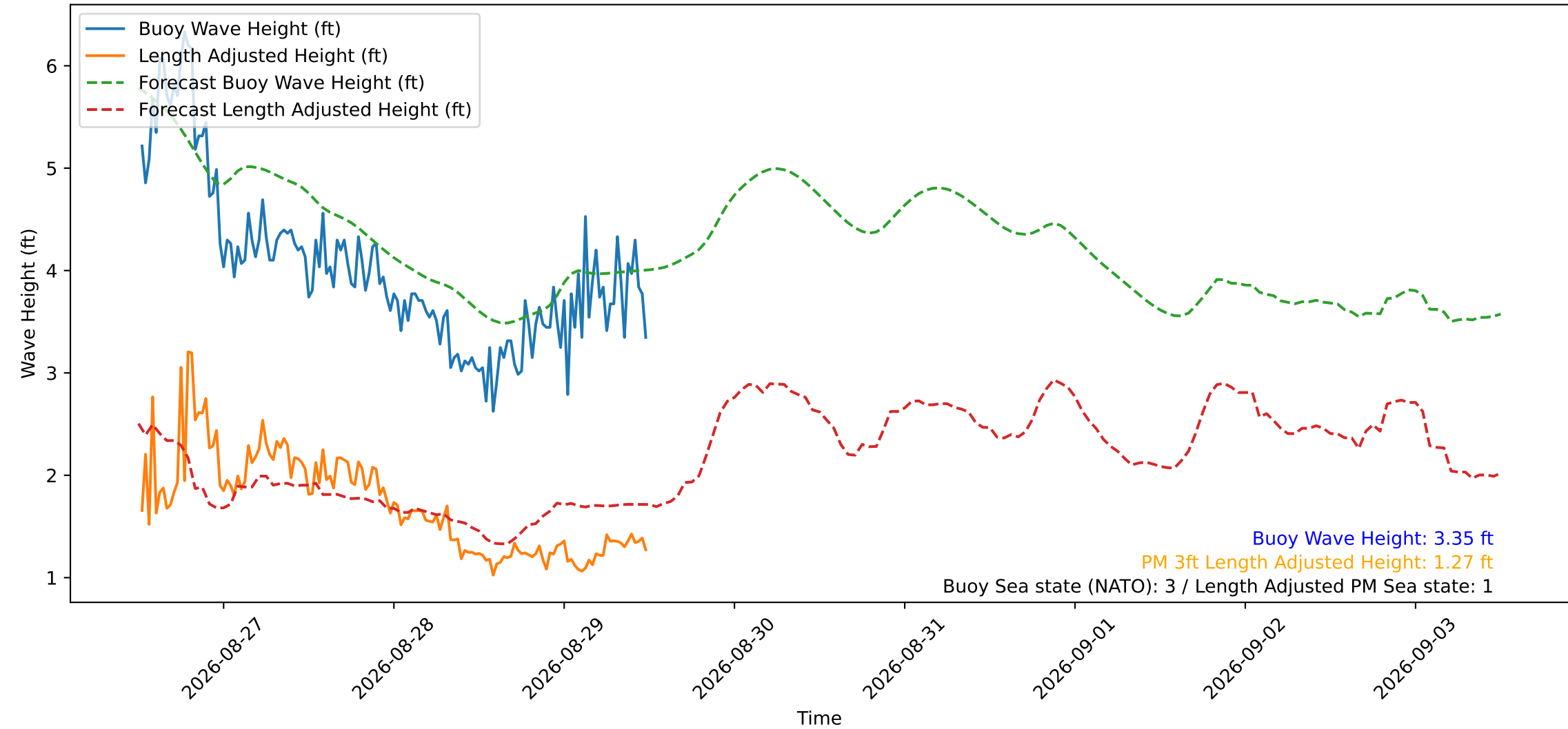
Wave Heights over Time for Green Beach at 2026-08-29 12:11:11
