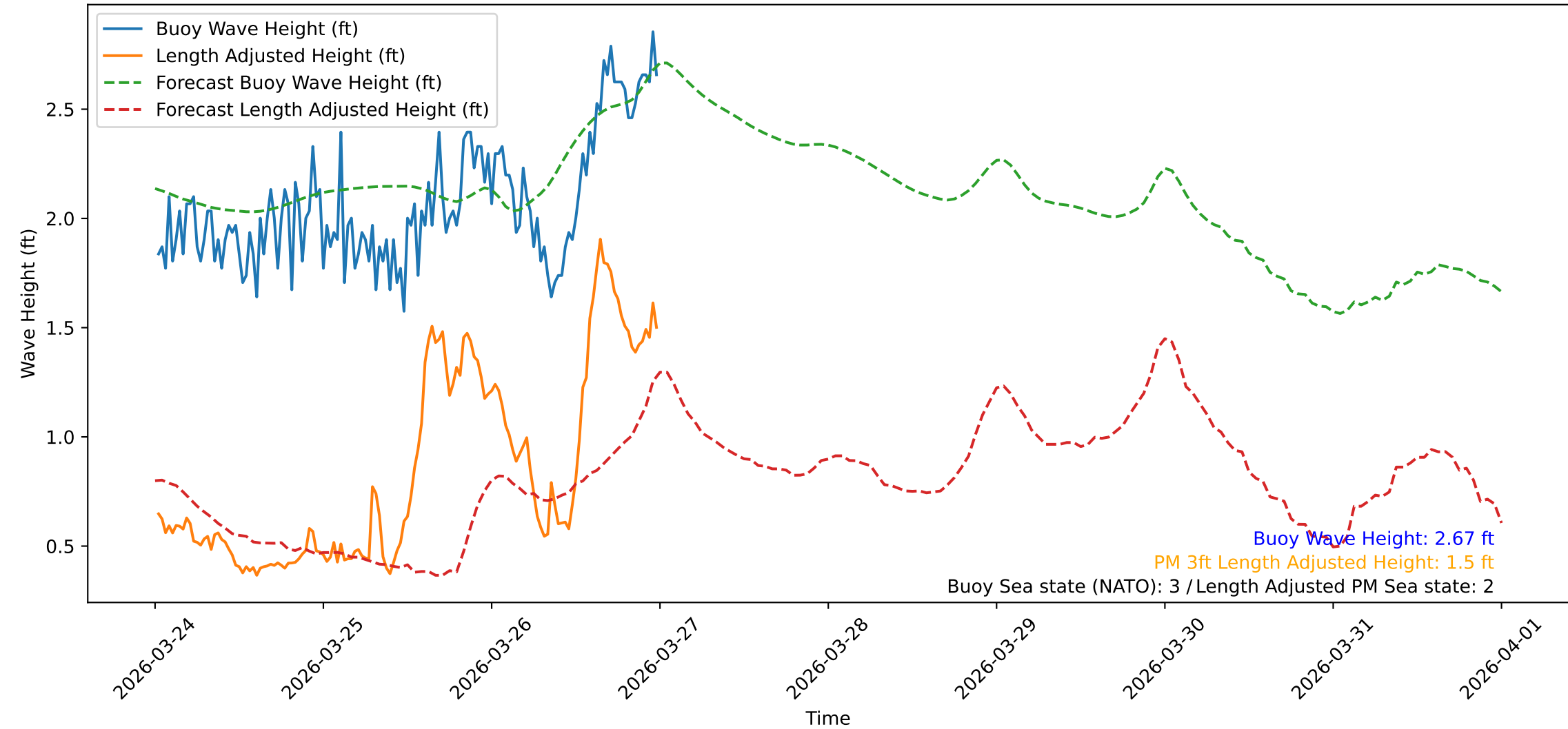
Wave Heights over Time for Red Beach at 2026-03-27 00:10:47
