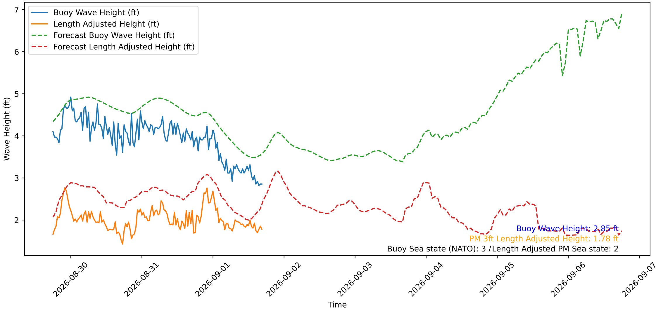
Wave Heights over Time for Green Beach at 2026-09-01 17:31:13
