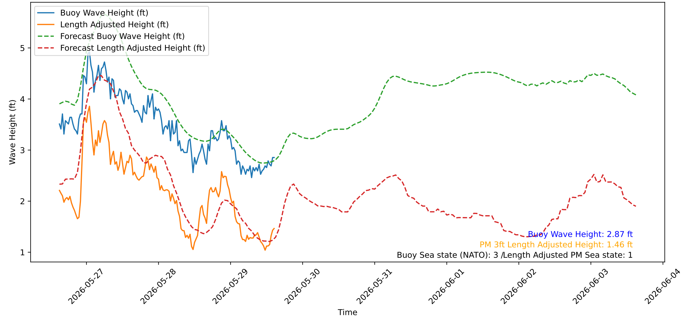
Wave Heights over Time for Green Beach at 2026-05-29 15:11:04
