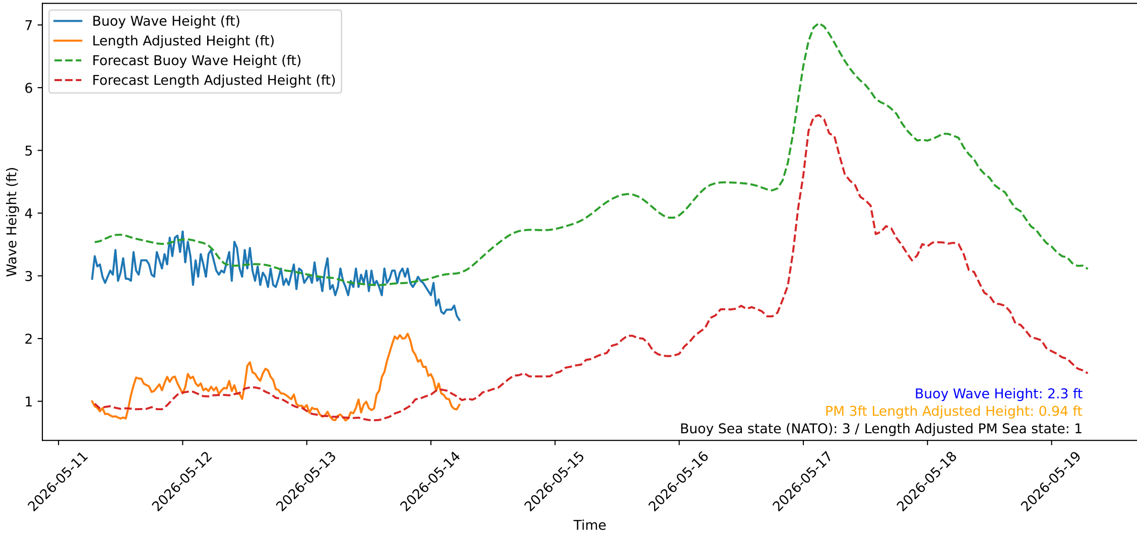
Wave Heights over Time for Oceanside Harbor at 2026-05-14 06:30:31
