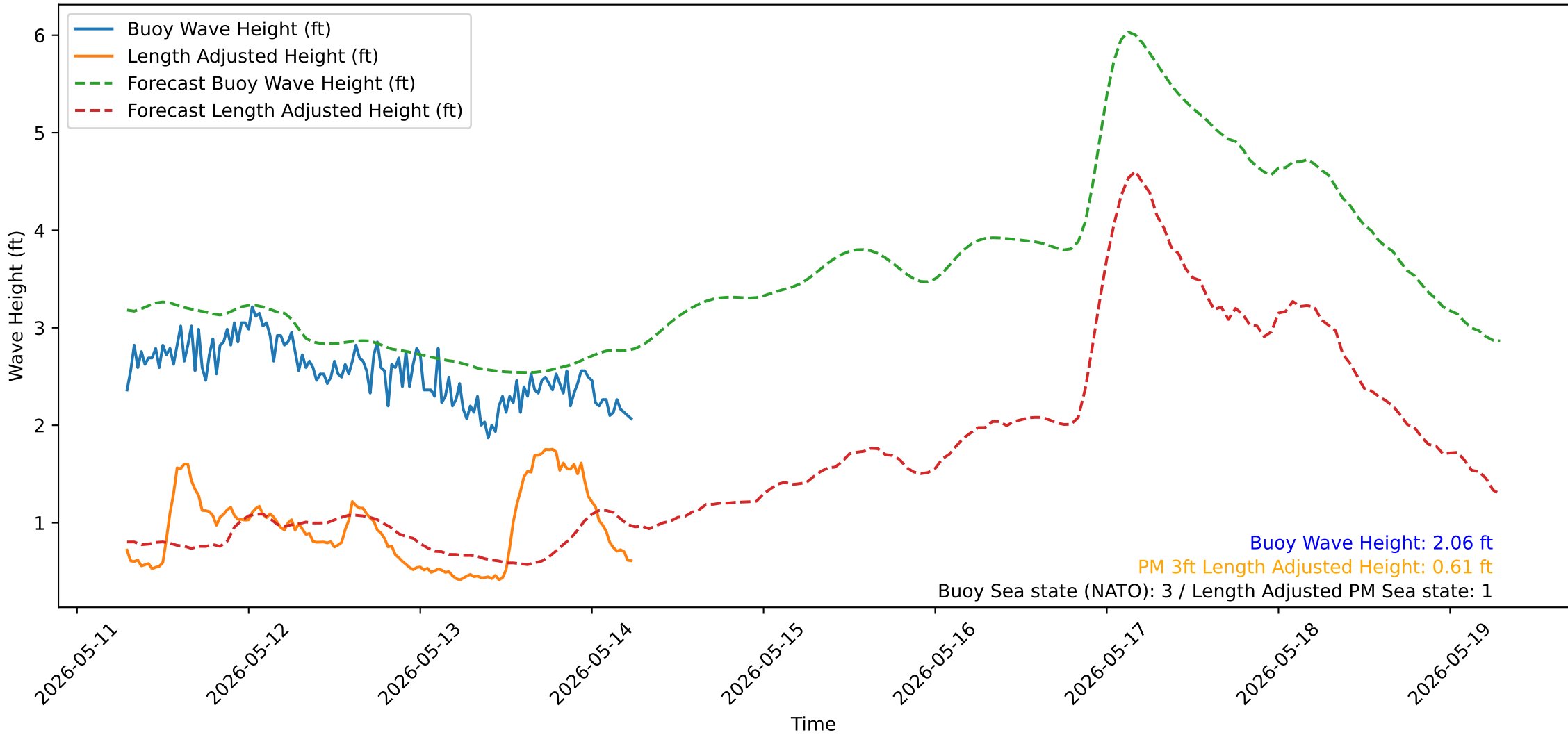
Wave Heights over Time for Red Beach at 2026-05-14 06:30:51
