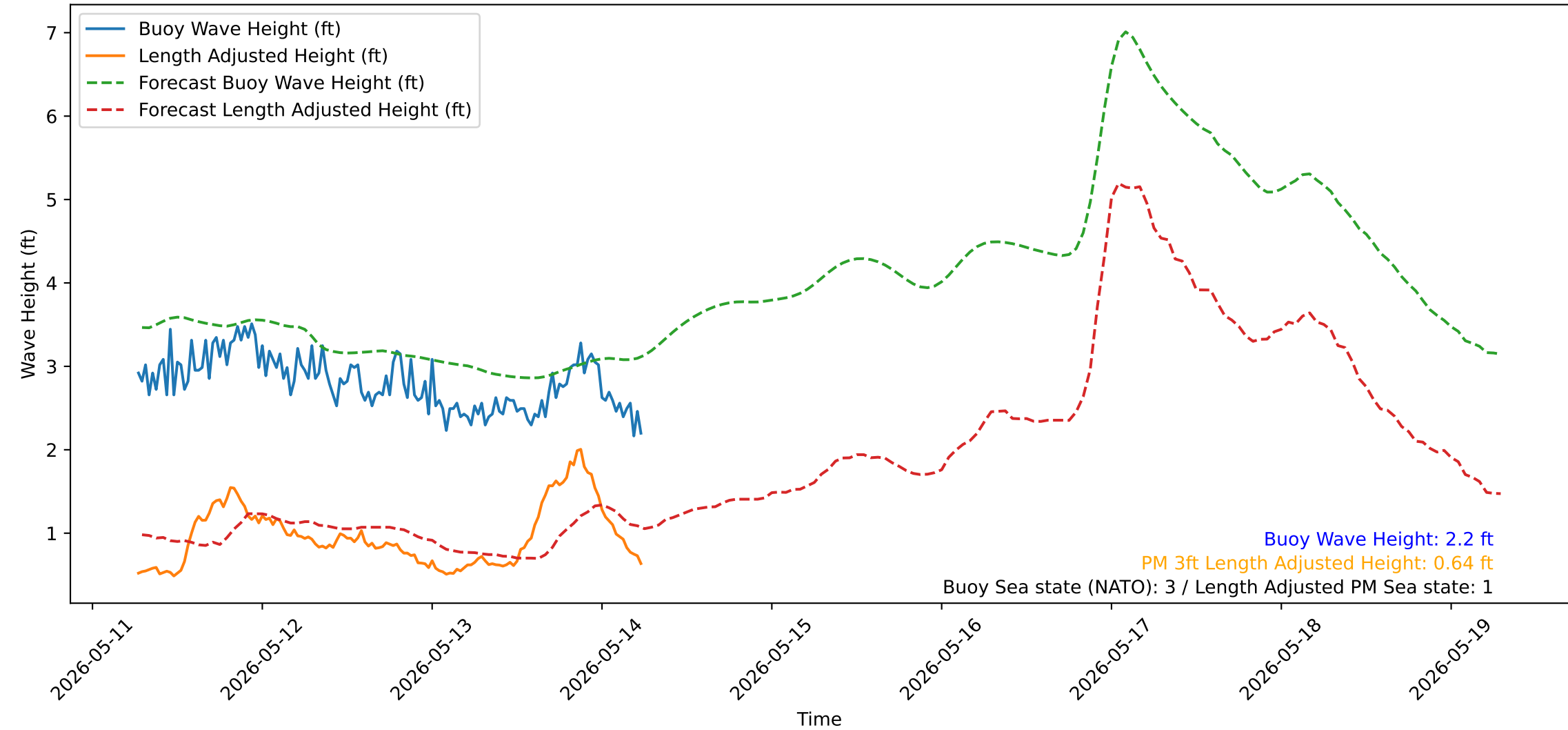
Wave Heights over Time for Green Beach at 2026-05-14 06:31:13
