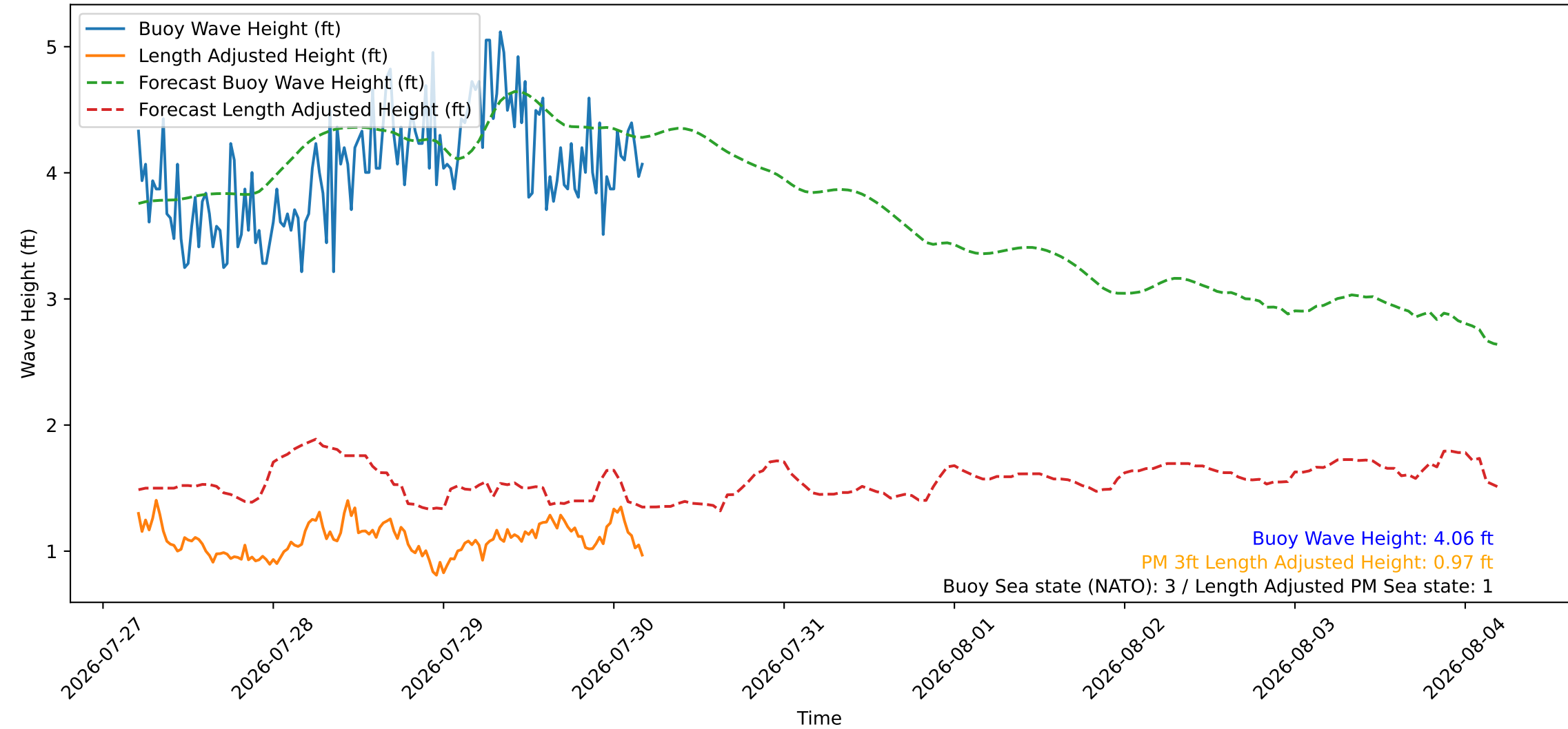
Wave Heights over Time for Red Beach at 2026-07-30 04:40:46
