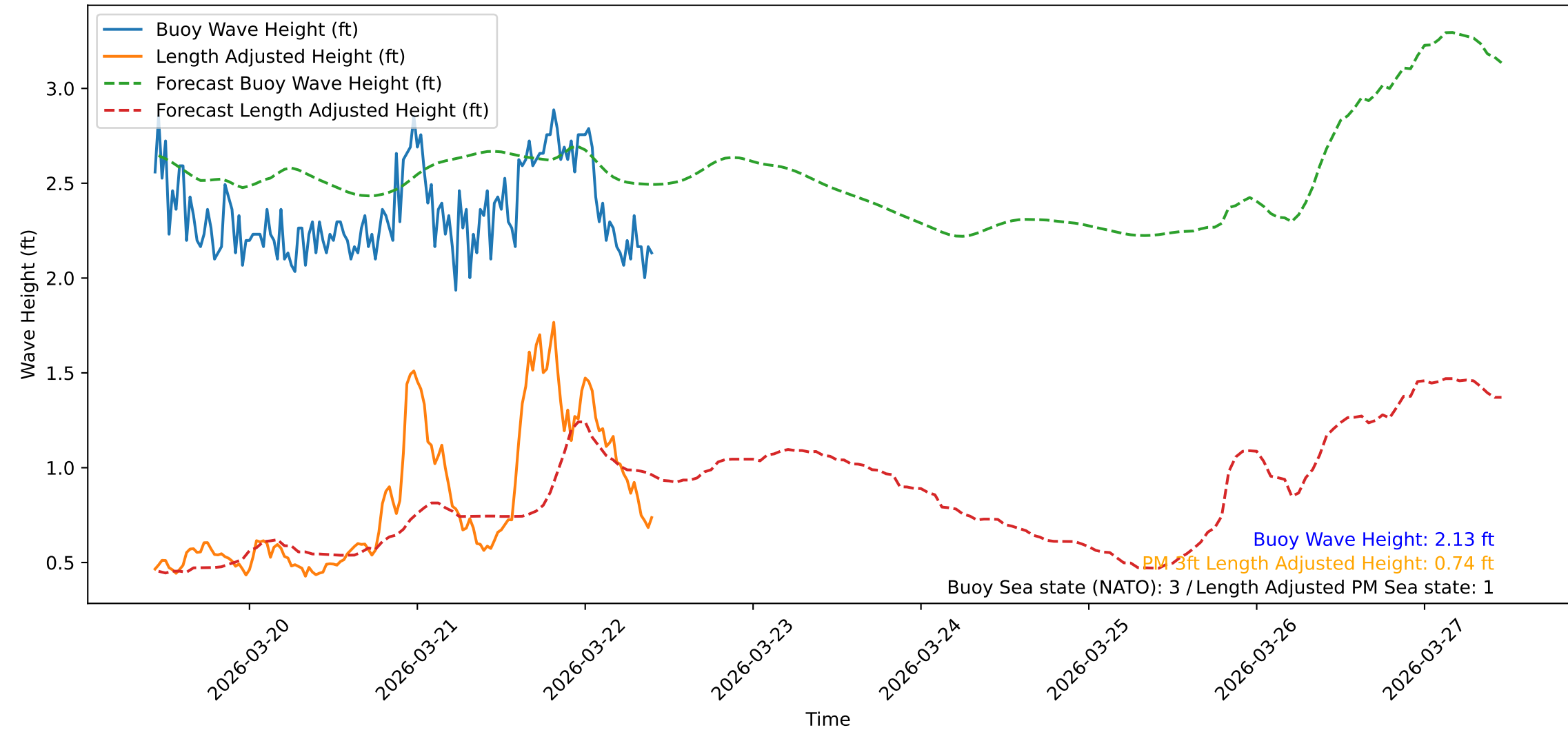
Wave Heights over Time for Green Beach at 2026-03-22 10:31:10
