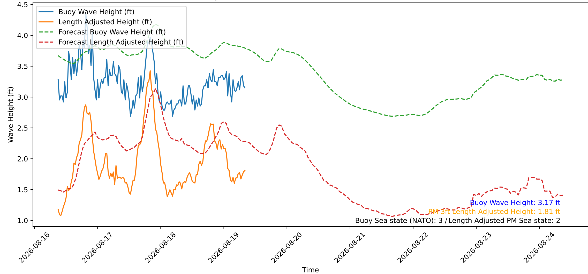
Wave Heights over Time for Green Beach at 2026-08-19 08:41:09
