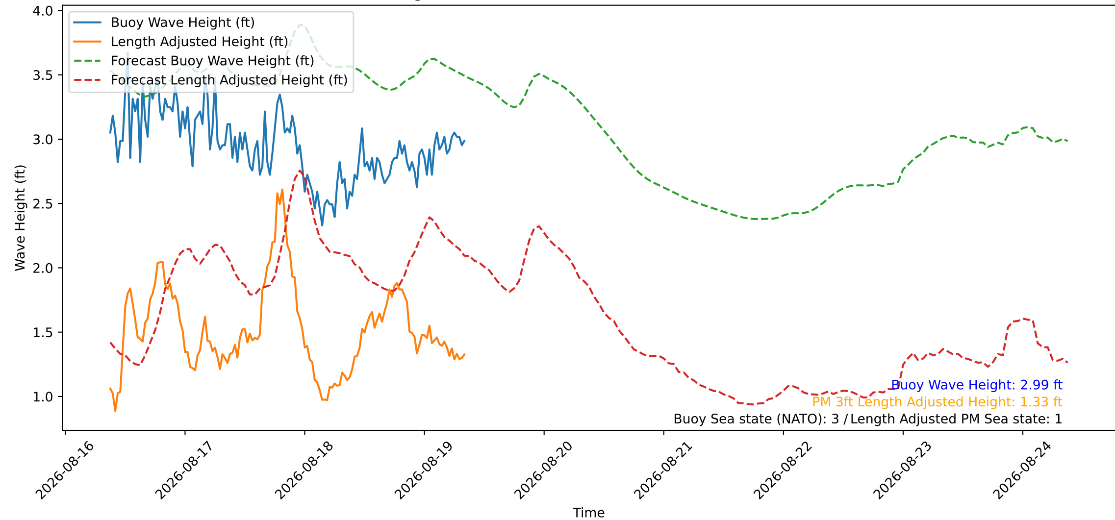
Wave Heights over Time for Red Beach at 2026-08-19 08:40:46
