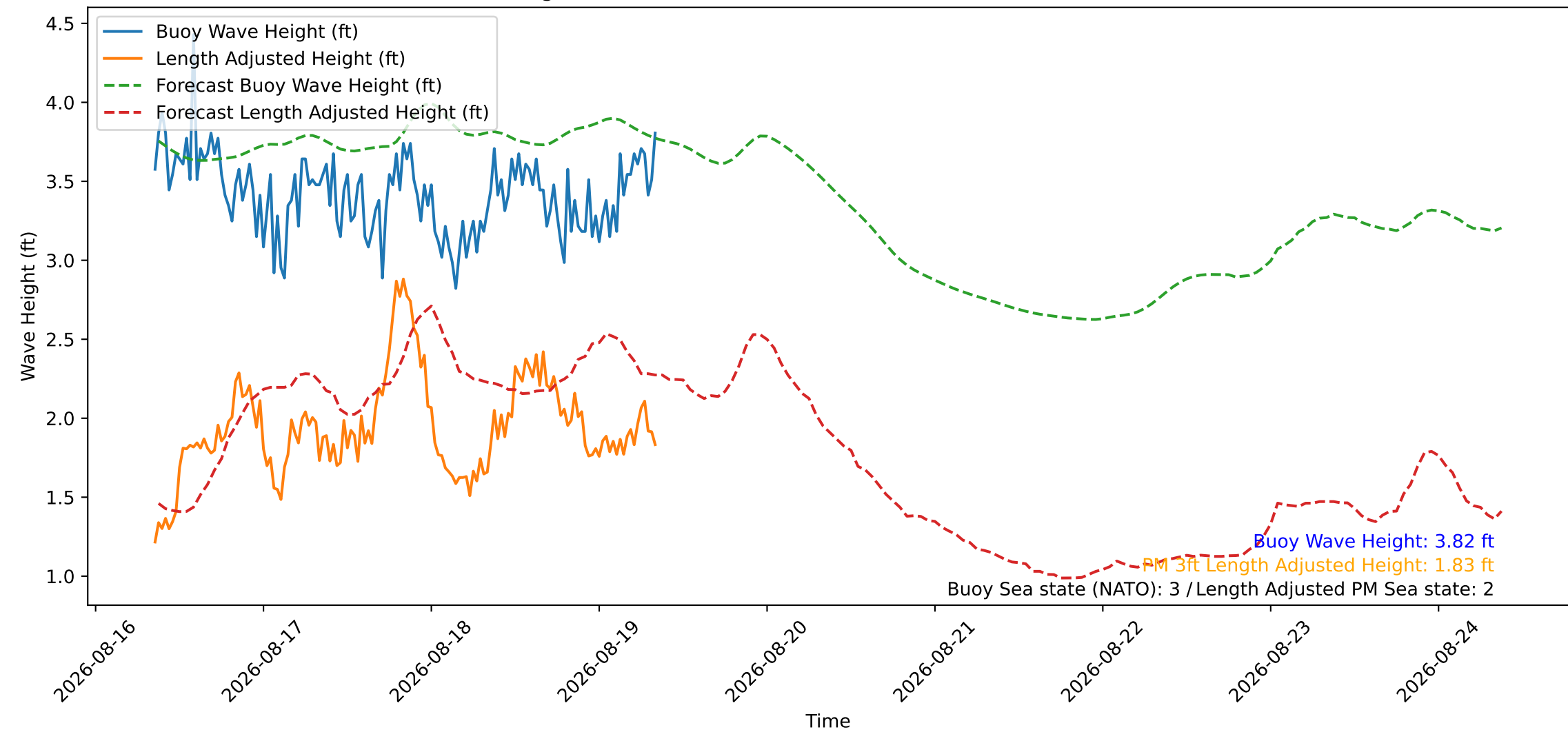
Wave Heights over Time for Oceanside Harbor at 2026-08-19 08:40:26
