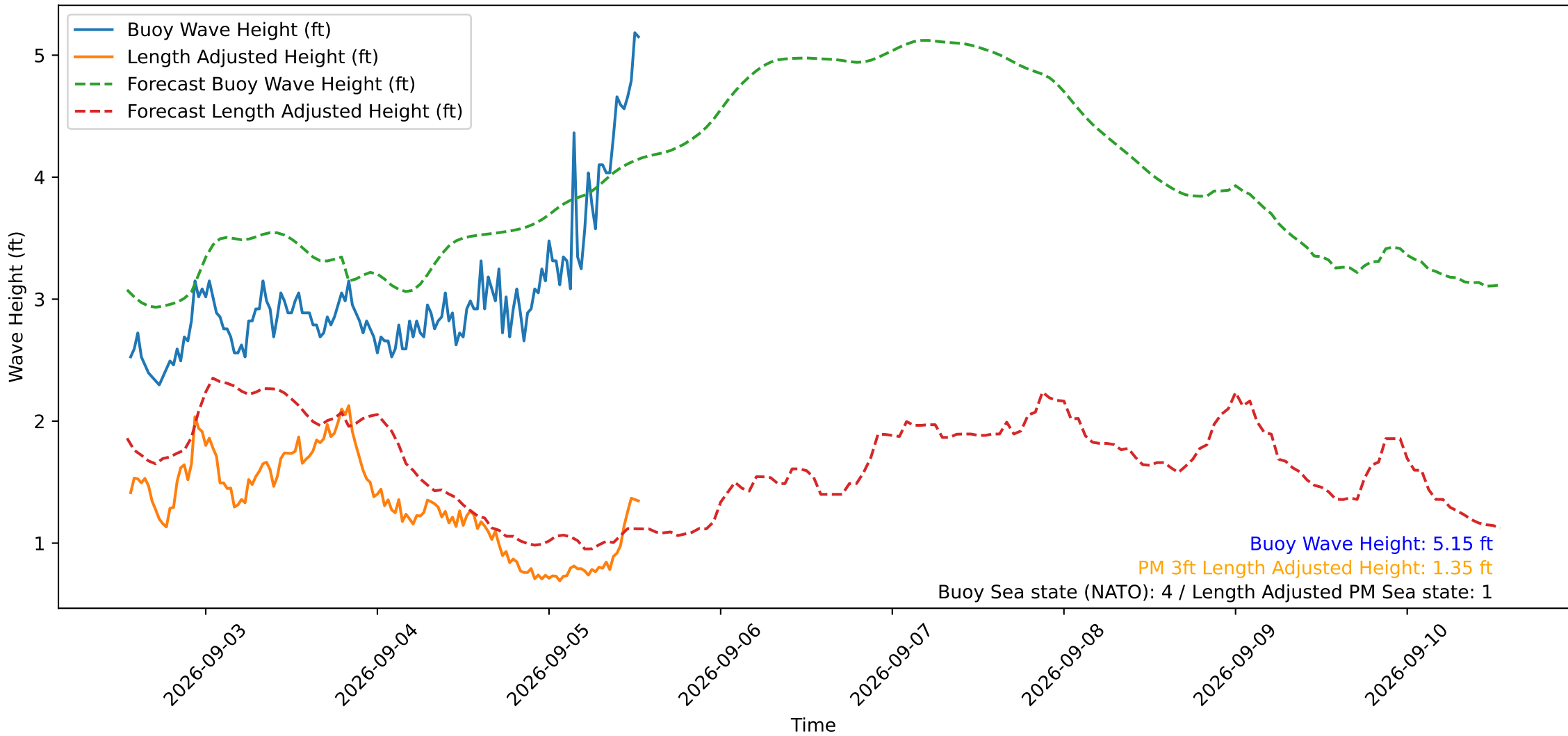
Wave Heights over Time for Red Beach at 2026-09-05 13:20:51
