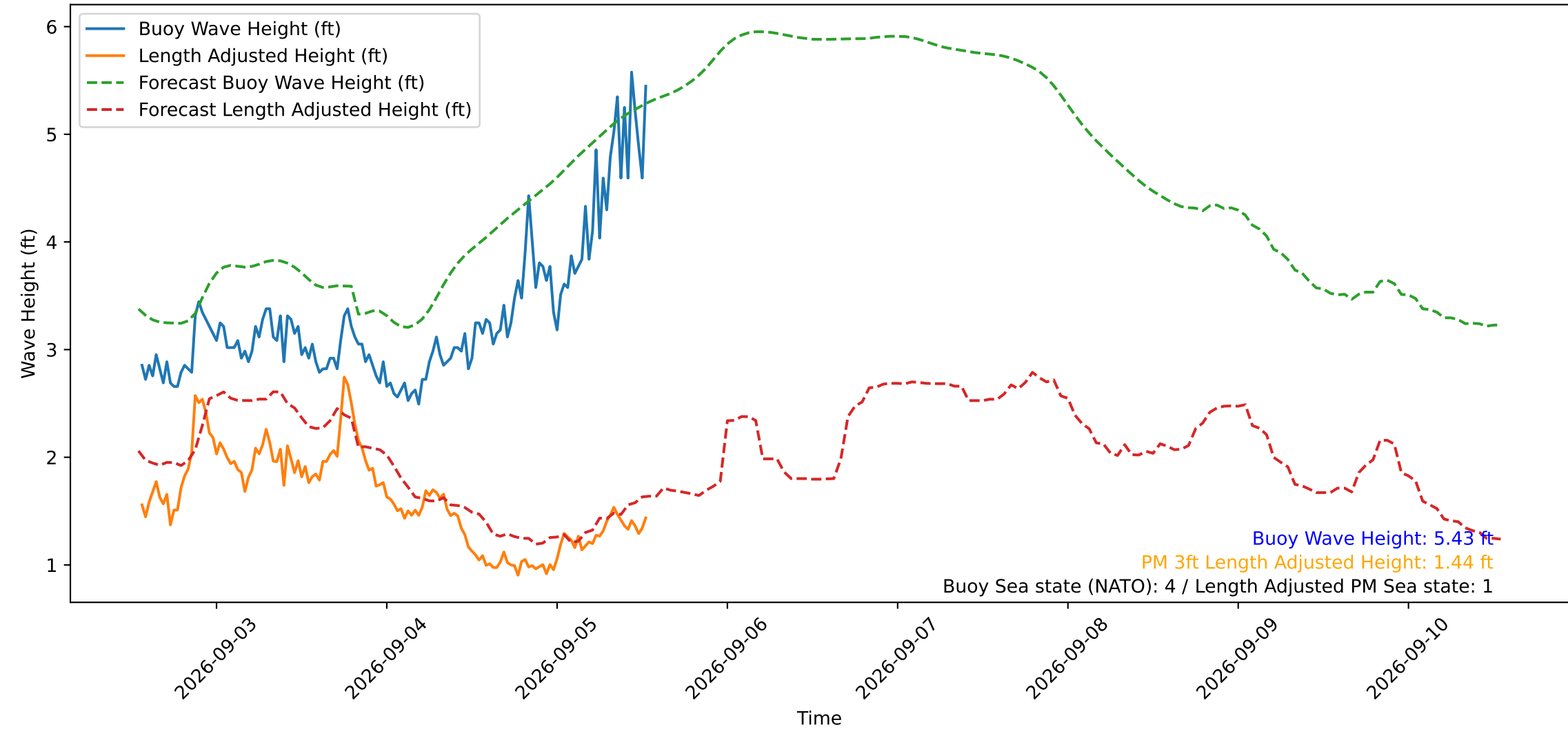
Wave Heights over Time for Green Beach at 2026-09-05 13:21:16
