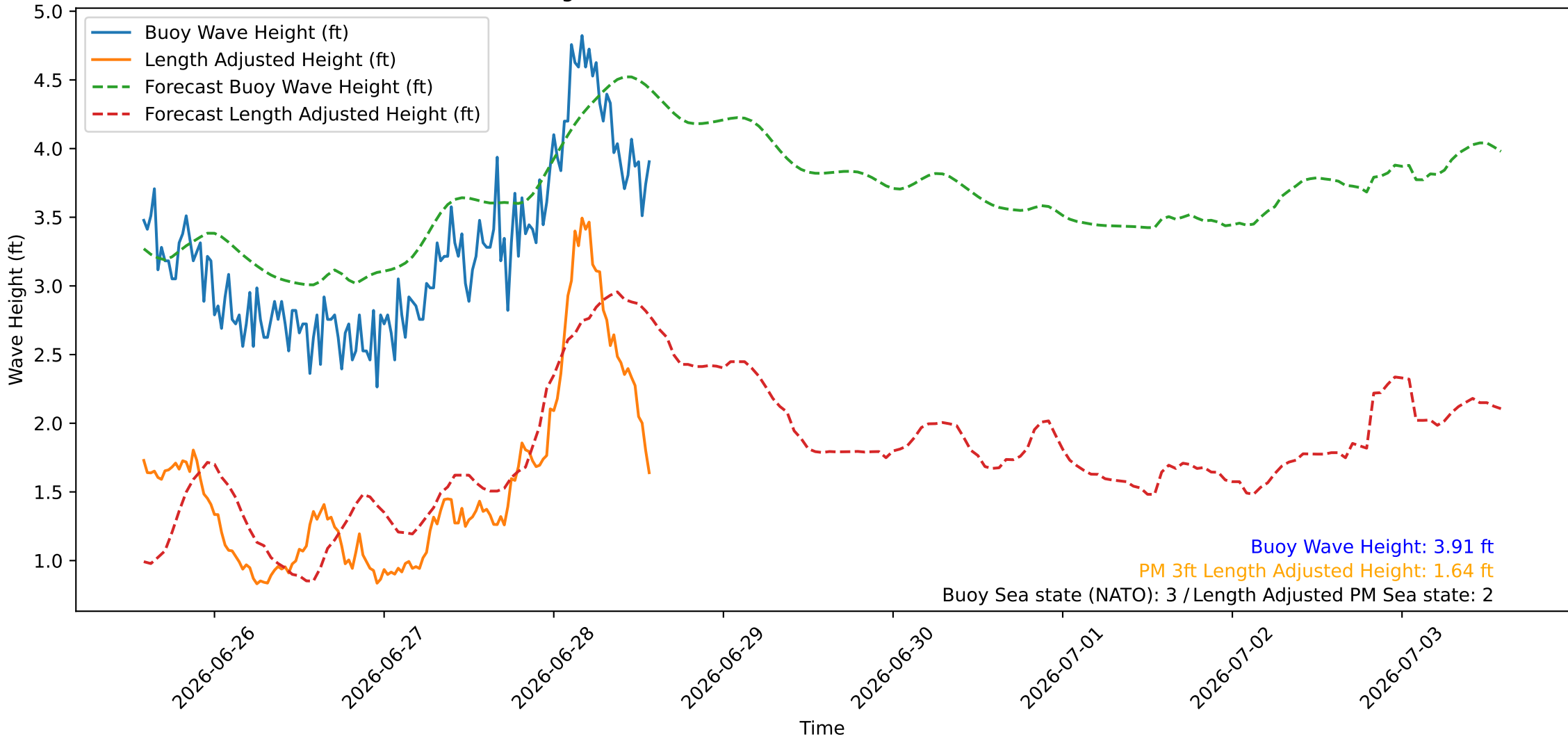
Wave Heights over Time for Green Beach at 2026-06-28 14:11:09
