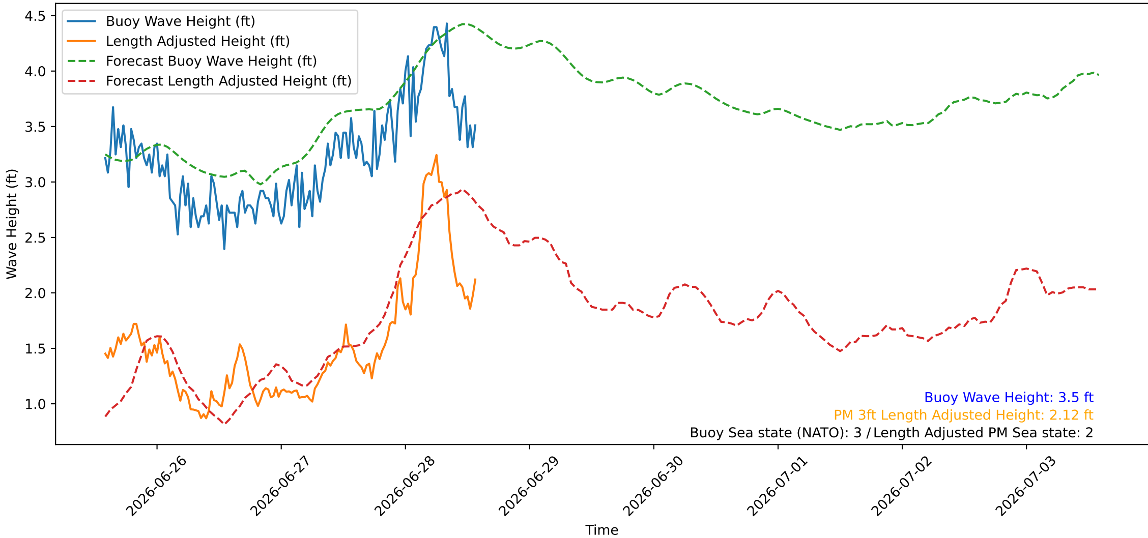
Wave Heights over Time for Oceanside Harbor at 2026-06-28 14:10:26
