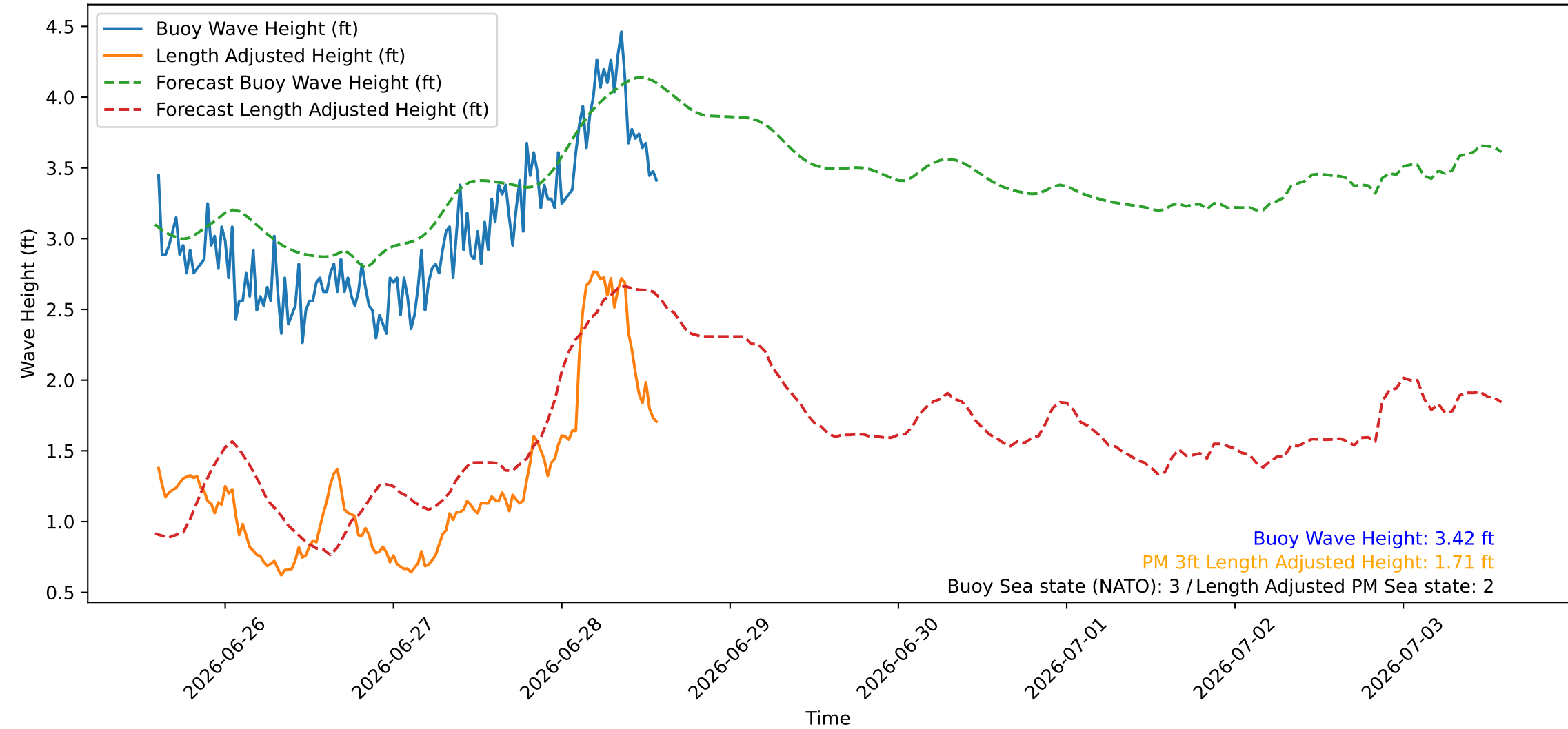
Wave Heights over Time for Red Beach at 2026-06-28 14:10:46
