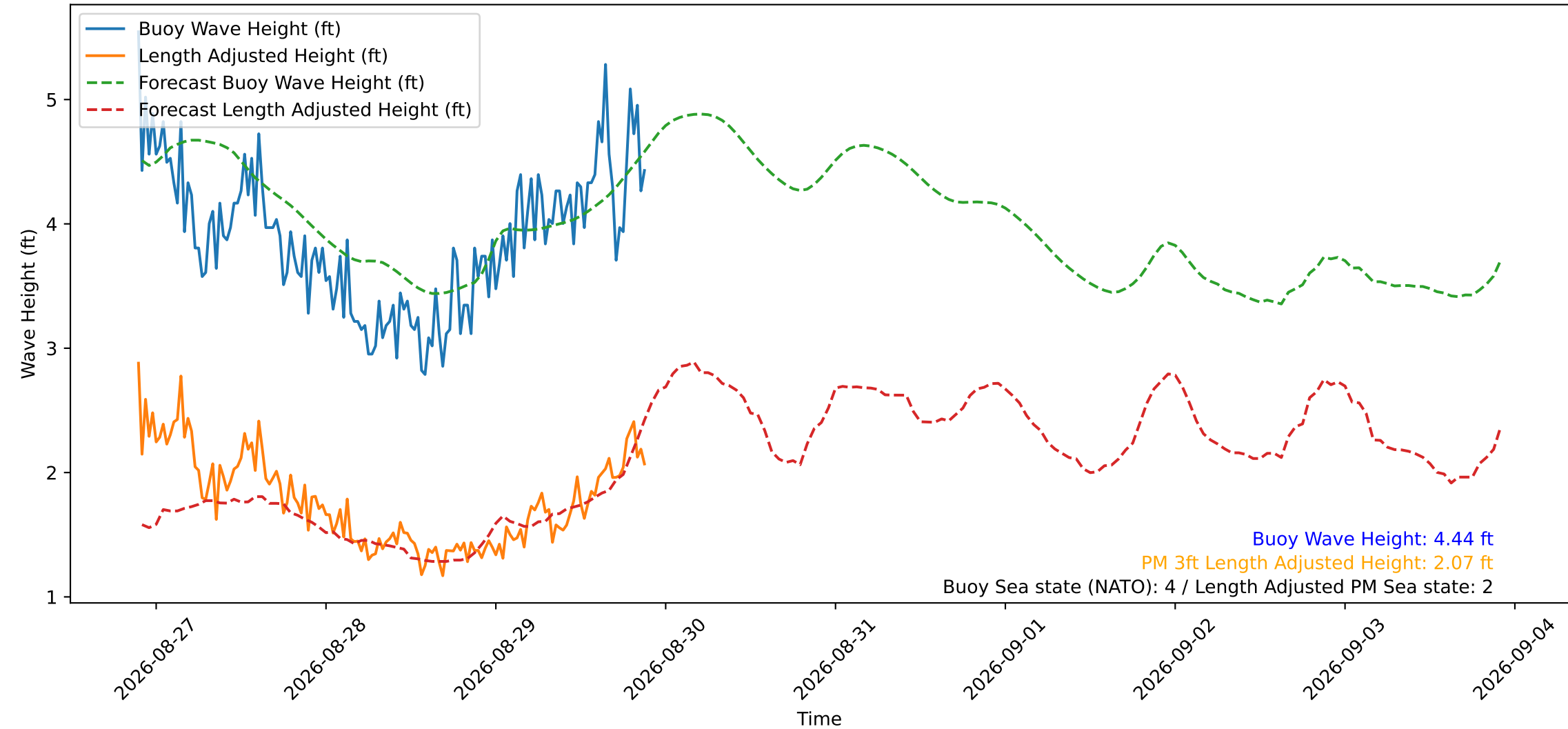
Wave Heights over Time for Oceanside Harbor at 2026-08-29 21:40:29
