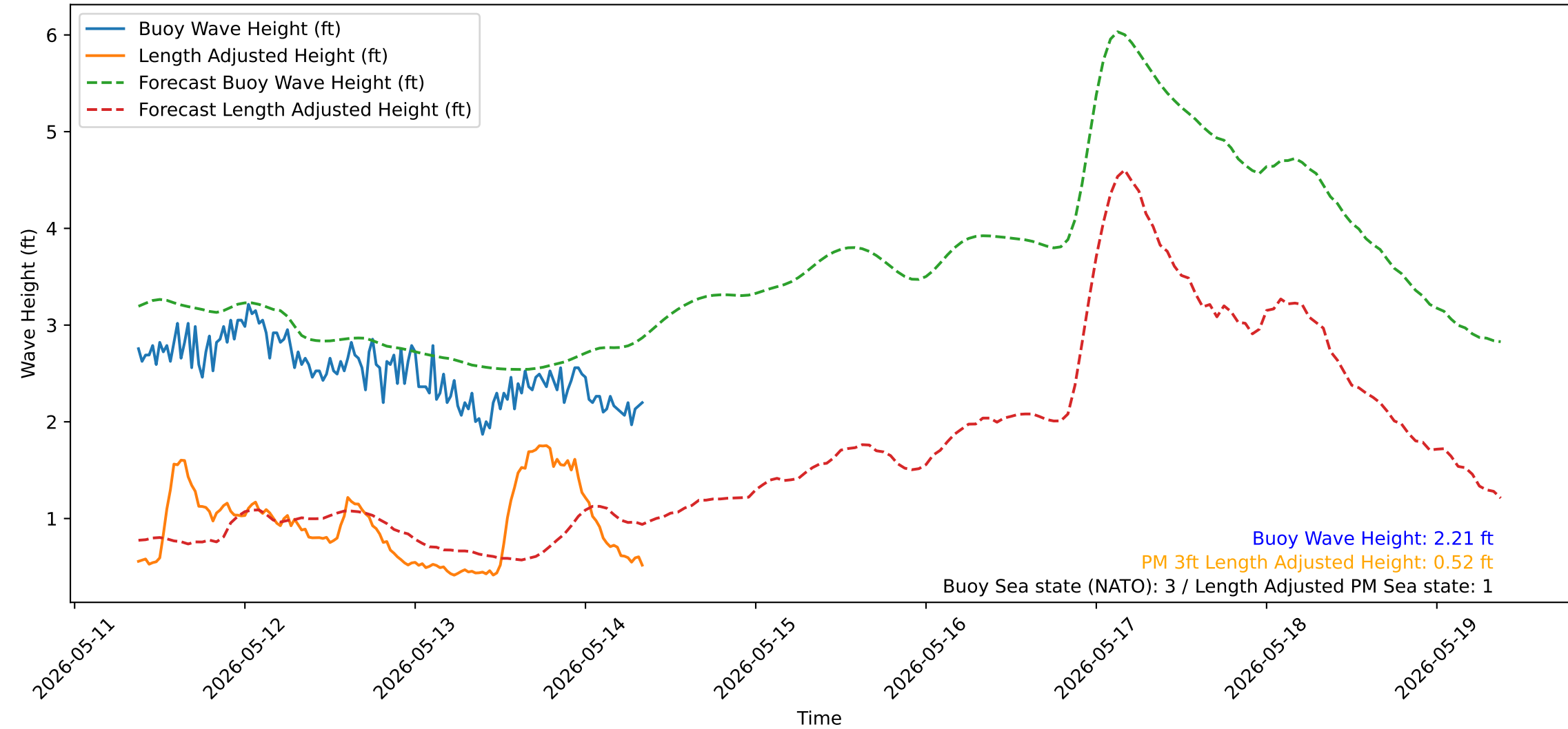
Wave Heights over Time for Red Beach at 2026-05-14 08:40:51
