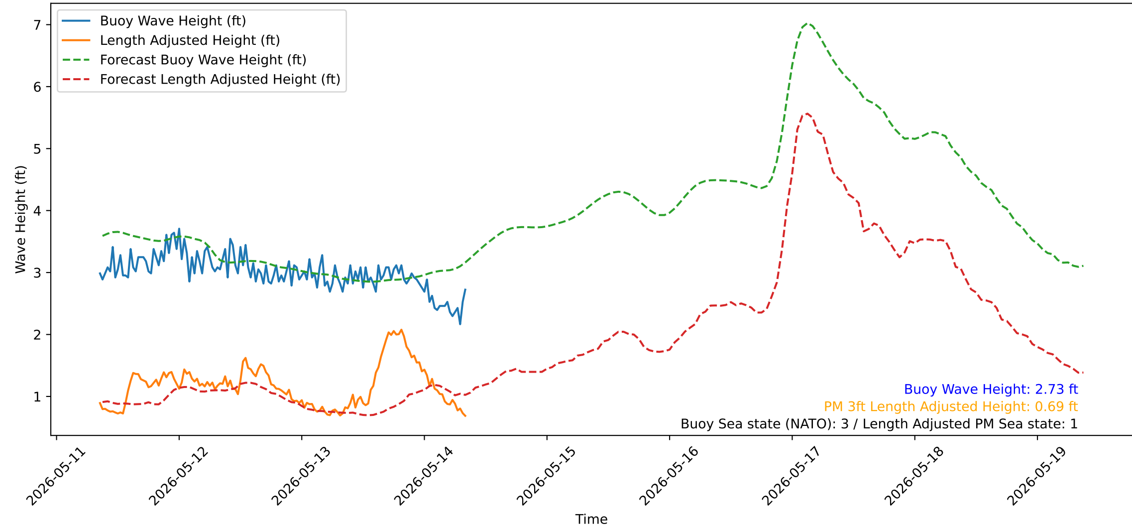
Wave Heights over Time for Oceanside Harbor at 2026-05-14 08:40:32
