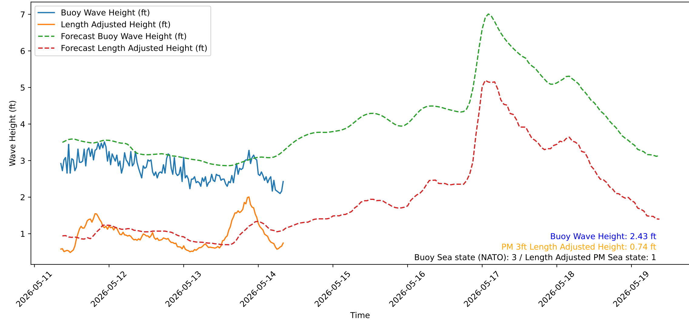
Wave Heights over Time for Green Beach at 2026-05-14 08:41:14
