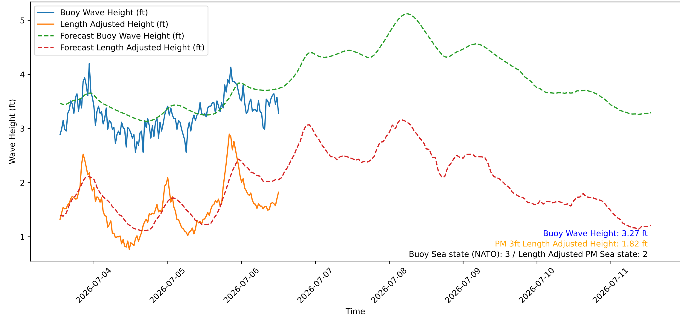
Wave Heights over Time for Green Beach at 2026-07-06 12:51:09
