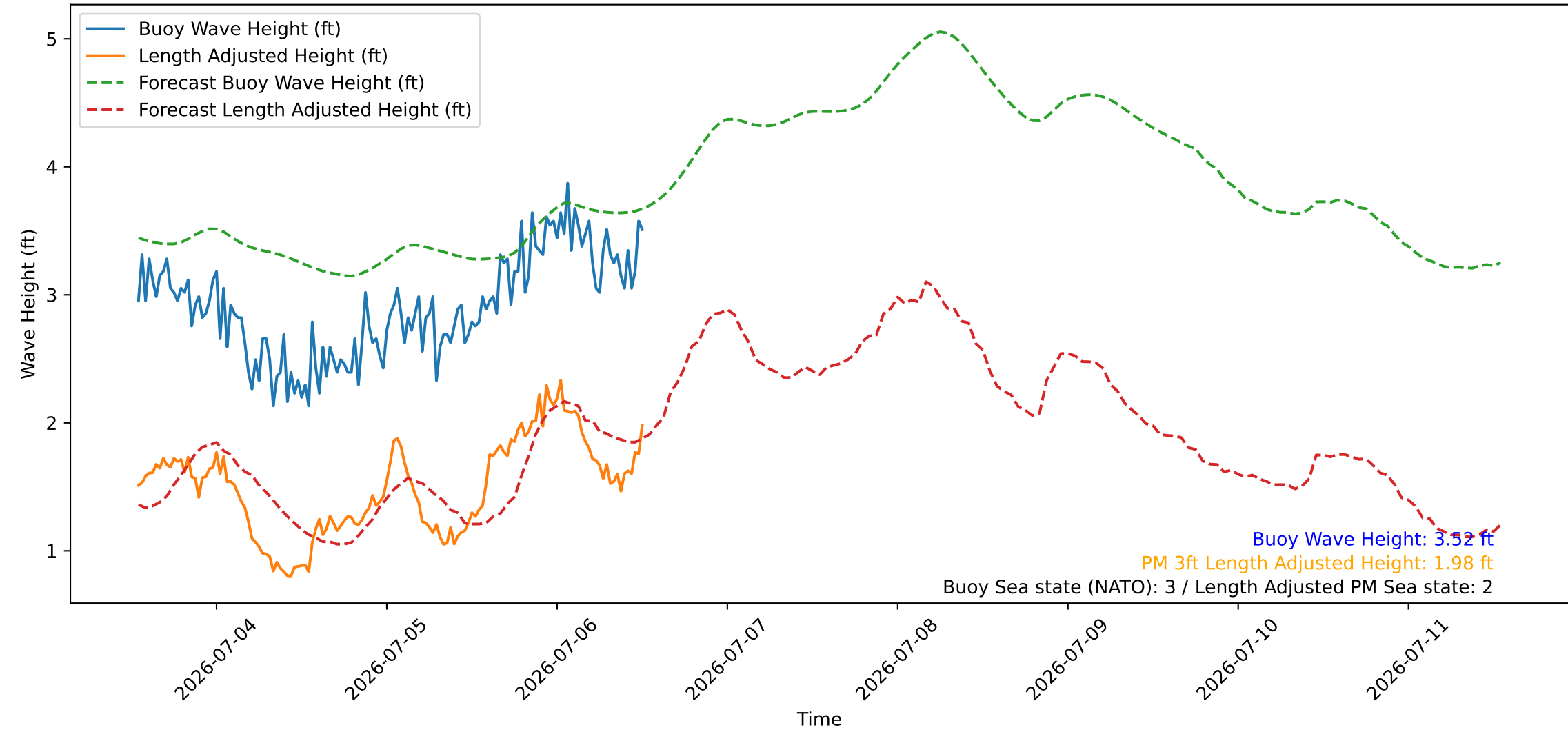
Wave Heights over Time for Oceanside Harbor at 2026-07-06 12:50:26
