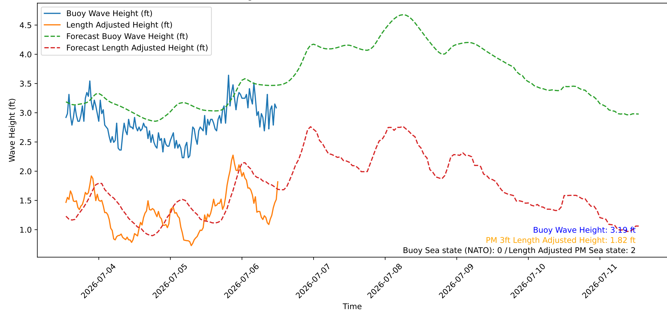
Wave Heights over Time for Red Beach at 2026-07-06 12:50:46
