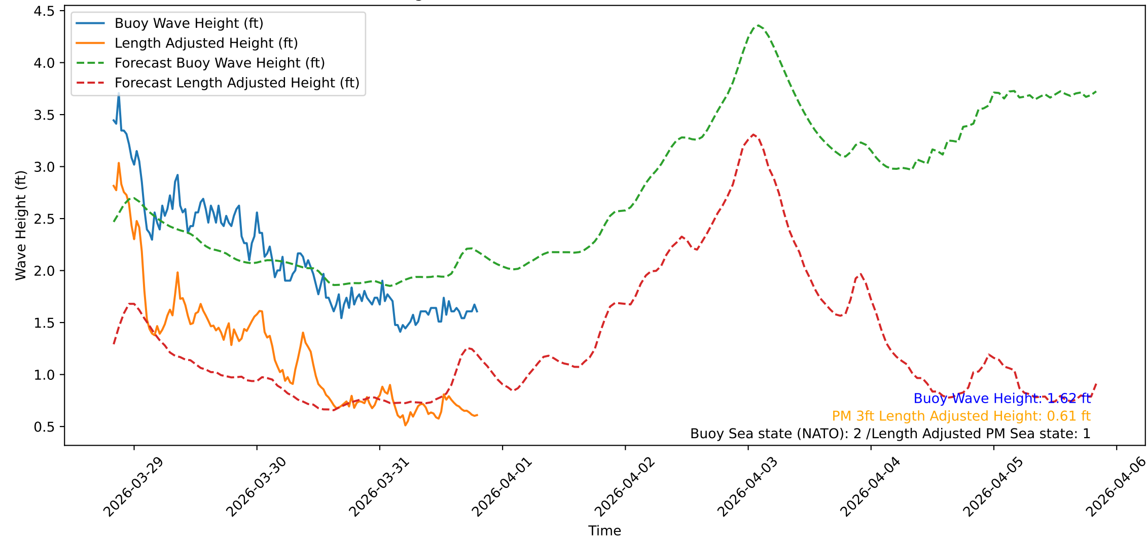
Wave Heights over Time for Green Beach at 2026-03-31 19:51:10
