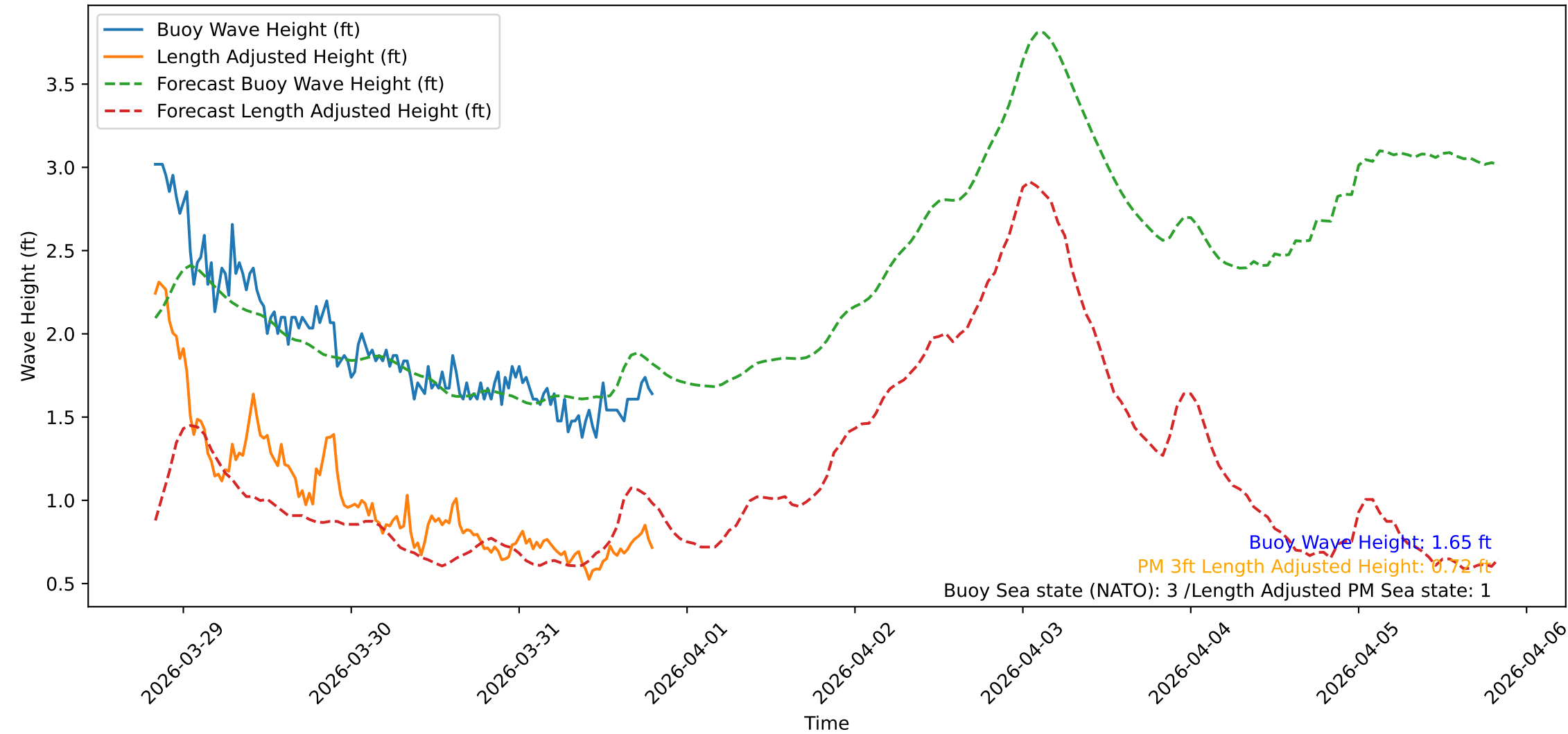
Wave Heights over Time for Red Beach at 2026-03-31 19:50:47
