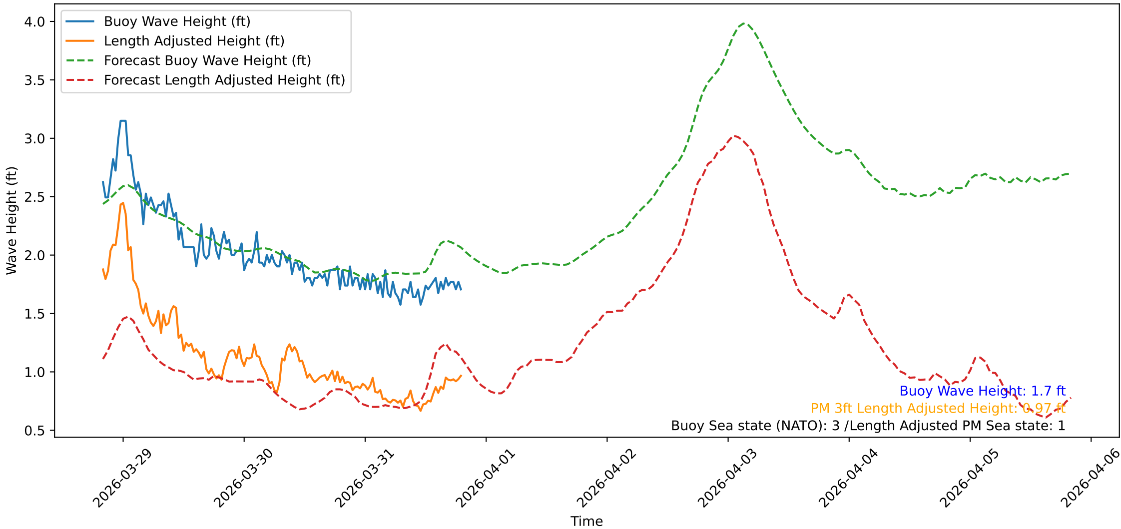
Wave Heights over Time for Oceanside Harbor at 2026-03-31 19:50:31
