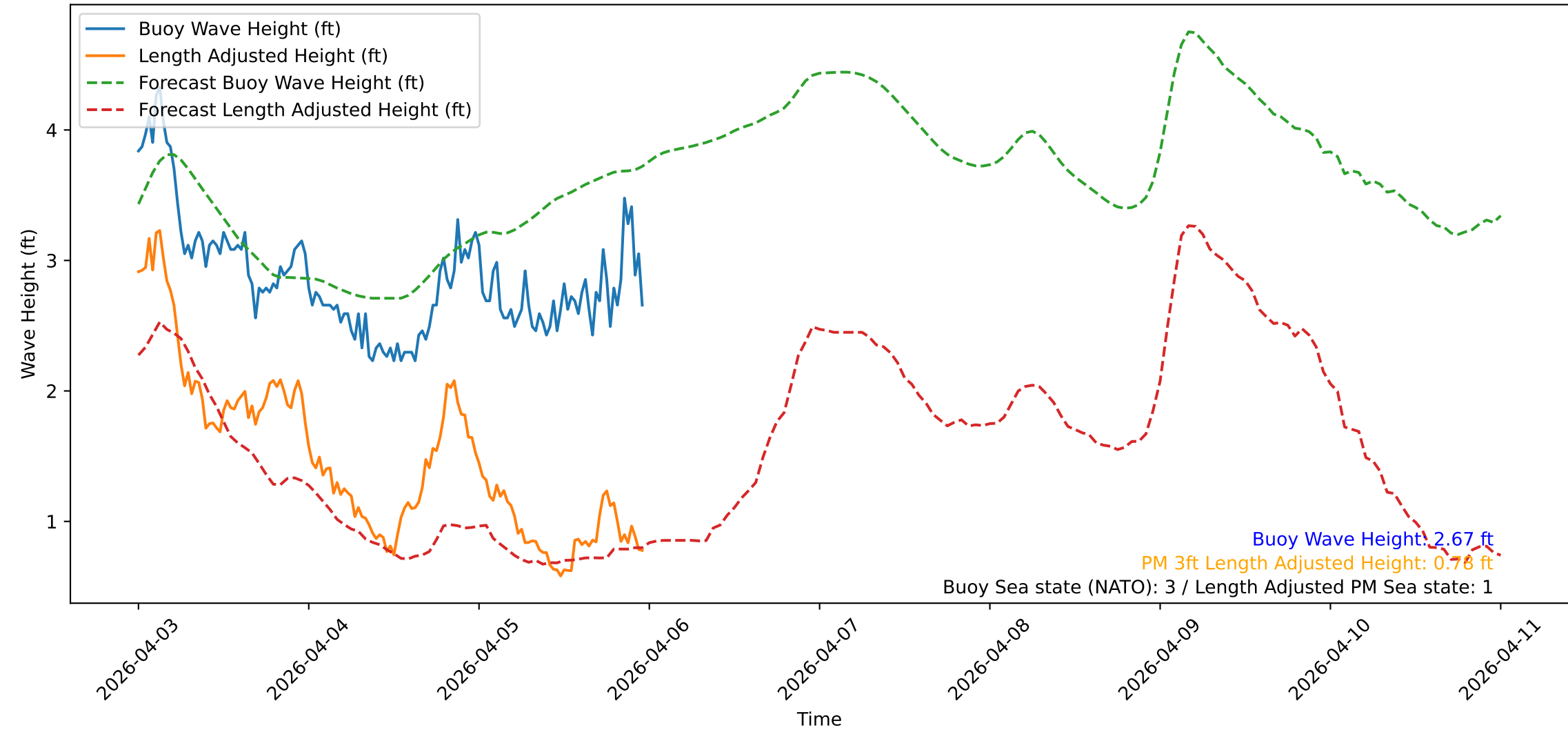
Wave Heights over Time for Green Beach at 2026-04-05 23:51:09
