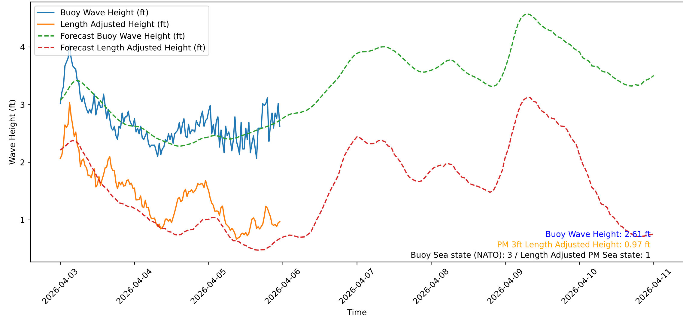
Wave Heights over Time for Oceanside Harbor at 2026-04-05 23:50:31
