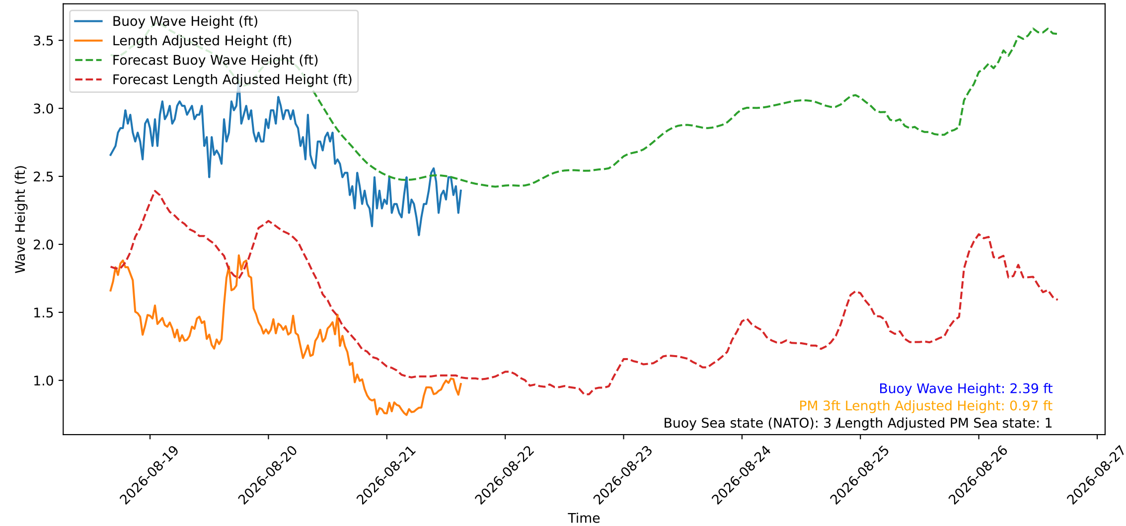
Wave Heights over Time for Red Beach at 2026-08-21 15:40:47
