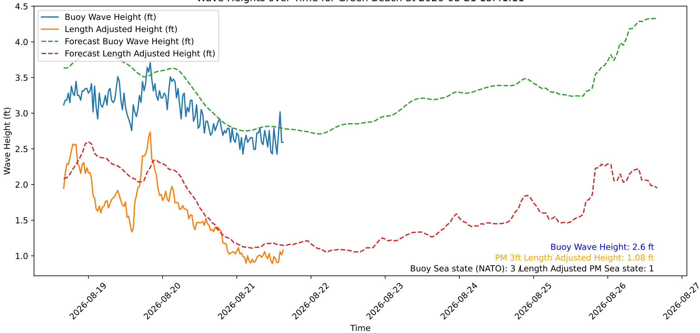
Wave Heights over Time for Green Beach at 2026-08-21 15:41:11
