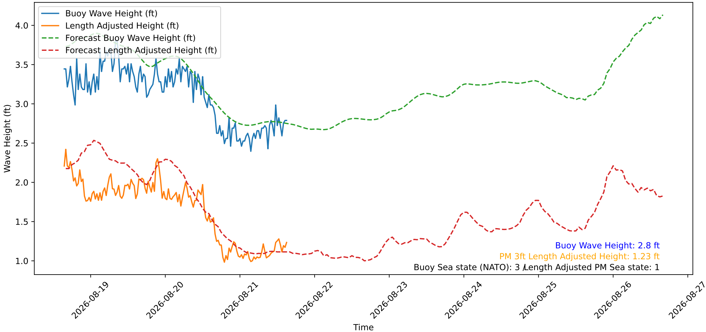
Wave Heights over Time for Oceanside Harbor at 2026-08-21 15:40:27
