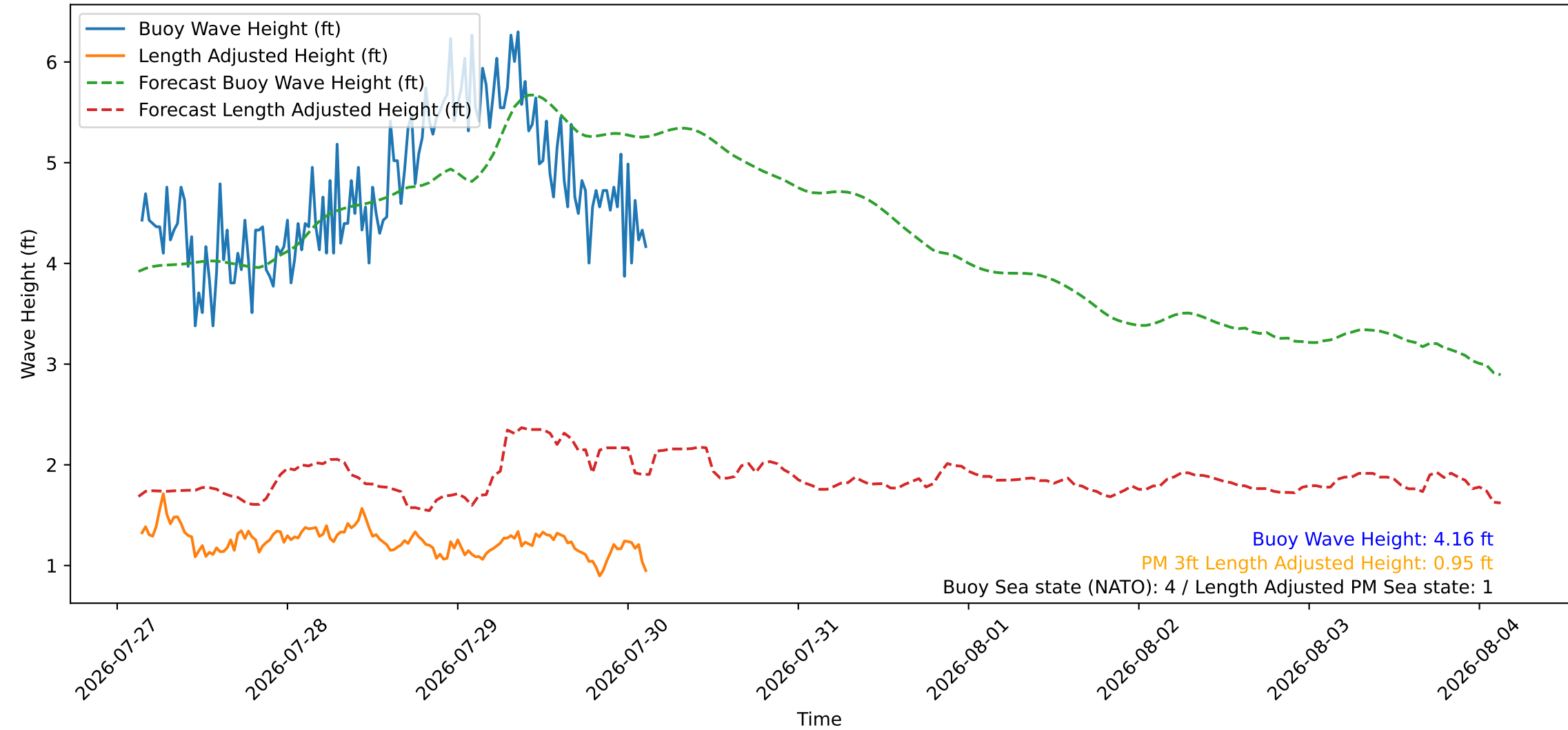
Wave Heights over Time for Green Beach at 2026-07-30 03:21:10
