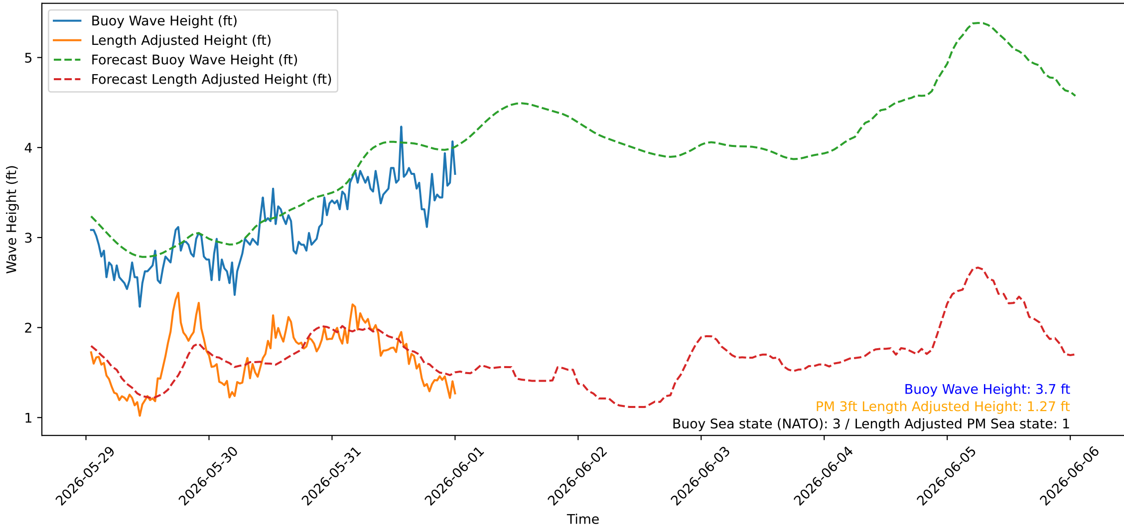
Wave Heights over Time for Oceanside Harbor at 2026-06-01 01:00:26
