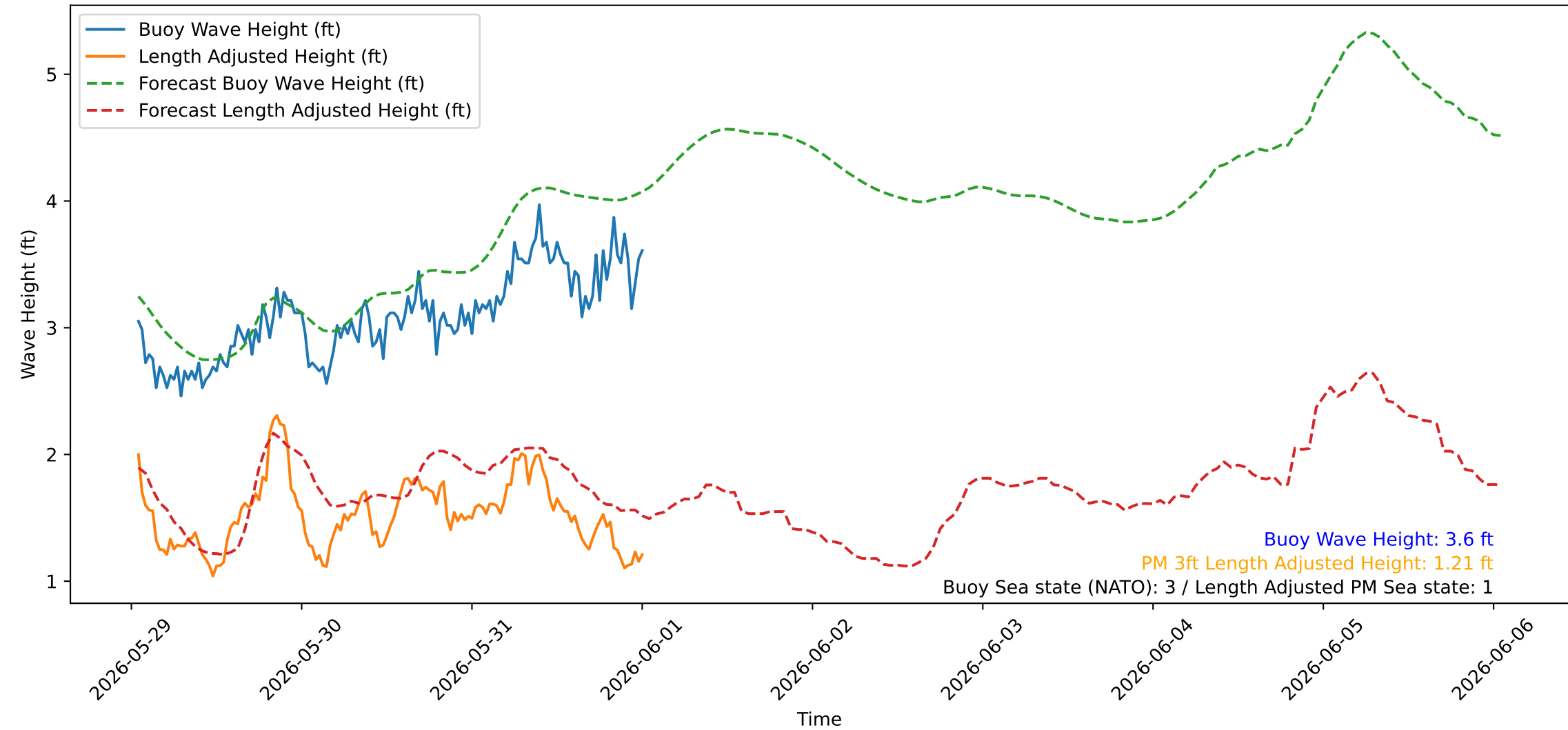
Wave Heights over Time for Green Beach at 2026-06-01 01:01:07
