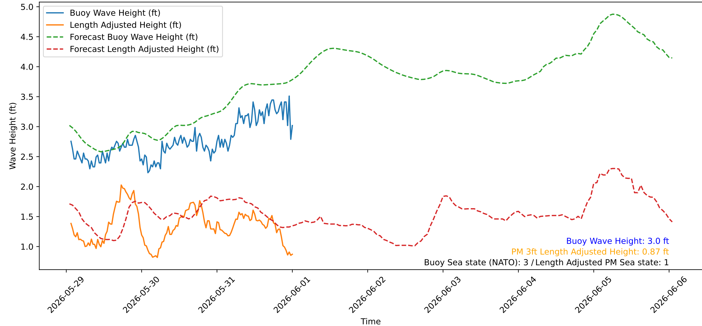
Wave Heights over Time for Red Beach at 2026-06-01 01:00:44
