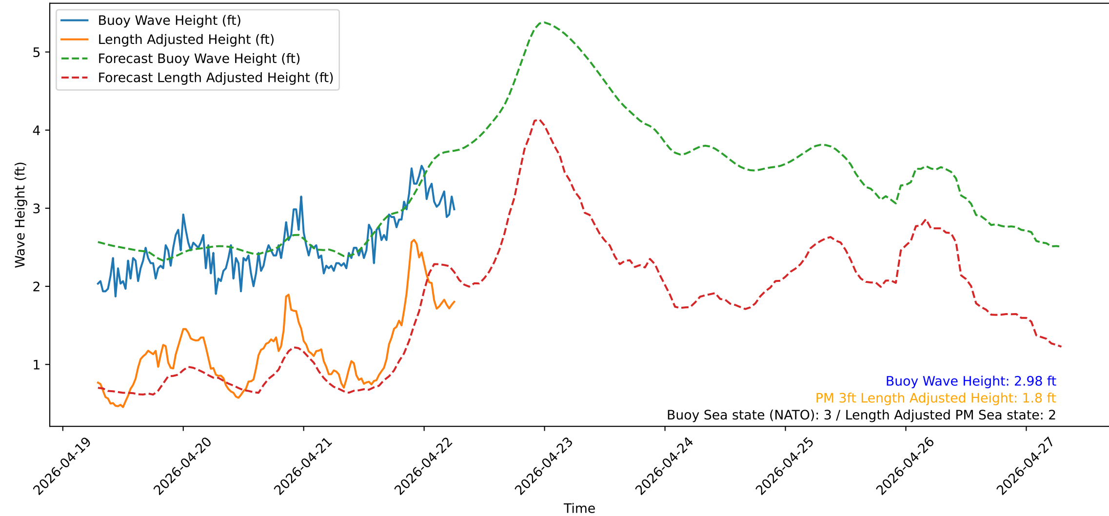
Wave Heights over Time for Green Beach at 2026-04-22 06:51:14
