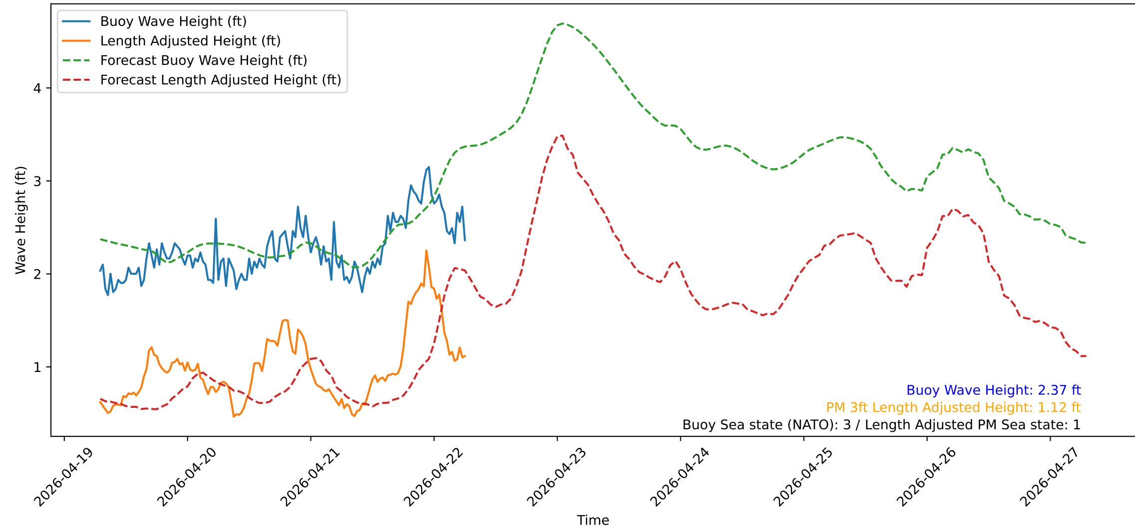
Wave Heights over Time for Red Beach at 2026-04-22 06:50:51
