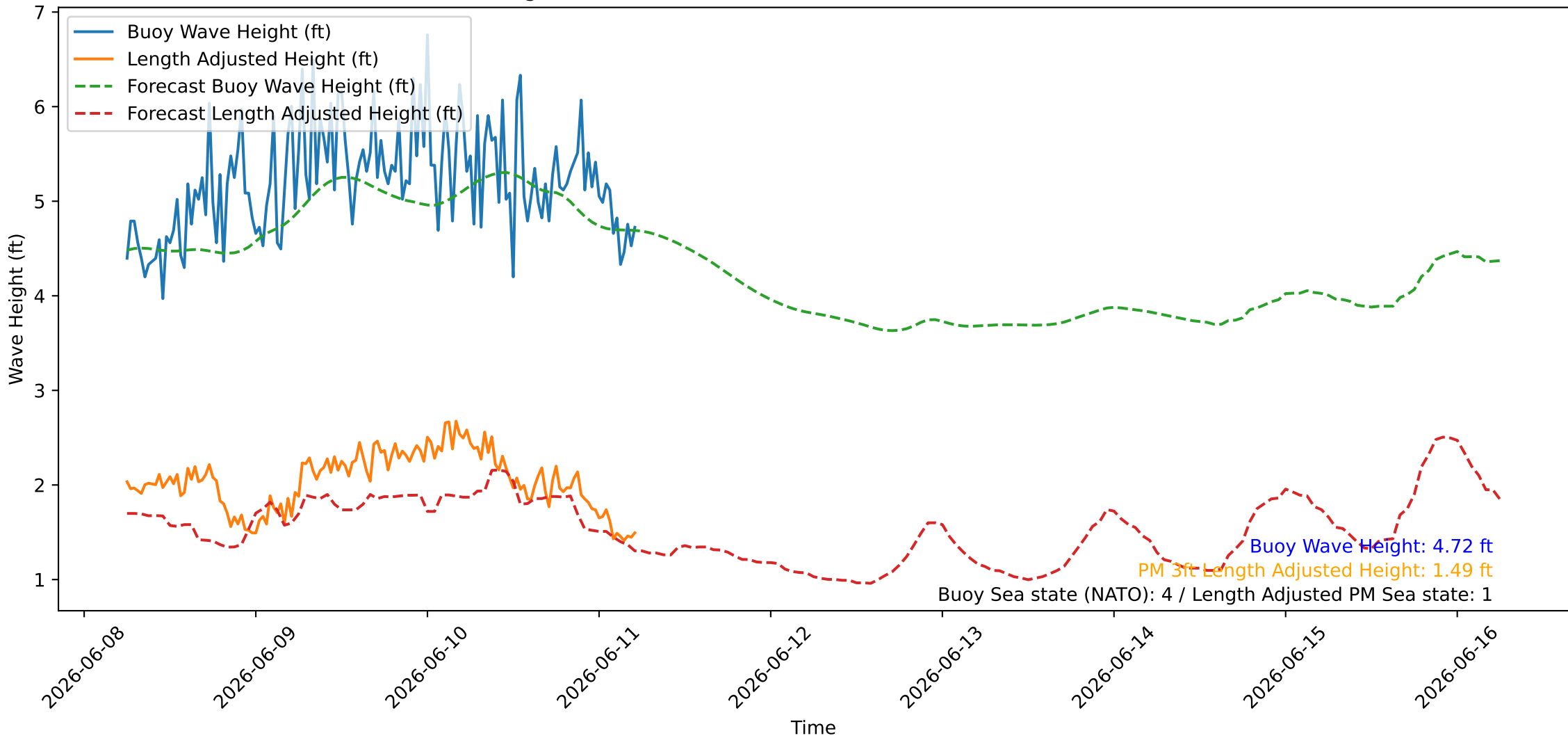
Wave Heights over Time for Oceanside Harbor at 2026-06-11 05:50:26
