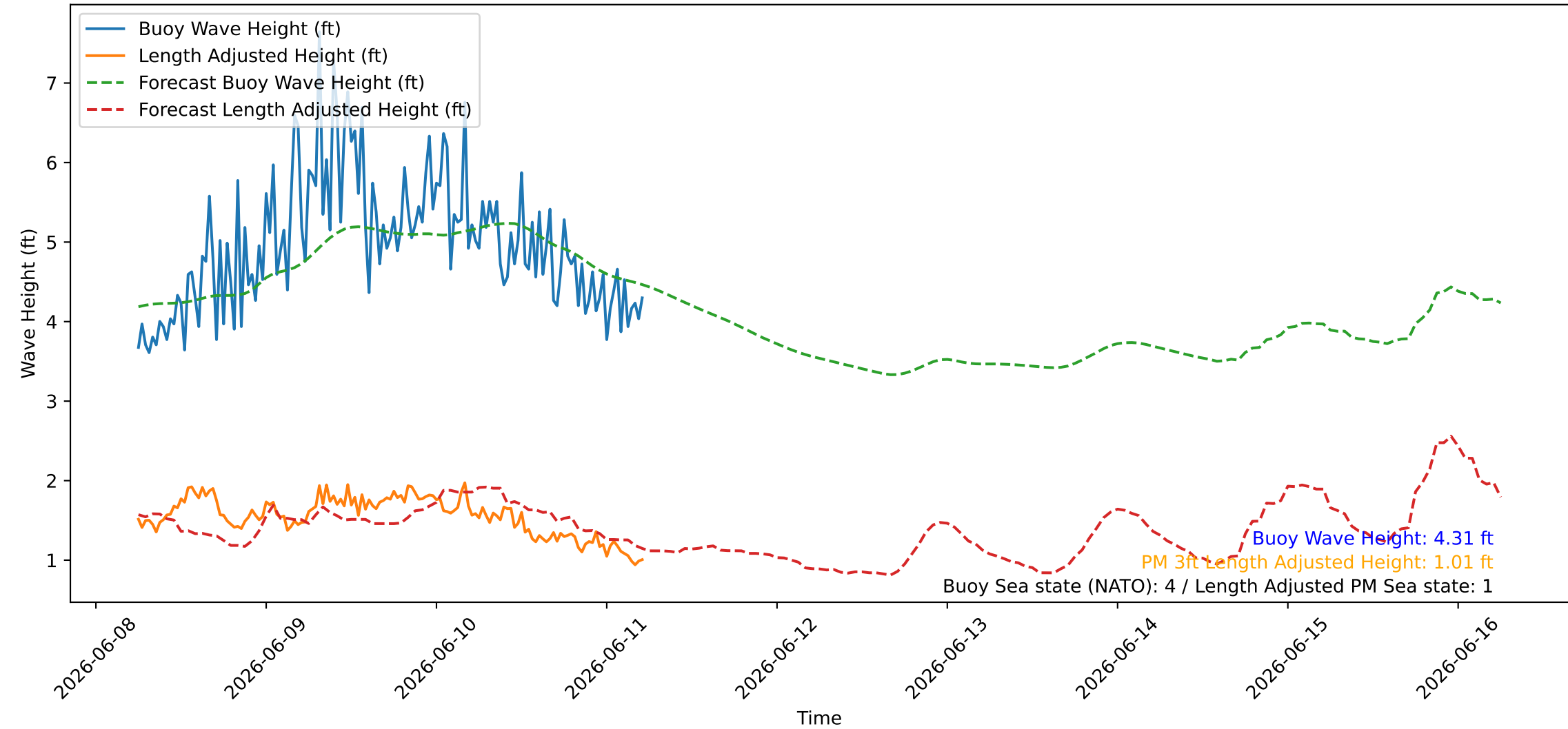
Wave Heights over Time for Red Beach at 2026-06-11 05:50:48
