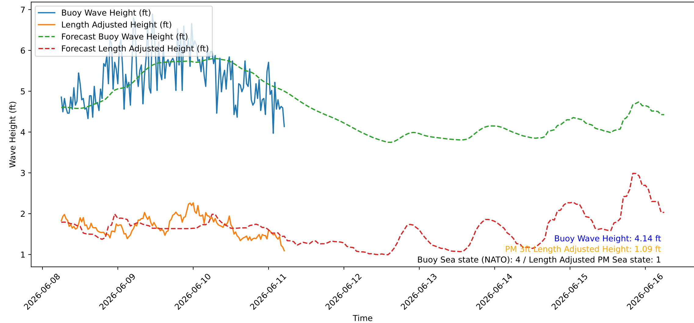
Wave Heights over Time for Green Beach at 2026-06-11 05:51:12
