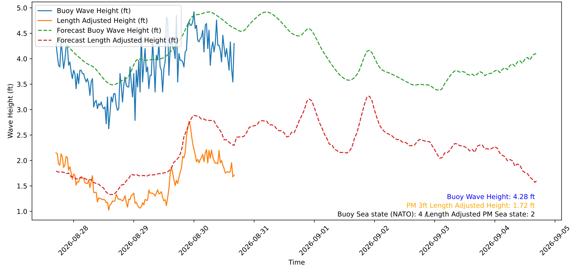
Wave Heights over Time for Green Beach at 2026-08-30 16:51:14
