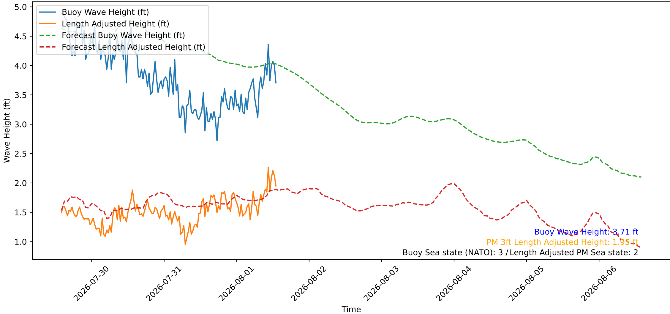
Wave Heights over Time for Oceanside Harbor at 2026-08-01 13:50:26
