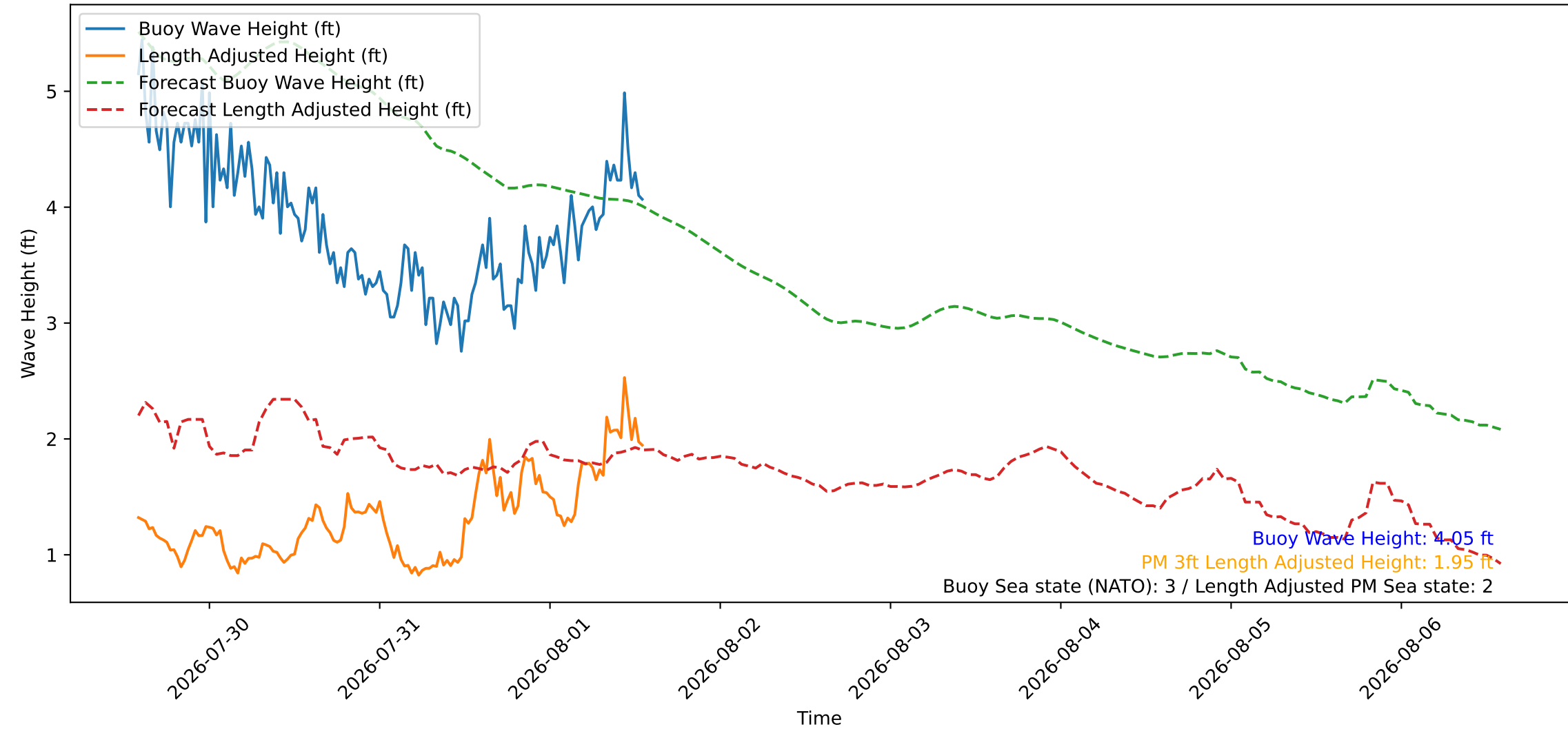
Wave Heights over Time for Green Beach at 2026-08-01 13:51:10
