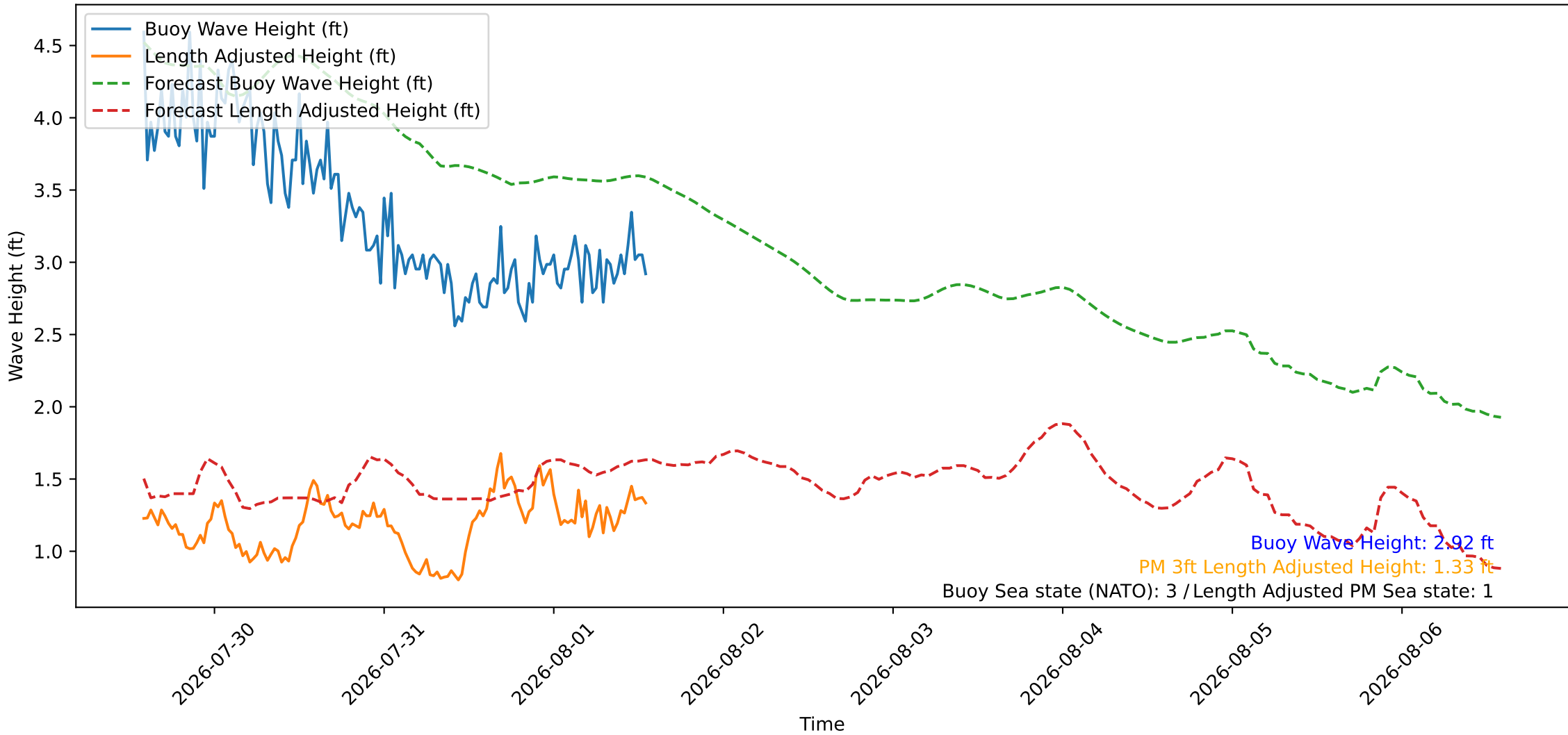
Wave Heights over Time for Red Beach at 2026-08-01 13:50:47
