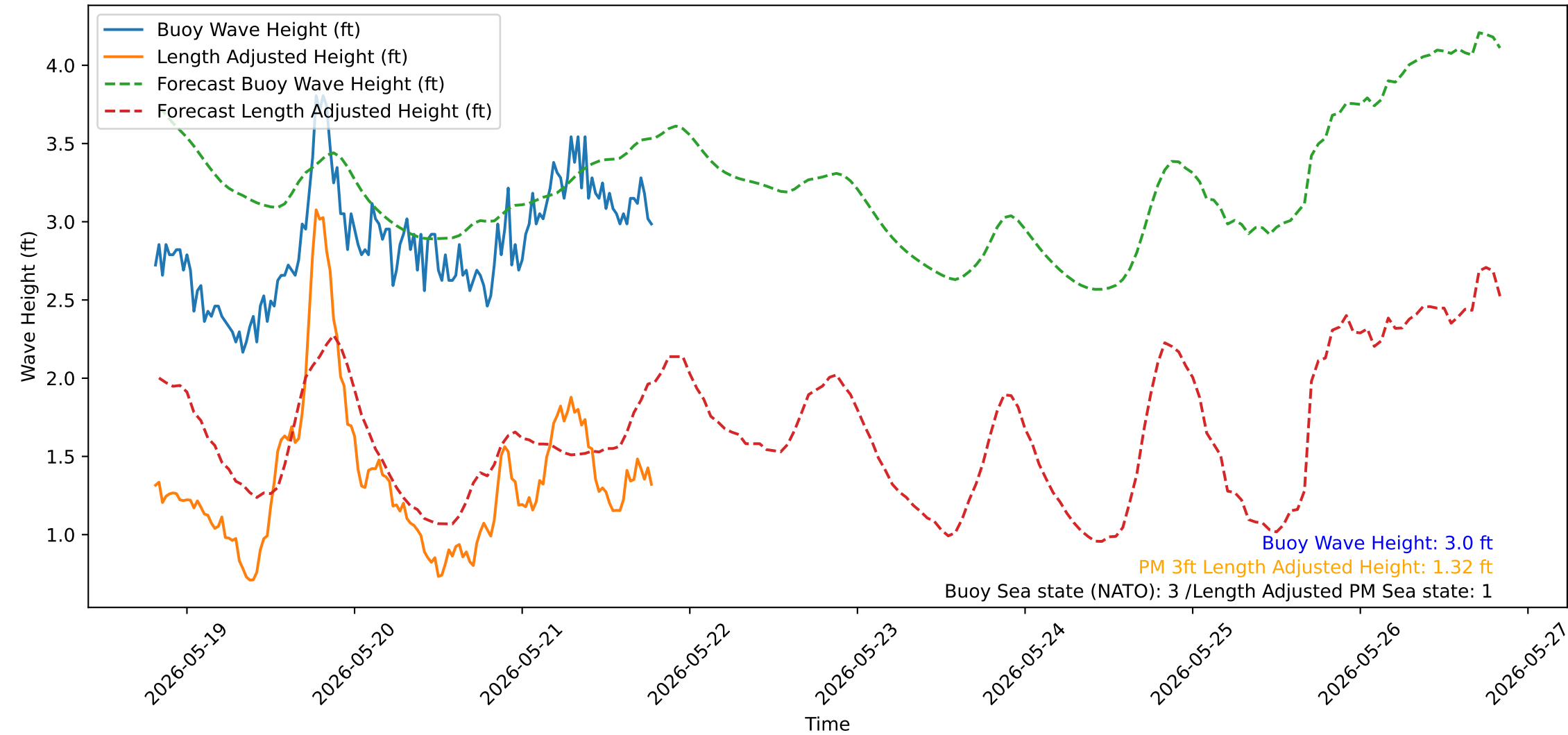
Wave Heights over Time for Green Beach at 2026-05-21 19:31:14
