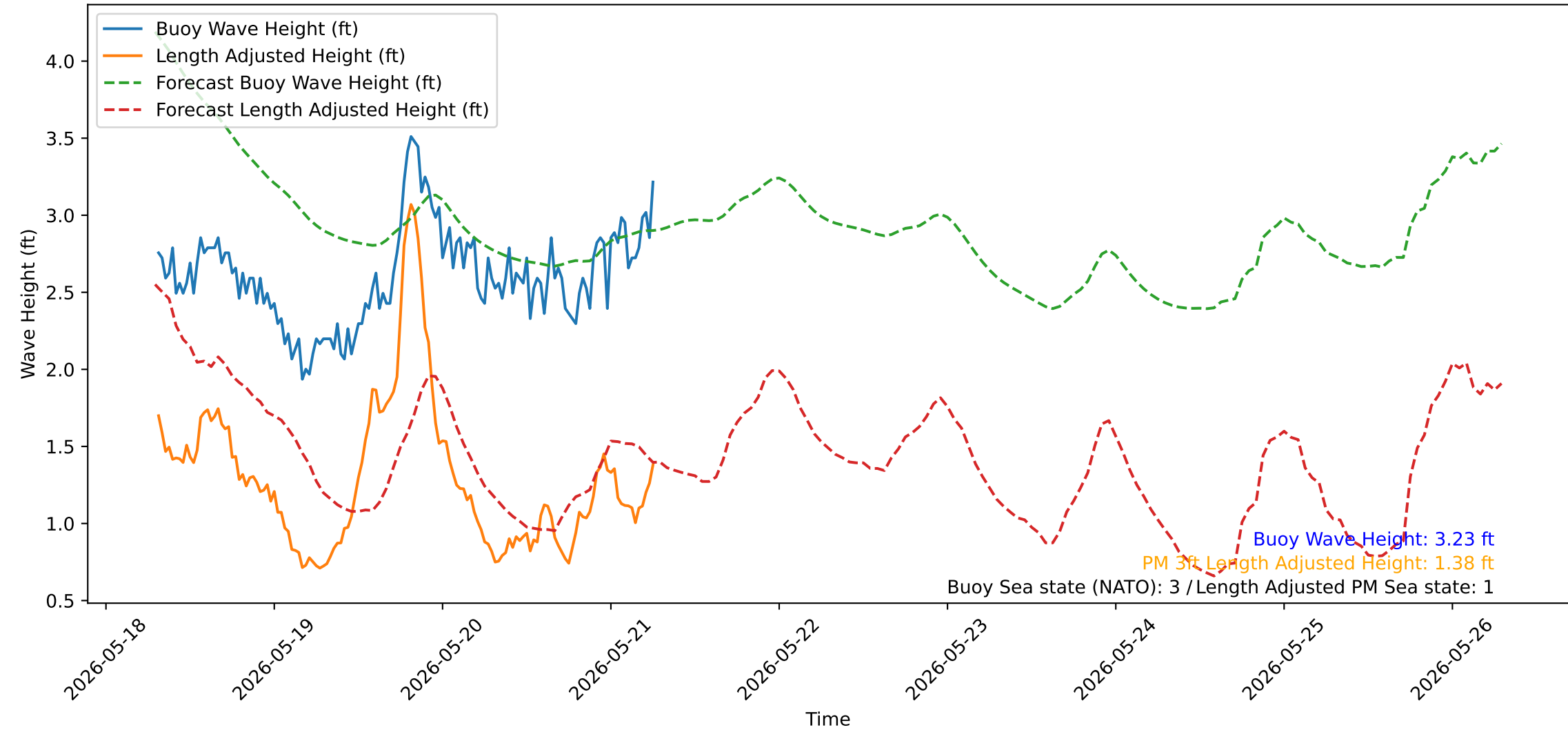
Wave Heights over Time for Red Beach at 2026-05-21 07:00:51
