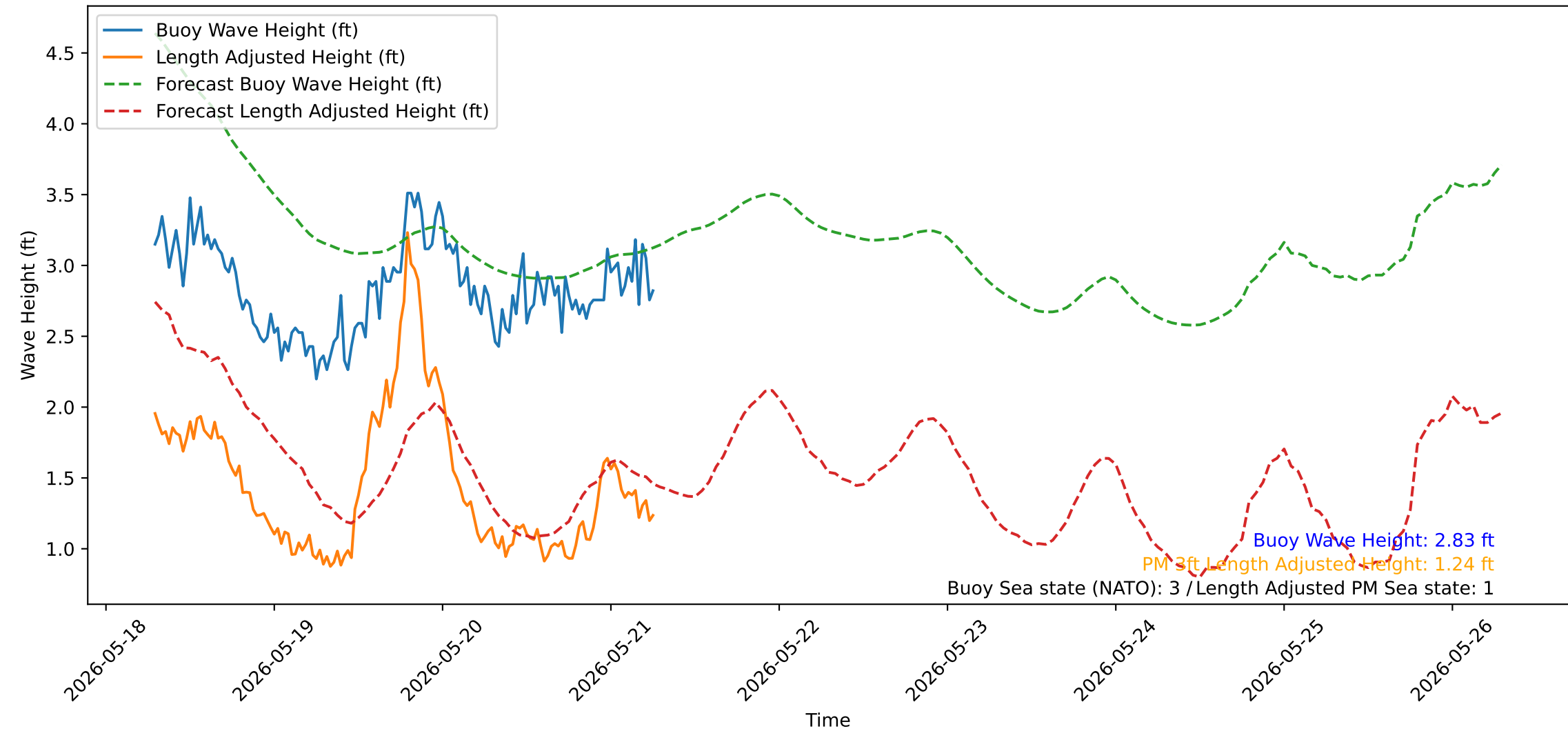
Wave Heights over Time for Oceanside Harbor at 2026-05-21 07:00:31
