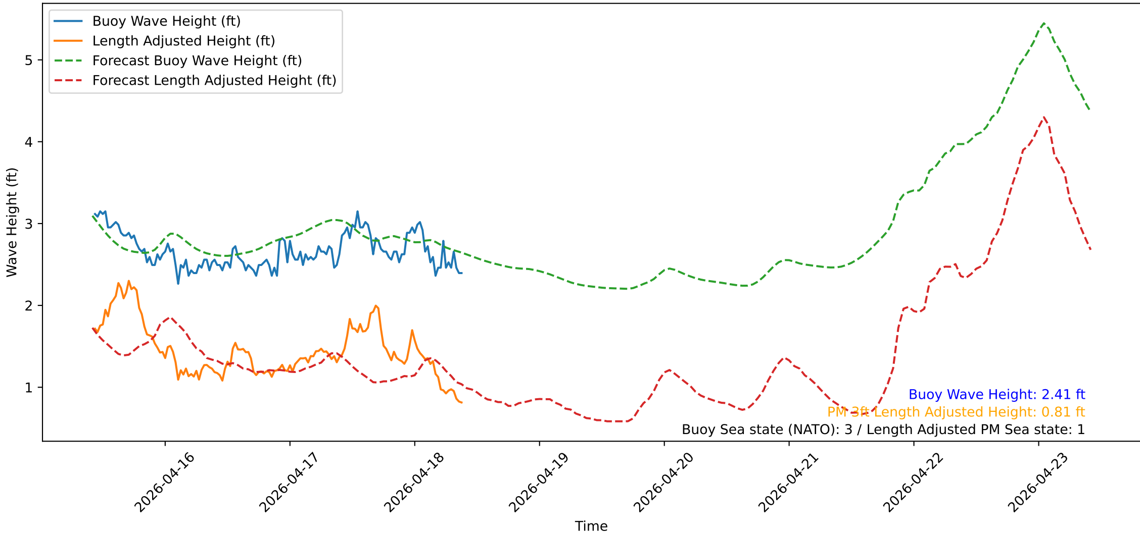
Wave Heights over Time for Red Beach at 2026-04-18 10:10:50
