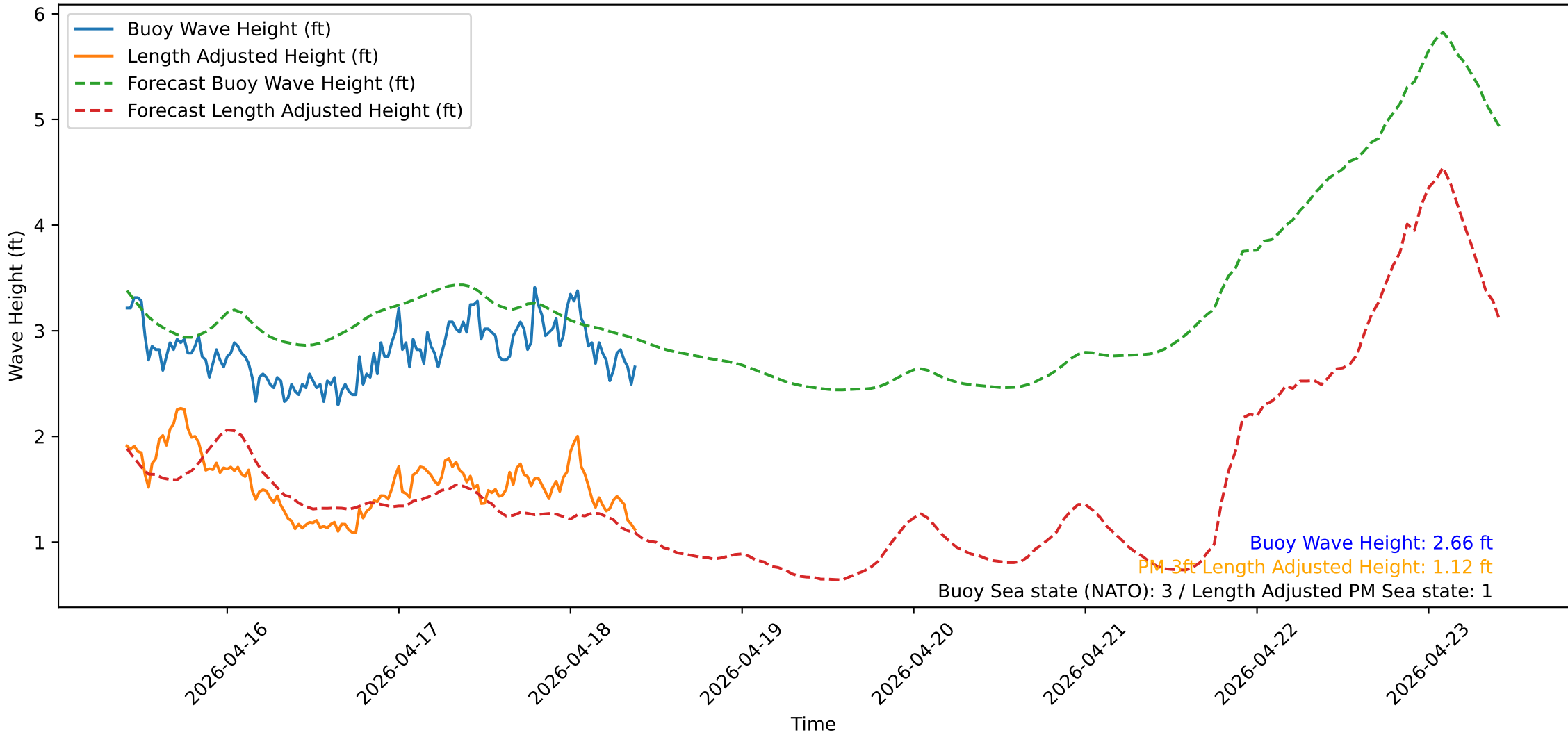
Wave Heights over Time for Oceanside Harbor at 2026-04-18 10:10:31
