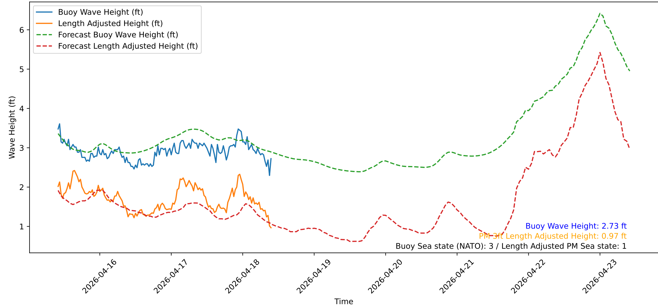
Wave Heights over Time for Green Beach at 2026-04-18 10:11:12
