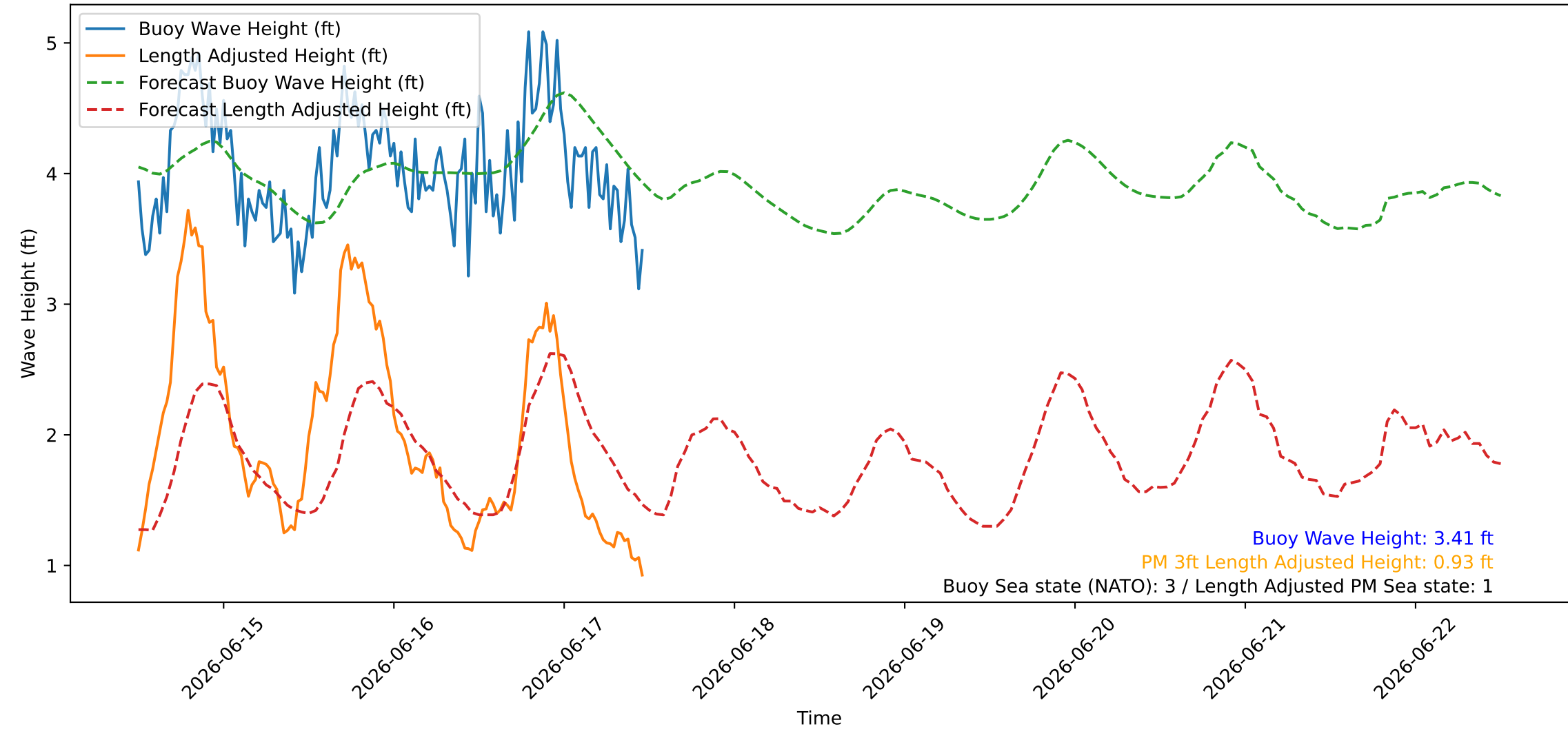
Wave Heights over Time for Green Beach at 2026-06-17 11:51:10
