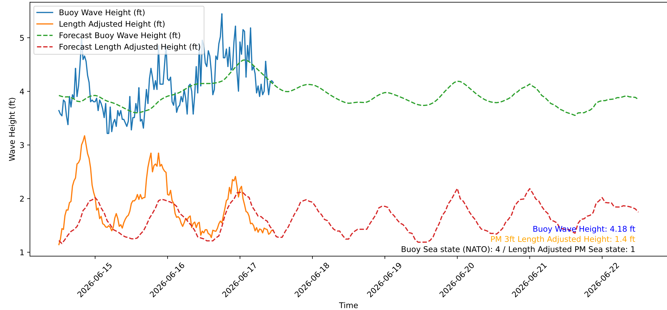
Wave Heights over Time for Oceanside Harbor at 2026-06-17 11:50:27
