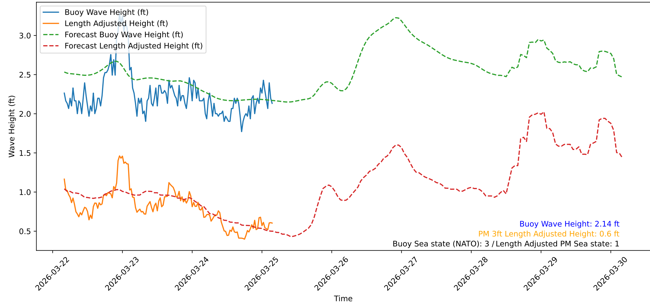
Wave Heights over Time for Green Beach at 2026-03-25 04:11:09
