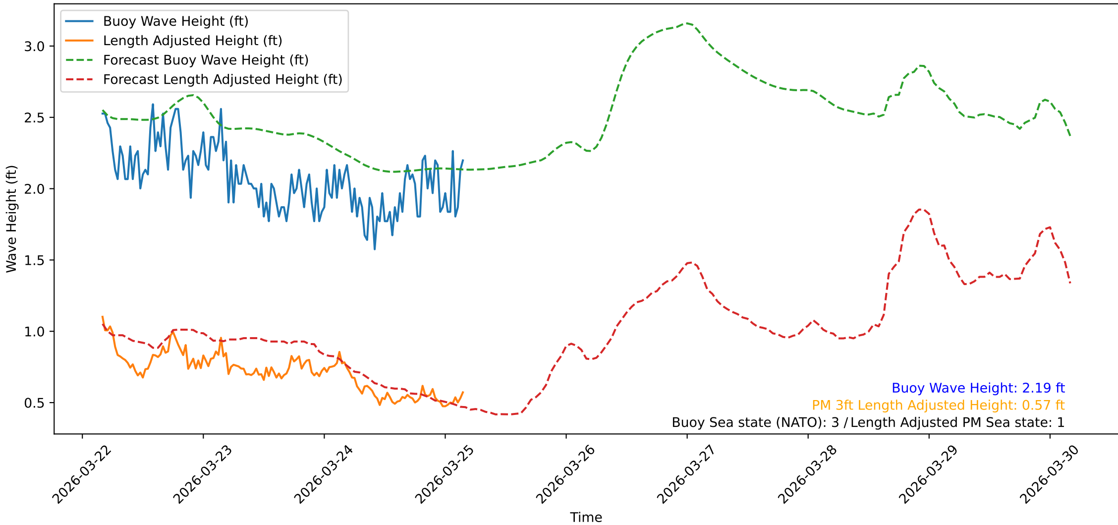
Wave Heights over Time for Oceanside Harbor at 2026-03-25 04:10:31
