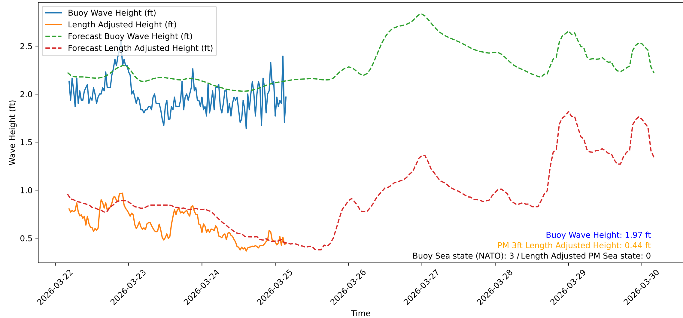
Wave Heights over Time for Red Beach at 2026-03-25 04:10:47
