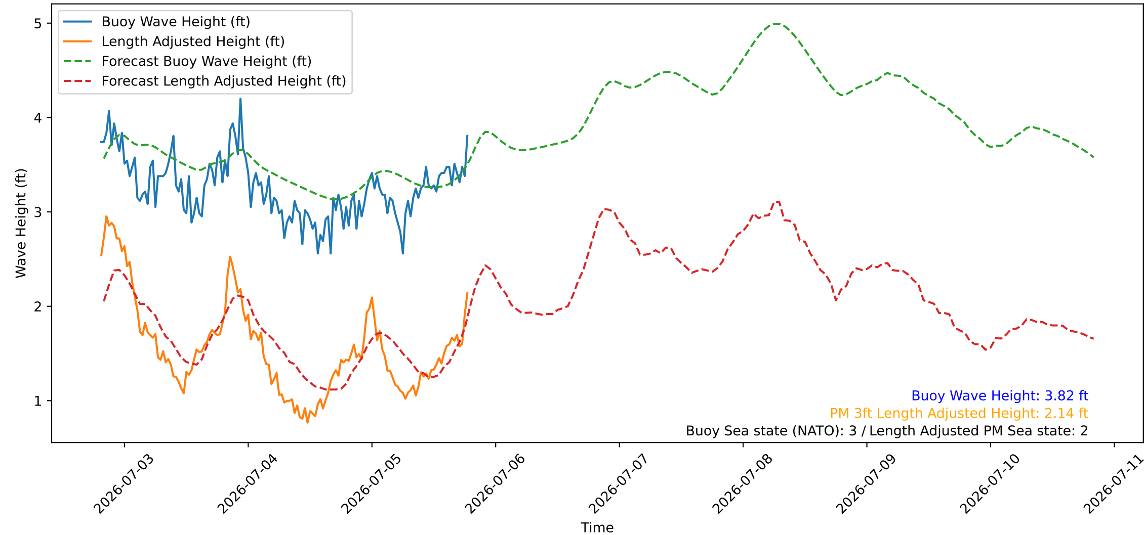
Wave Heights over Time for Green Beach at 2026-07-05 19:31:08
