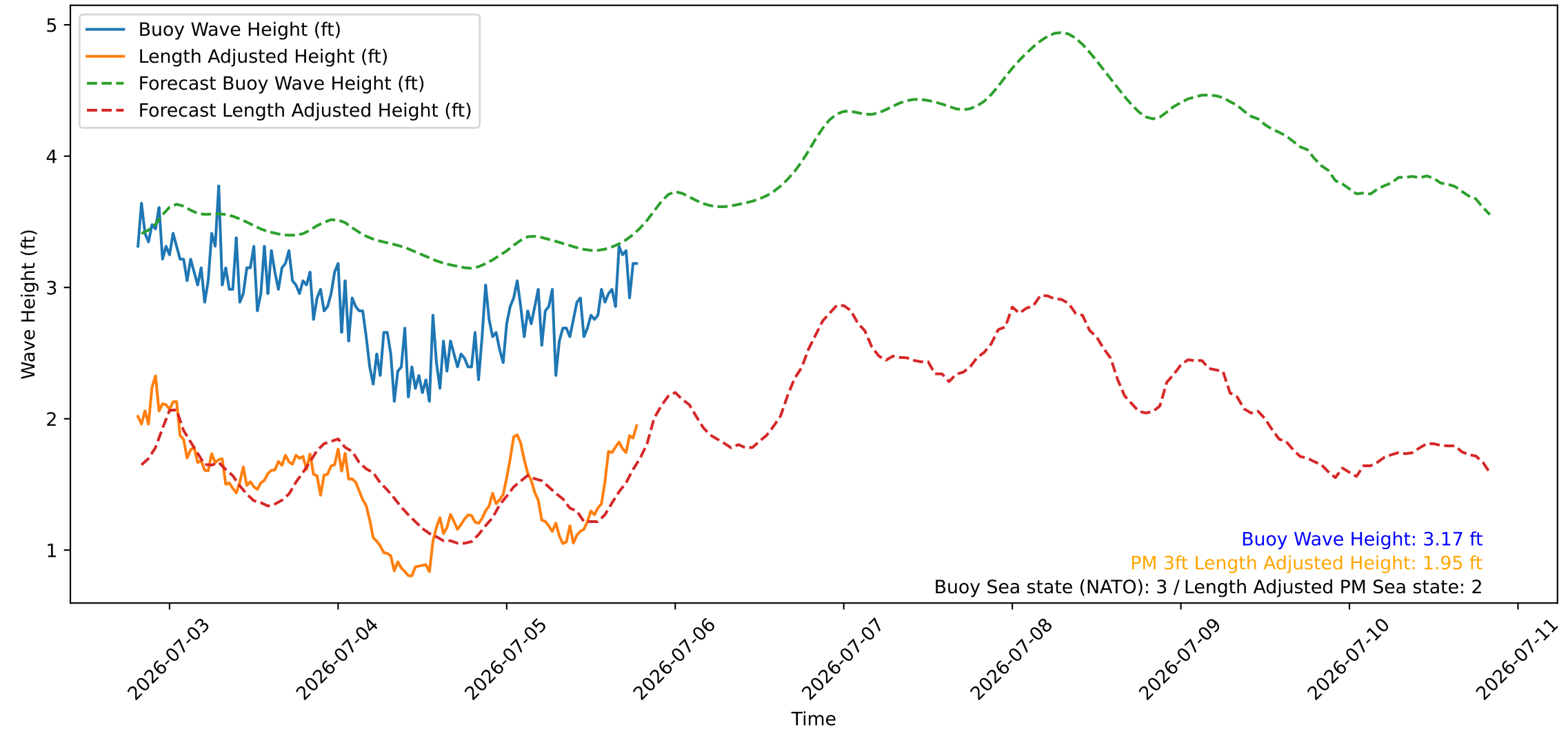
Wave Heights over Time for Oceanside Harbor at 2026-07-05 19:30:27
