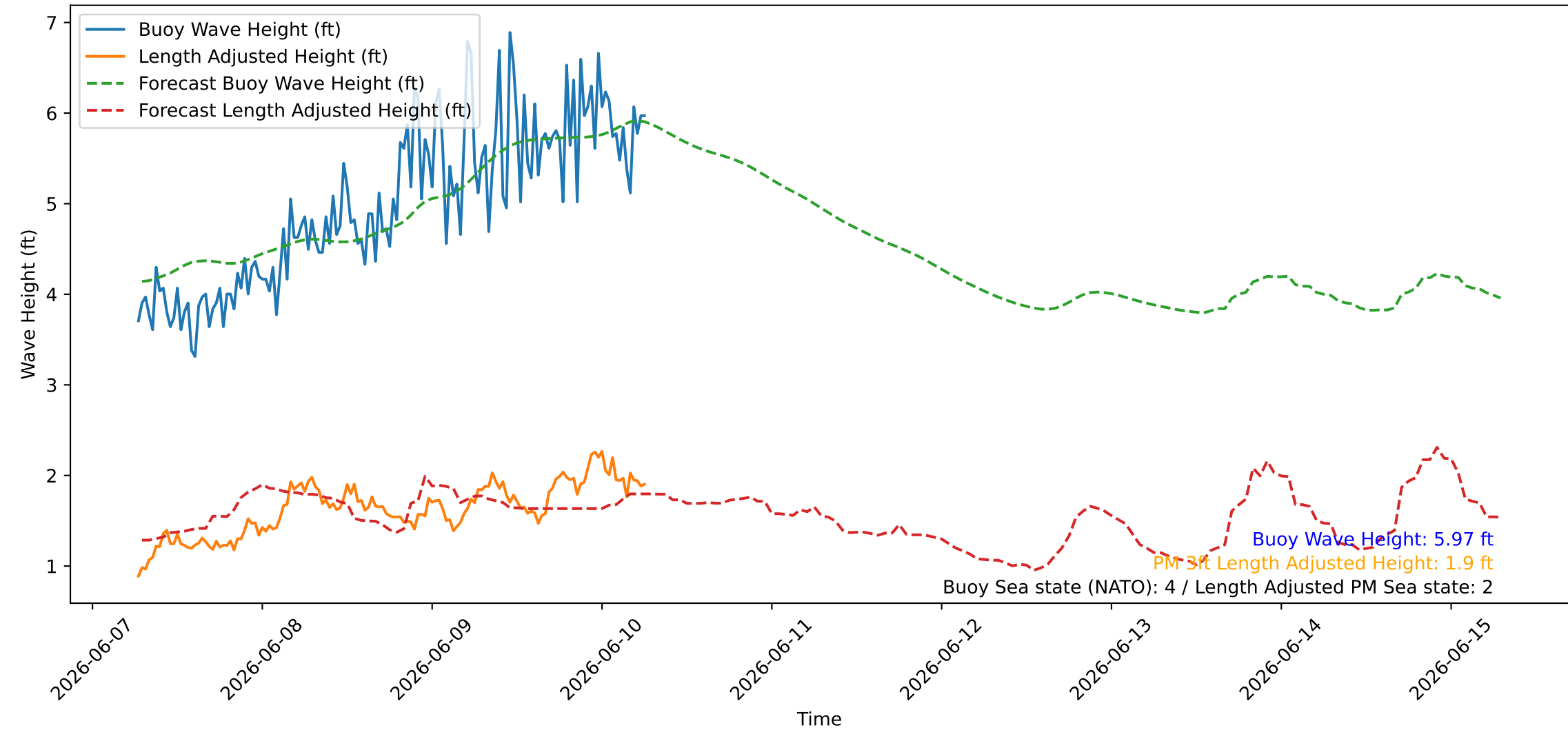
Wave Heights over Time for Green Beach at 2026-06-10 06:41:10
