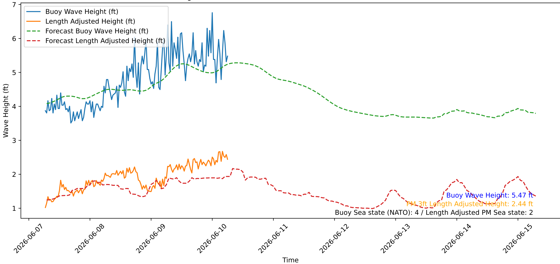
Wave Heights over Time for Oceanside Harbor at 2026-06-10 06:40:26
