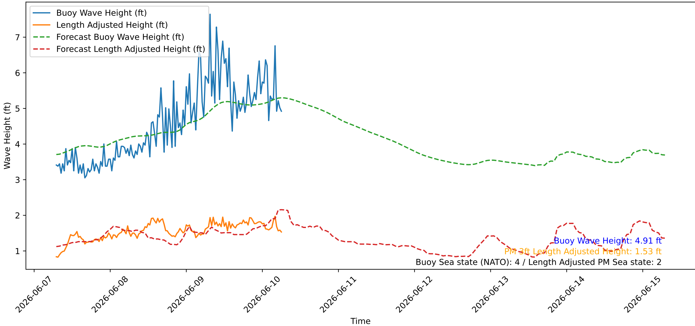
Wave Heights over Time for Red Beach at 2026-06-10 06:40:46
