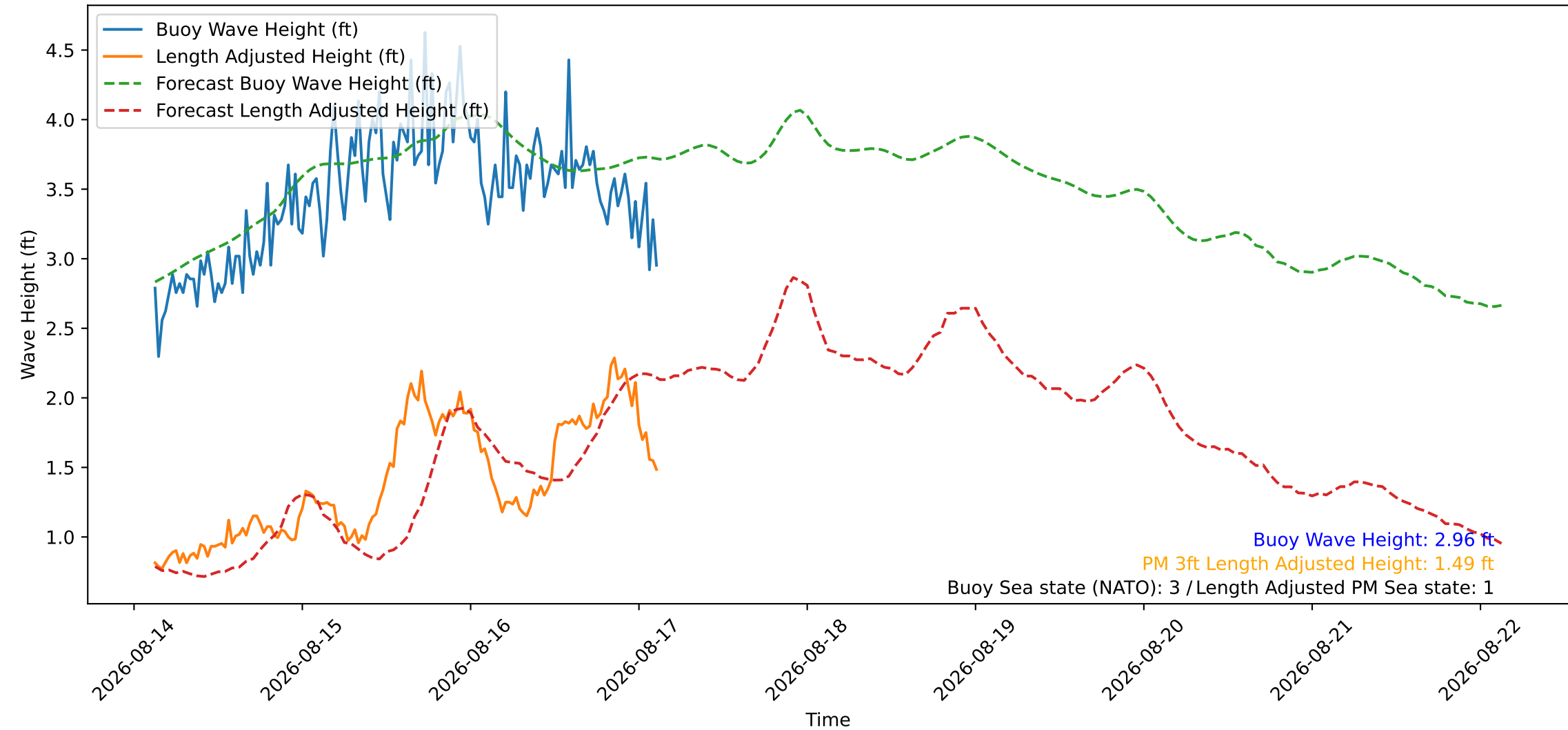
Wave Heights over Time for Oceanside Harbor at 2026-08-17 03:10:26
