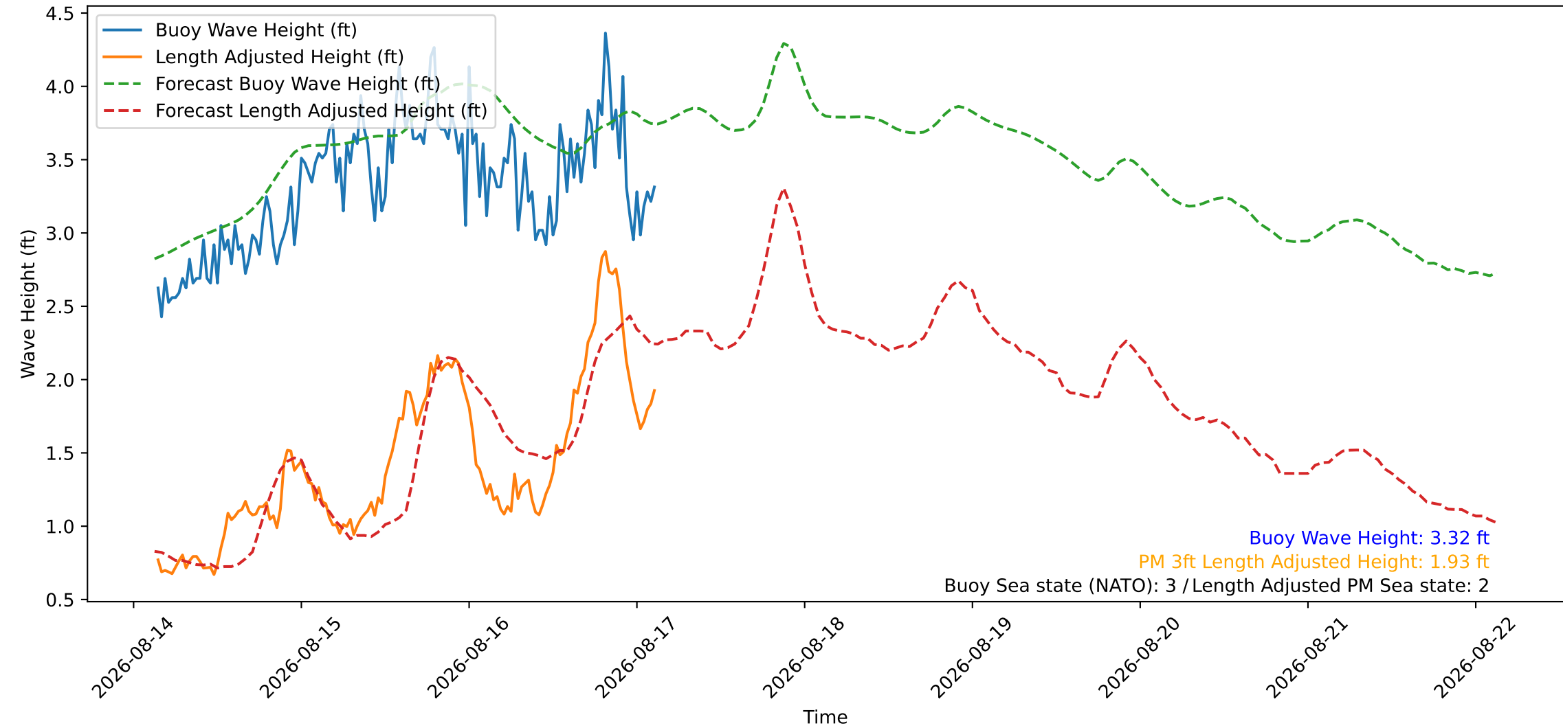
Wave Heights over Time for Green Beach at 2026-08-17 03:11:09
