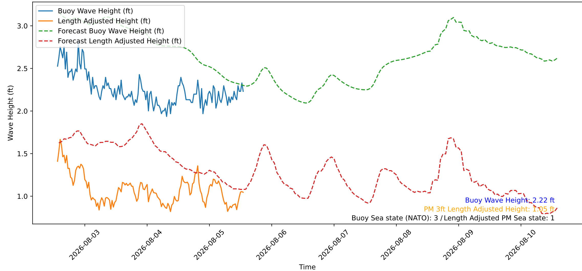
Wave Heights over Time for Green Beach at 2026-08-05 13:41:08
