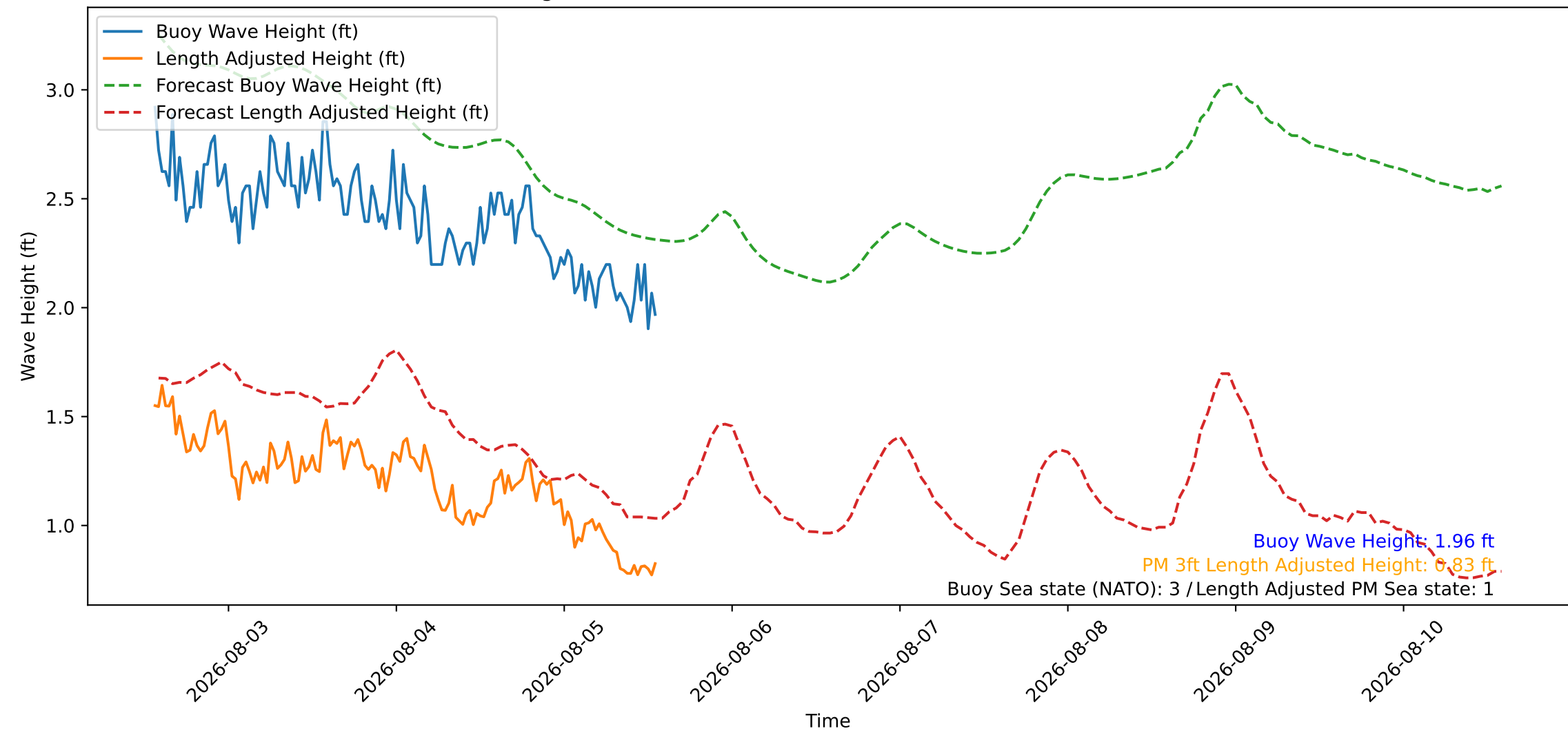
Wave Heights over Time for Oceanside Harbor at 2026-08-05 13:40:26
