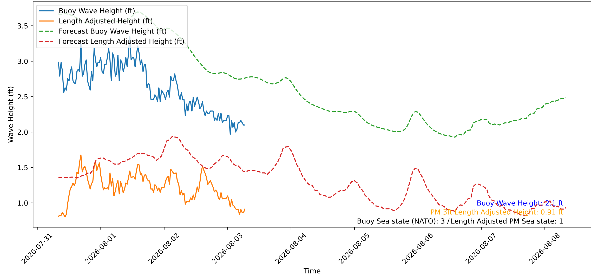
Wave Heights over Time for Red Beach at 2026-08-03 07:30:46
