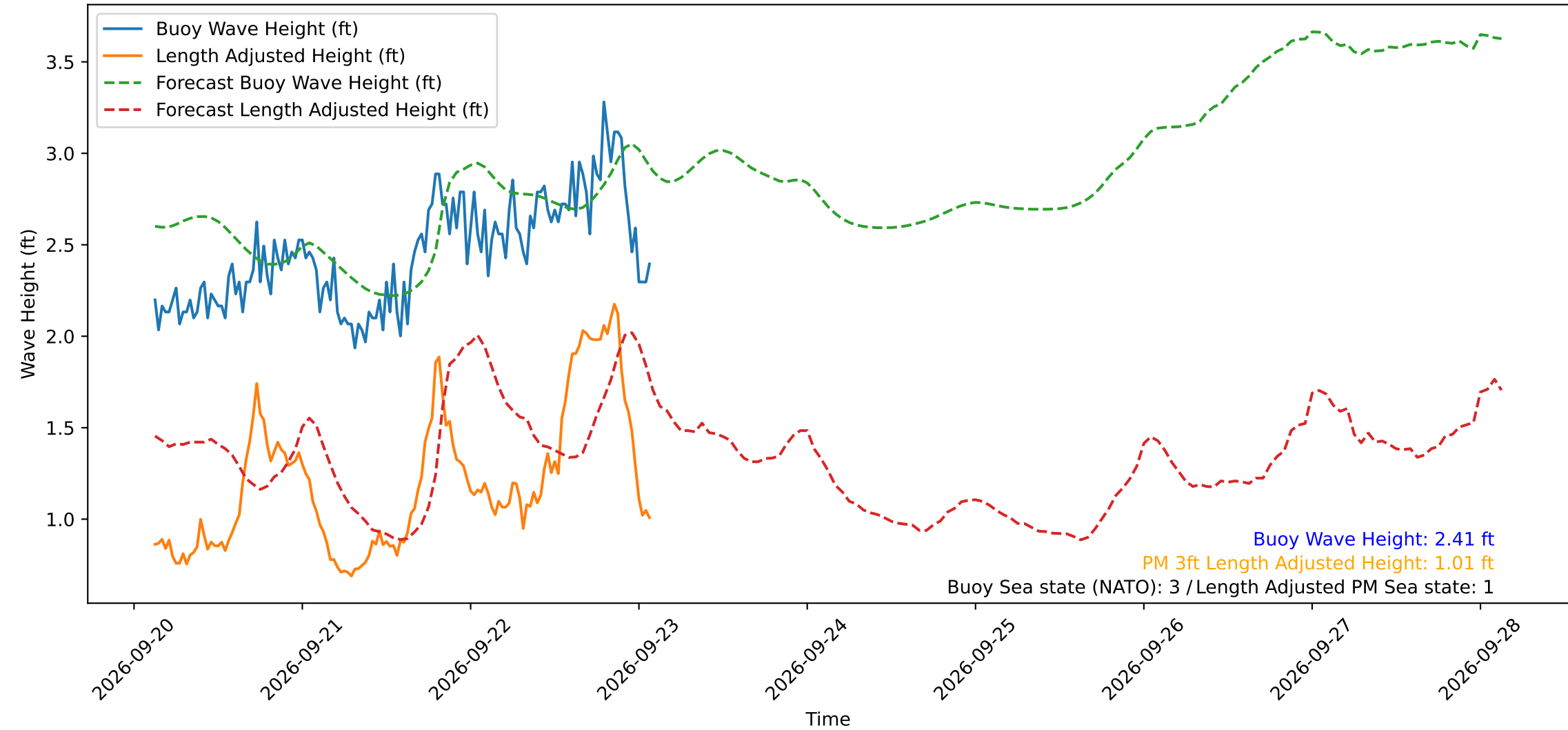
Wave Heights over Time for Red Beach at 2026-09-23 02:30:50
