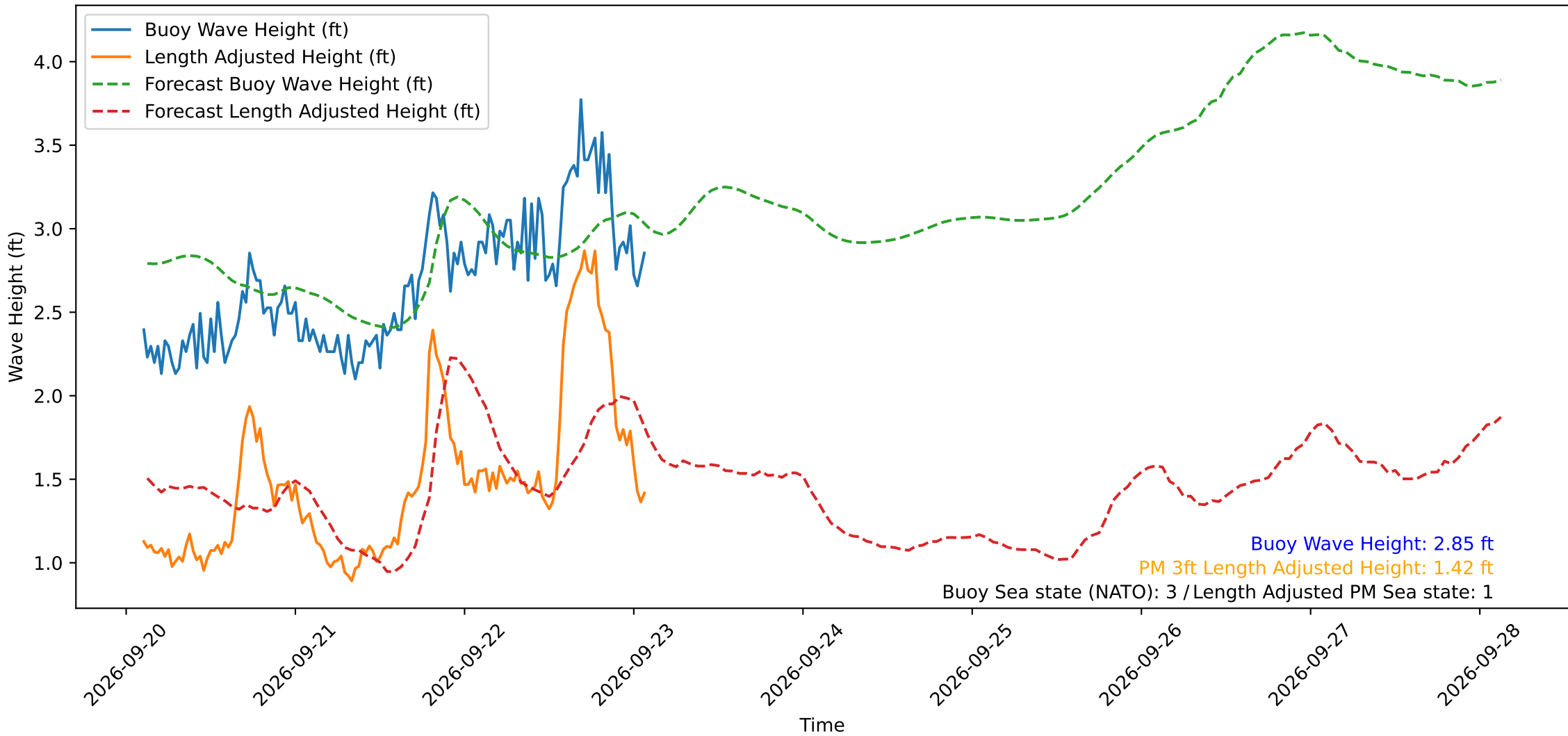
Wave Heights over Time for Oceanside Harbor at 2026-09-23 02:30:30
