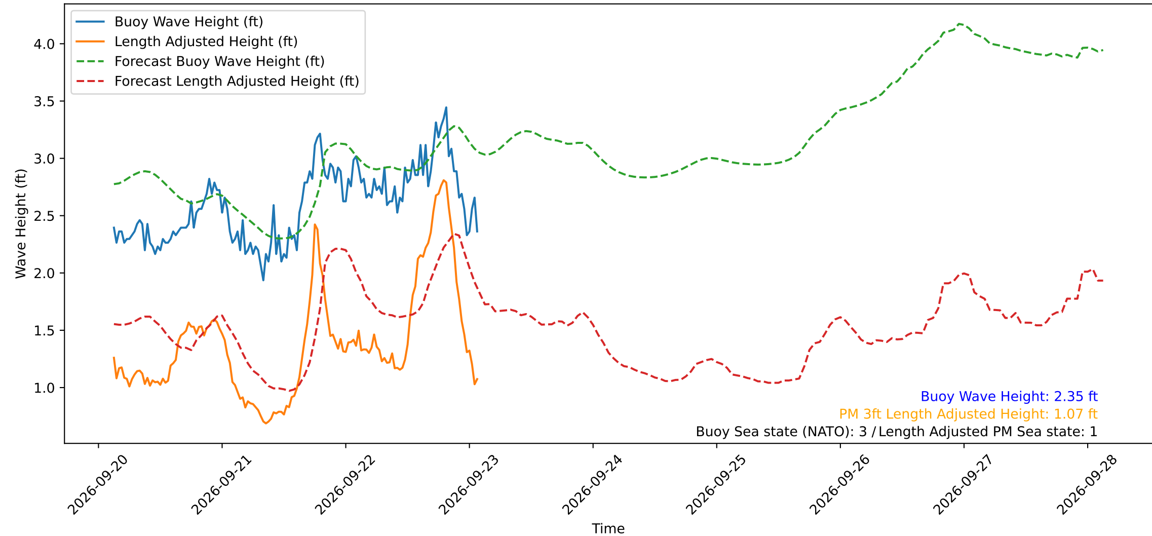
Wave Heights over Time for Green Beach at 2026-09-23 02:31:13
