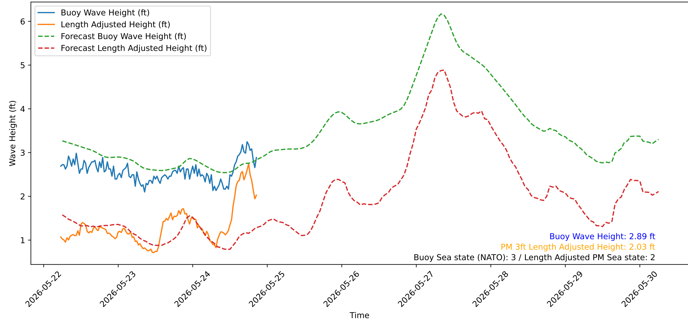
Wave Heights over Time for Oceanside Harbor at 2026-05-25 05:30:30
