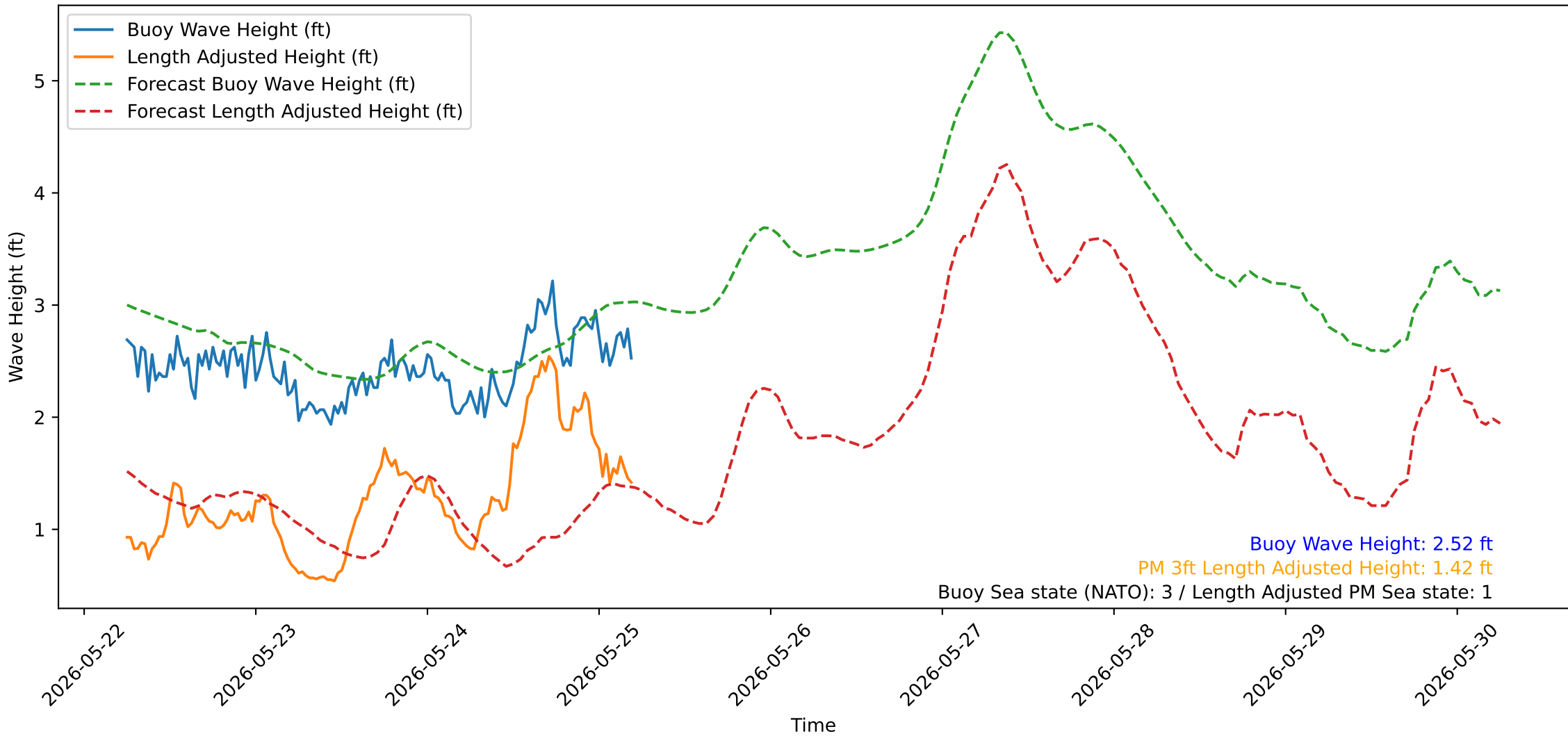
Wave Heights over Time for Red Beach at 2026-05-25 05:30:50
