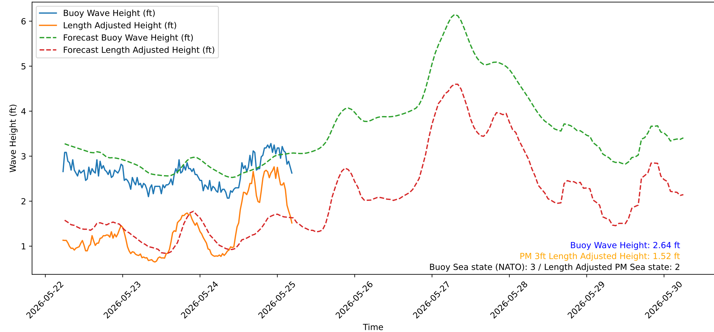
Wave Heights over Time for Green Beach at 2026-05-25 05:31:12
