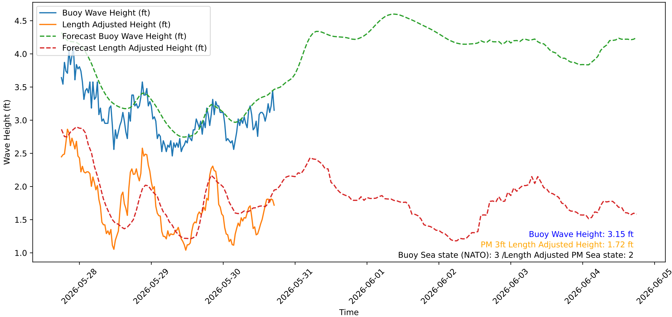
Wave Heights over Time for Green Beach at 2026-05-30 18:01:06
