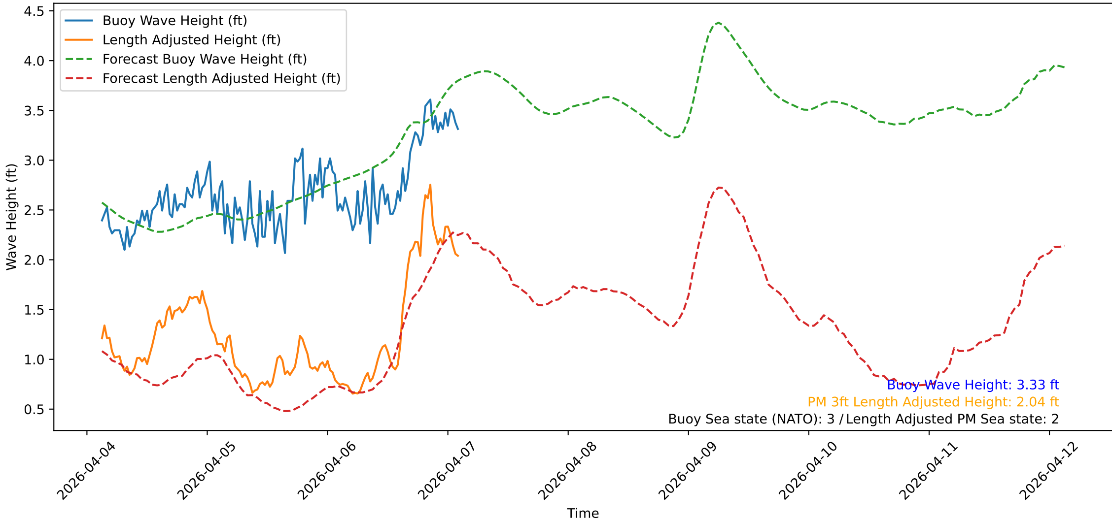
Wave Heights over Time for Oceanside Harbor at 2026-04-07 03:10:31
