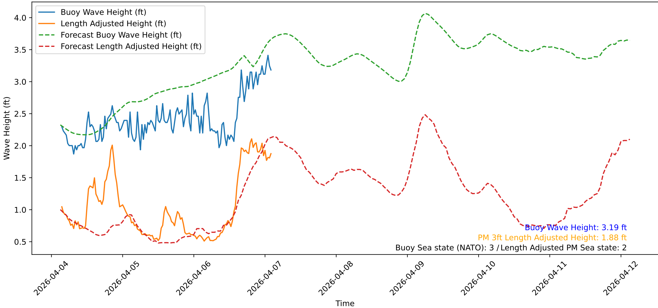
Wave Heights over Time for Red Beach at 2026-04-07 03:10:47
