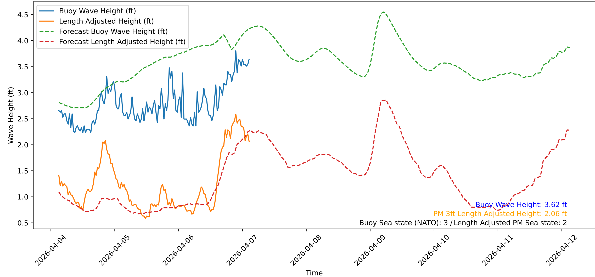
Wave Heights over Time for Green Beach at 2026-04-07 03:11:09
