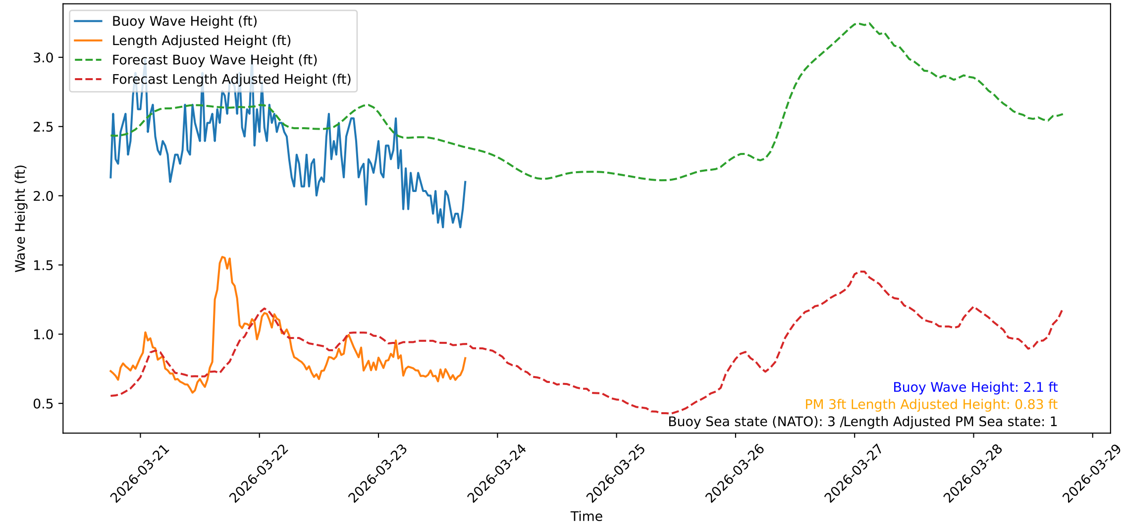
Wave Heights over Time for Oceanside Harbor at 2026-03-23 18:10:31
