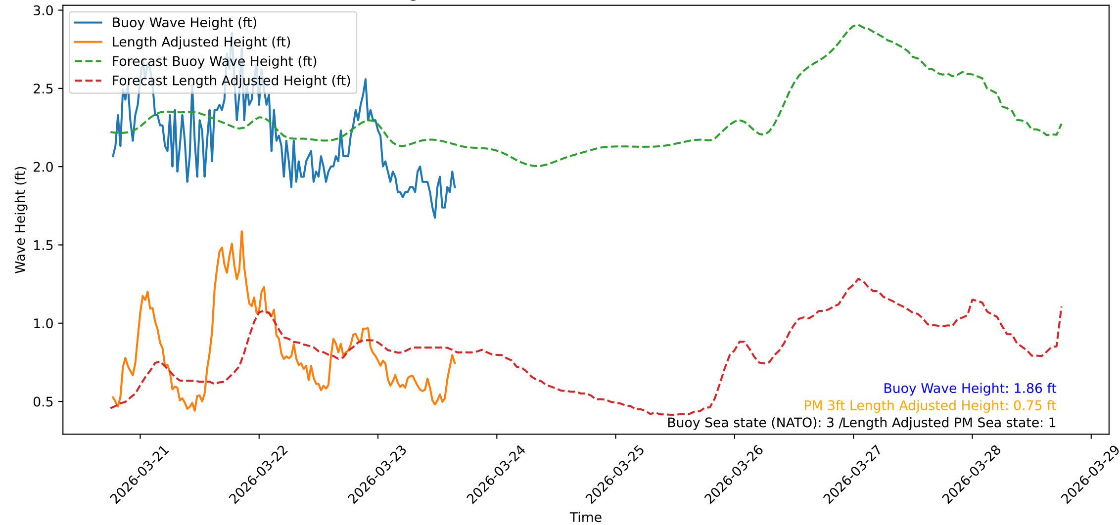
Wave Heights over Time for Red Beach at 2026-03-23 18:10:47
