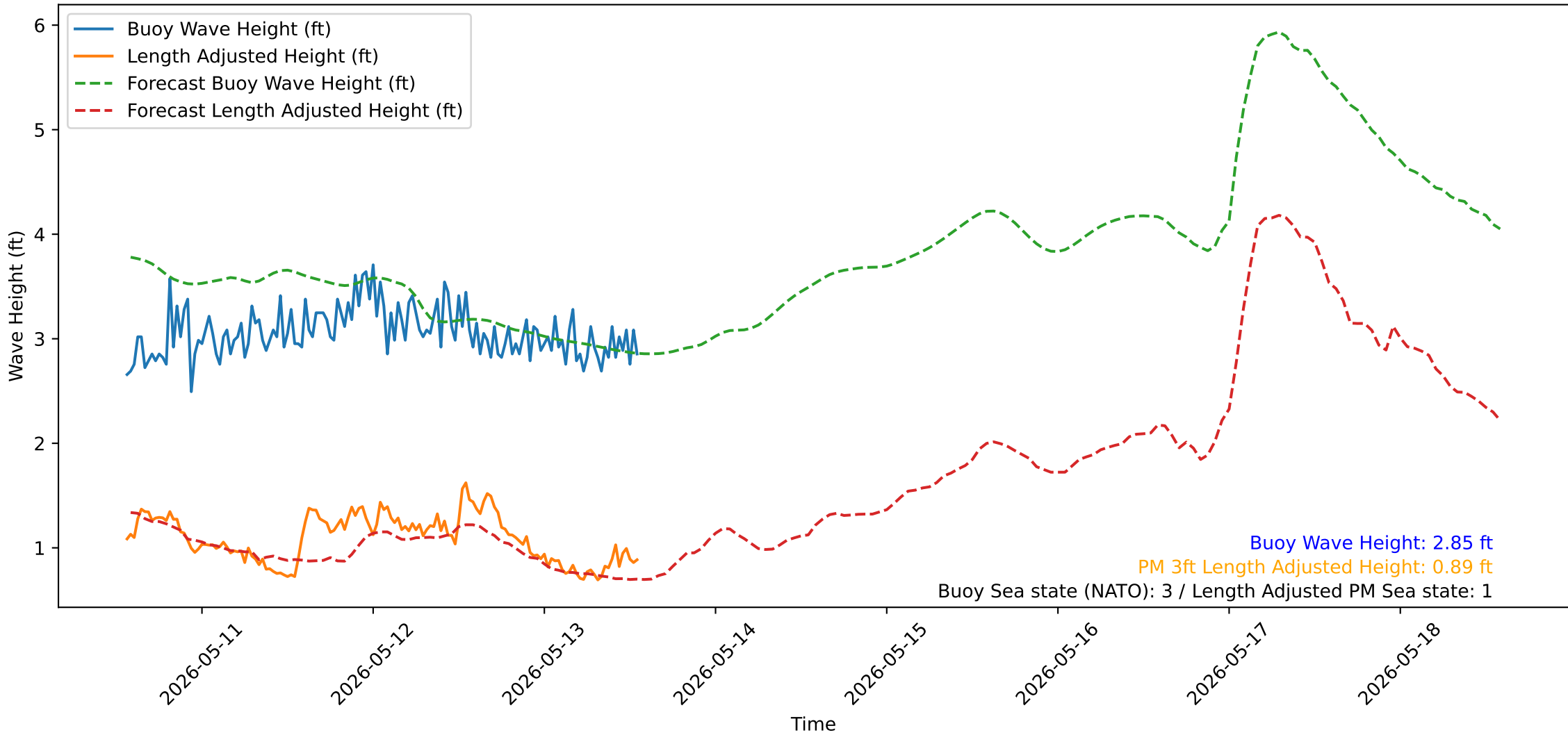
Wave Heights over Time for Oceanside Harbor at 2026-05-13 13:30:31
