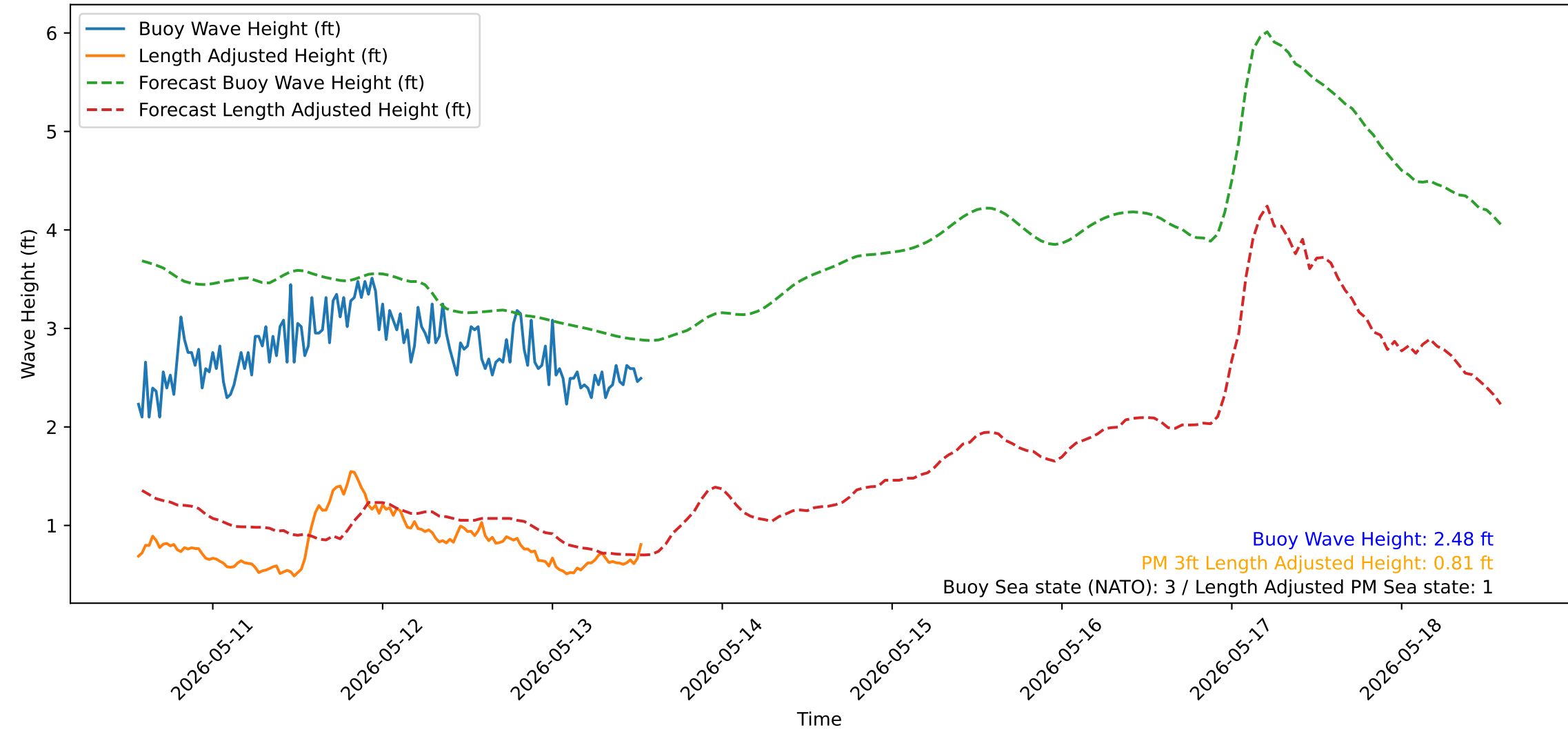
Wave Heights over Time for Green Beach at 2026-05-13 13:31:13
