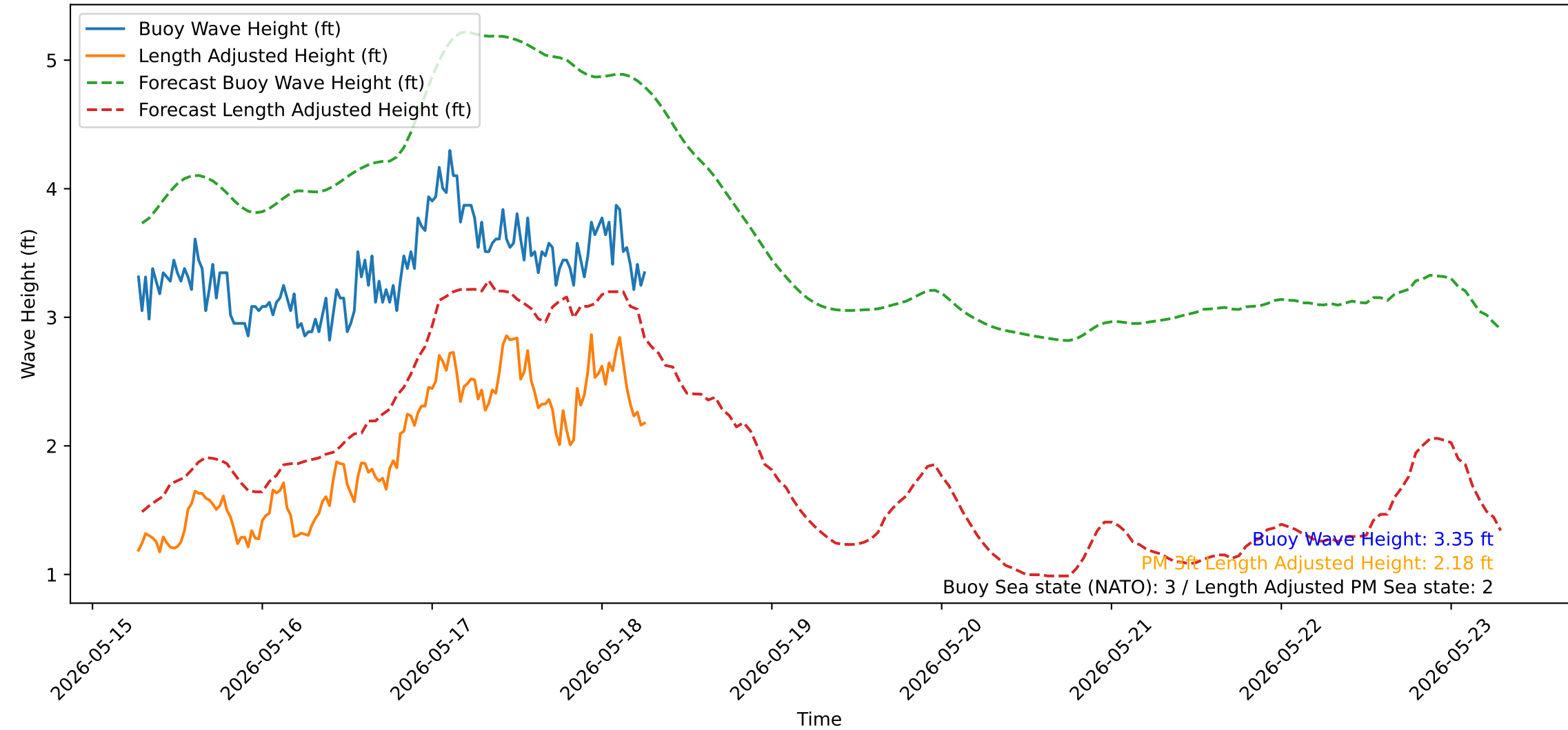
Wave Heights over Time for Oceanside Harbor at 2026-05-18 06:40:32
