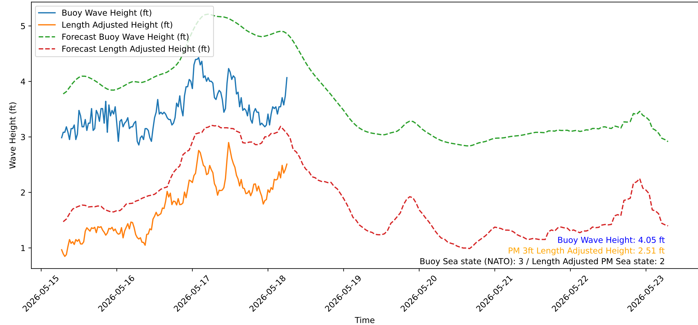
Wave Heights over Time for Green Beach at 2026-05-18 06:41:14
