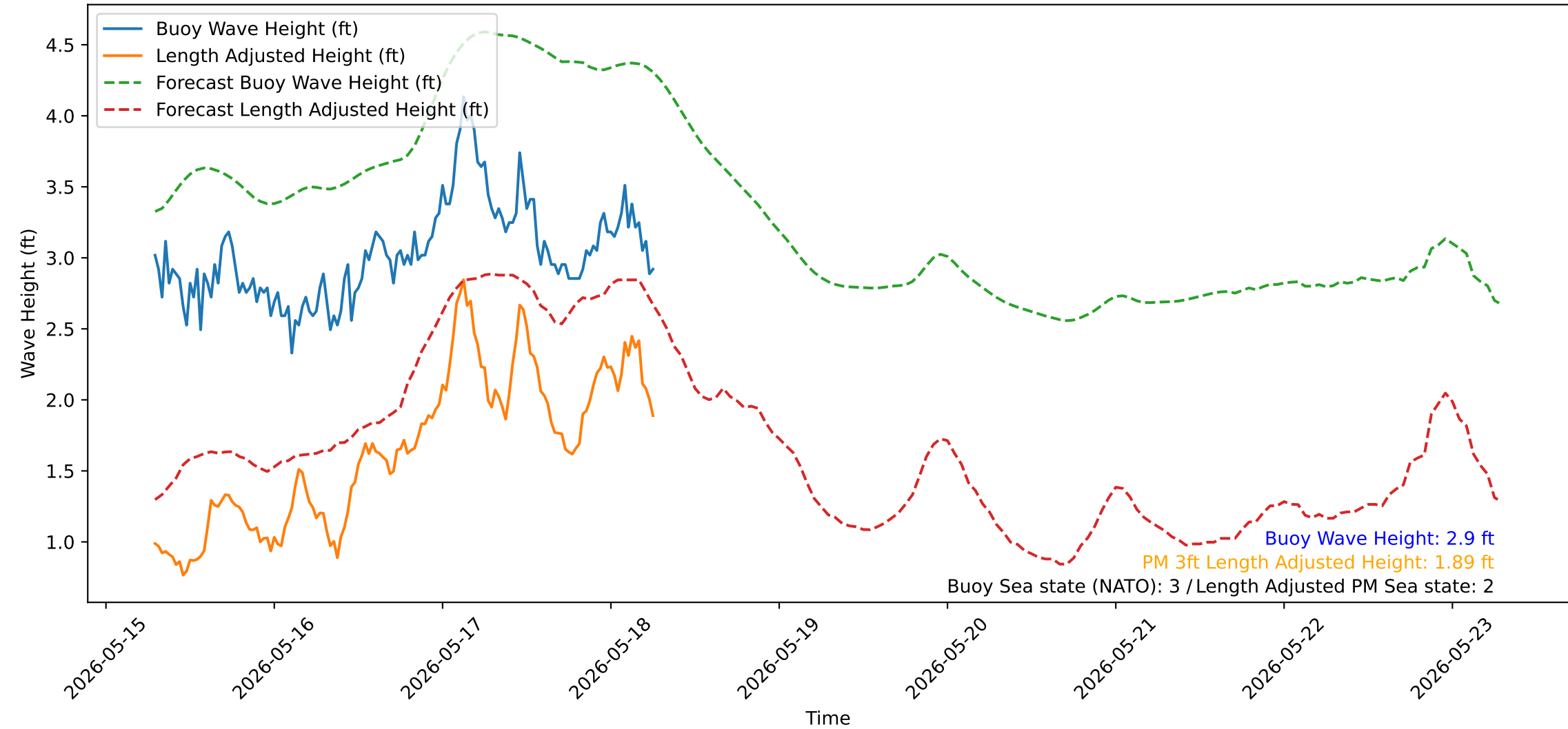
Wave Heights over Time for Red Beach at 2026-05-18 06:40:51
