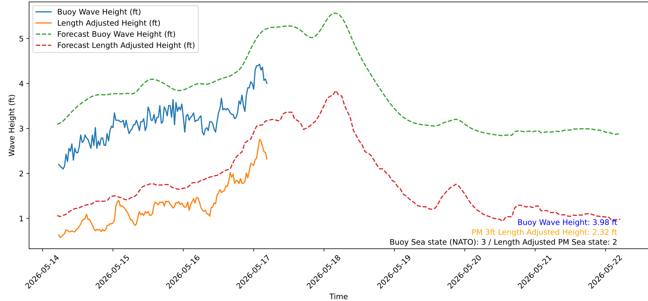
Wave Heights over Time for Green Beach at 2026-05-17 05:21:15
